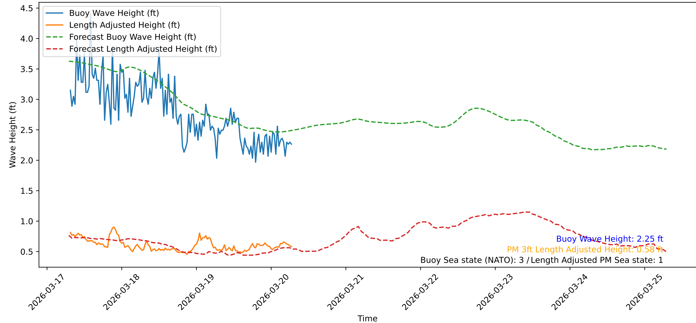
Wave Heights over Time for Oceanside Harbor at 2026-03-20 07:20:31
