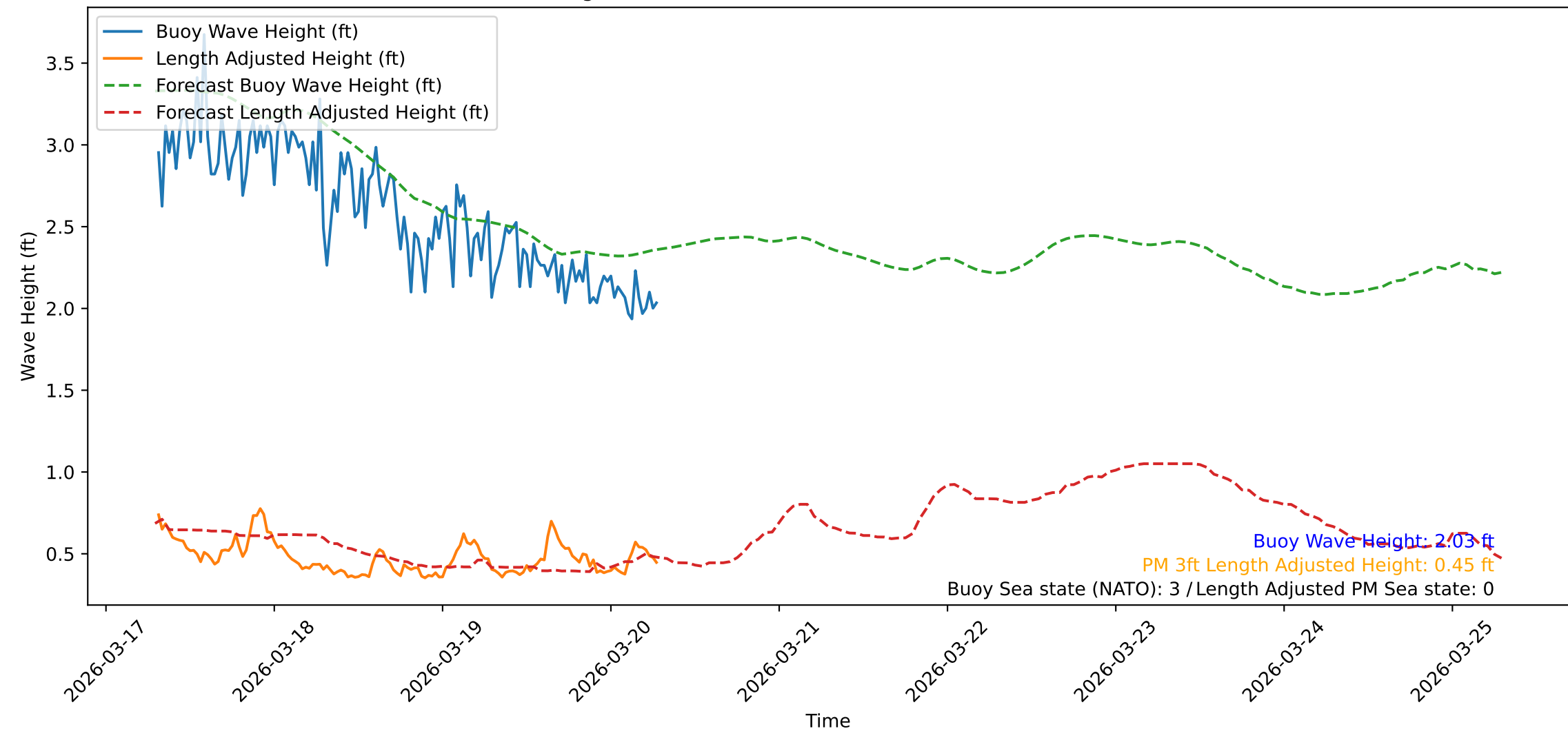
Wave Heights over Time for Red Beach at 2026-03-20 07:20:47
