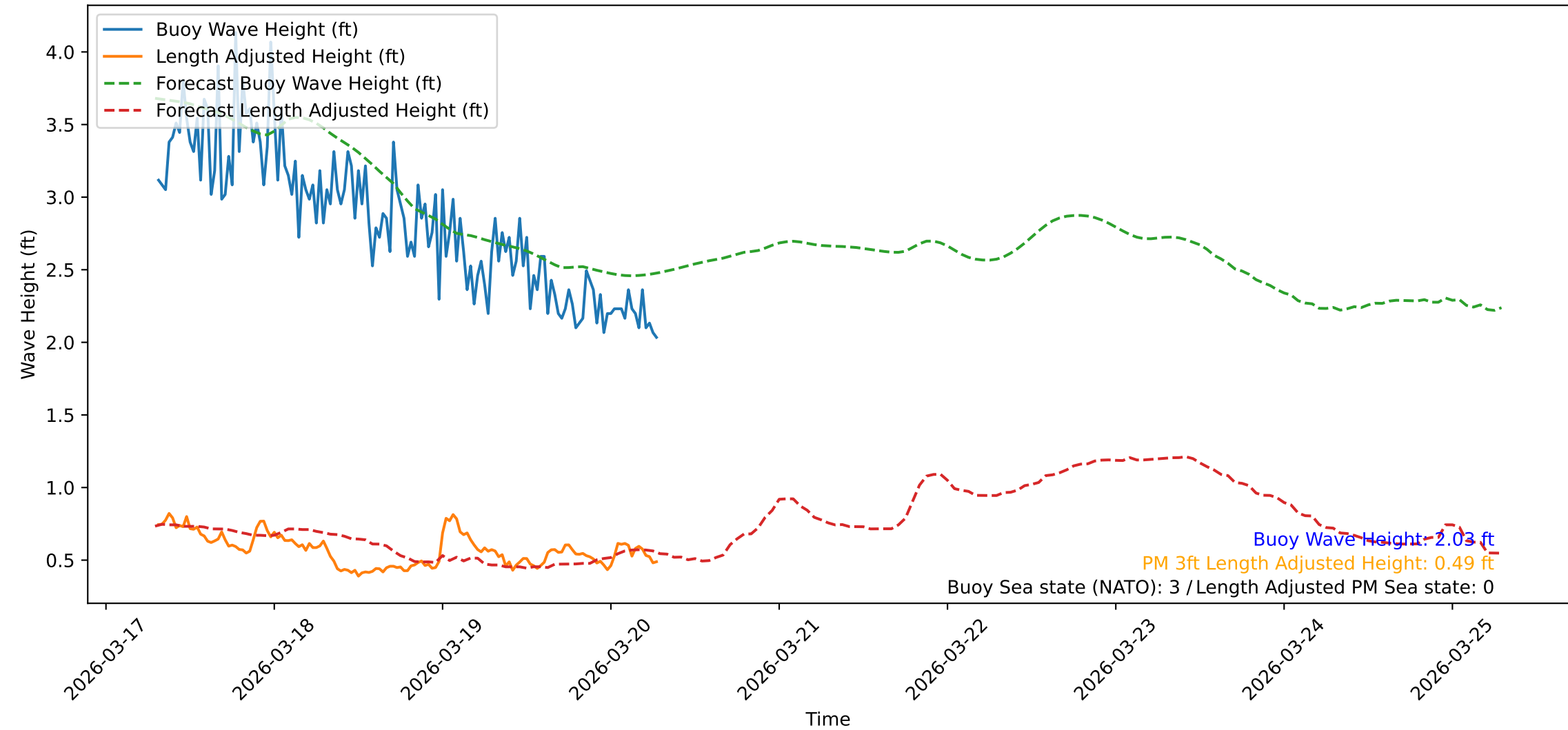
Wave Heights over Time for Green Beach at 2026-03-20 07:21:09
