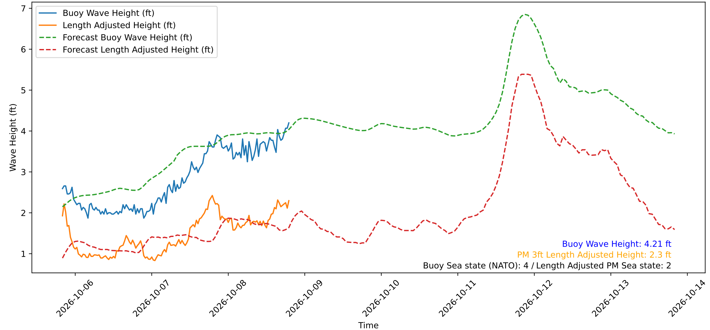
Wave Heights over Time for Red Beach at 2026-10-08 19:50:50
