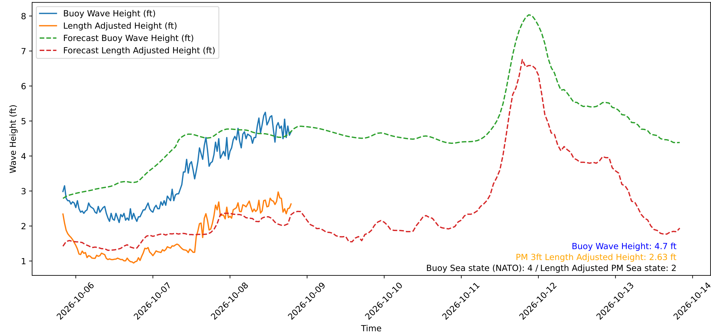
Wave Heights over Time for Green Beach at 2026-10-08 19:51:14
