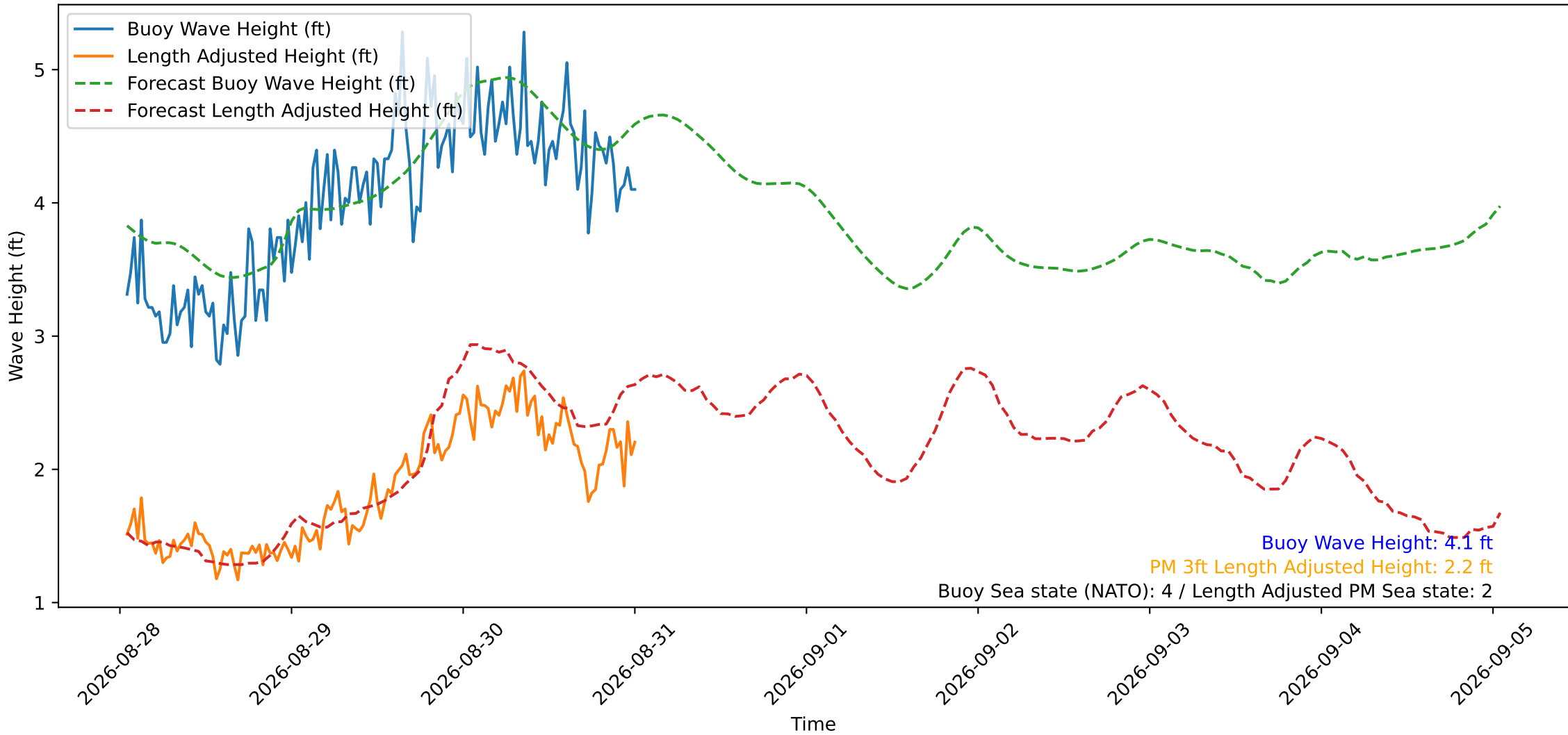
Wave Heights over Time for Oceanside Harbor at 2026-08-31 00:50:30
