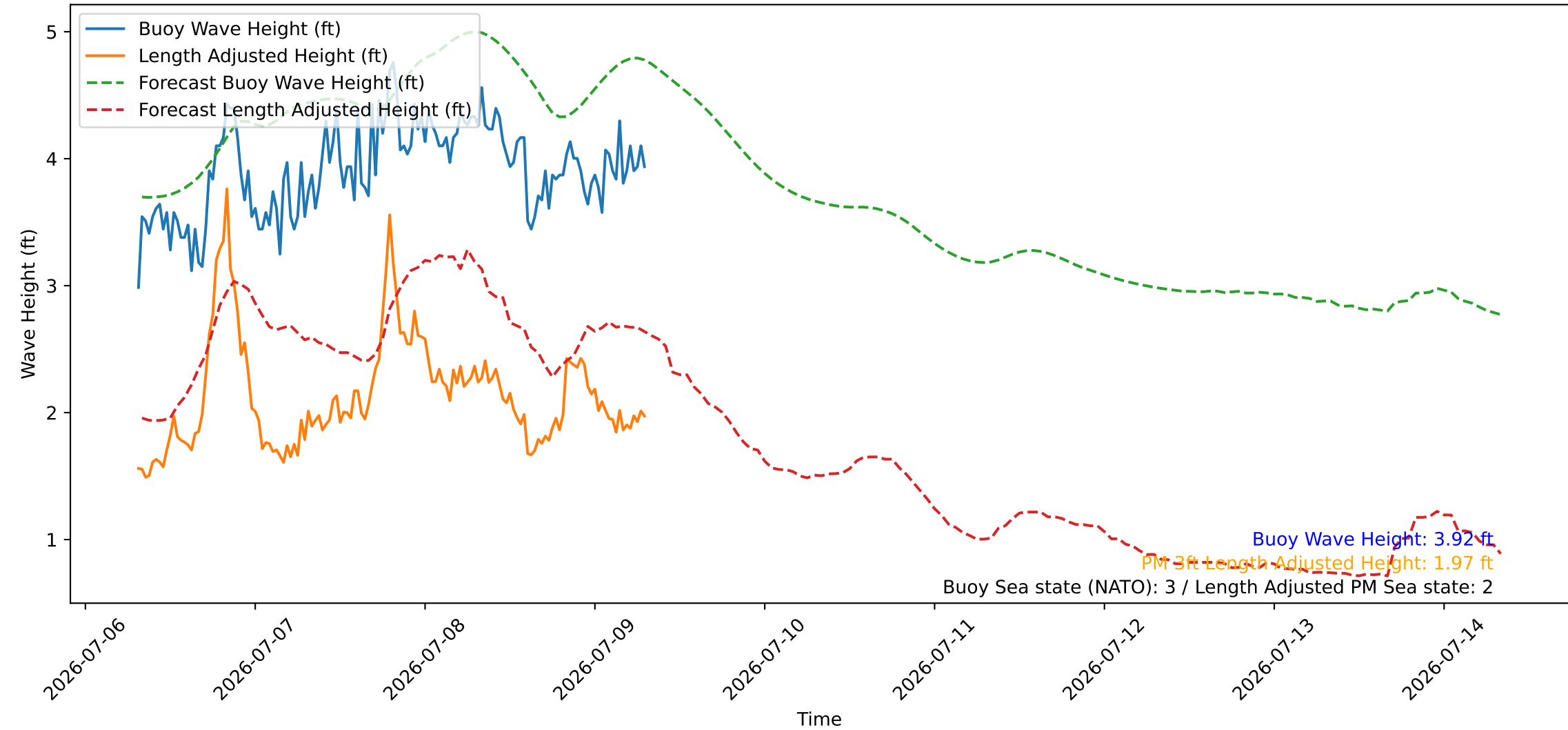
Wave Heights over Time for Green Beach at 2026-07-09 07:41:09
