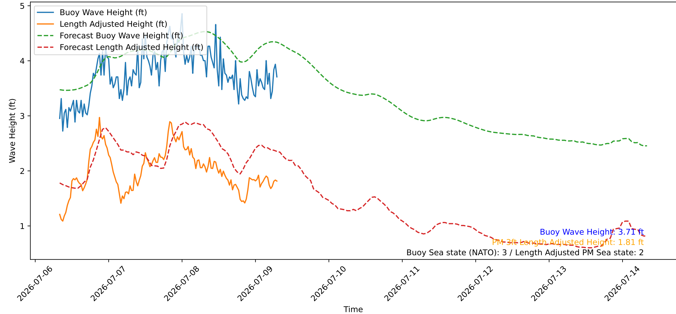
Wave Heights over Time for Red Beach at 2026-07-09 07:40:47
