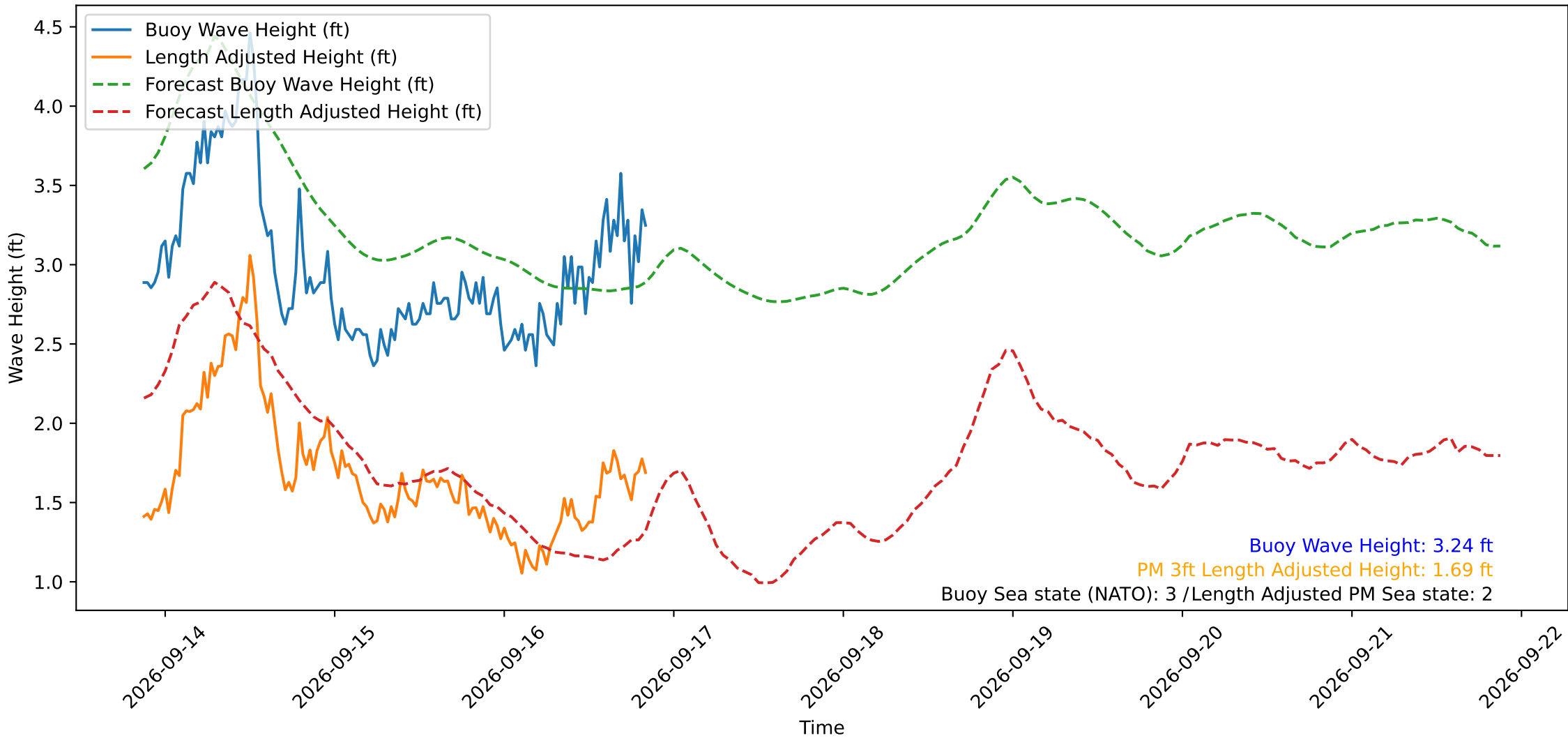
Wave Heights over Time for Oceanside Harbor at 2026-09-16 21:00:30
