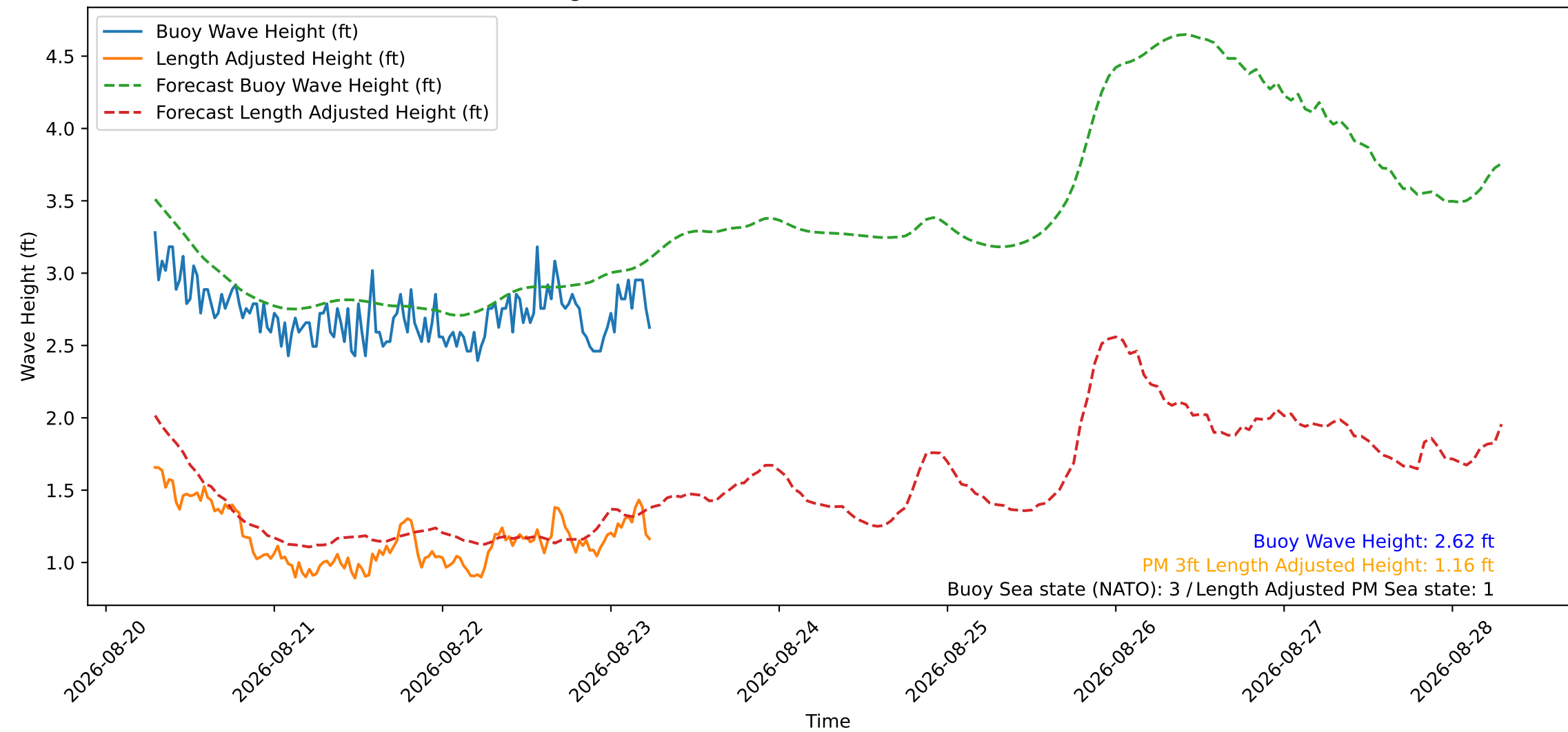
Wave Heights over Time for Green Beach at 2026-08-23 06:31:11
