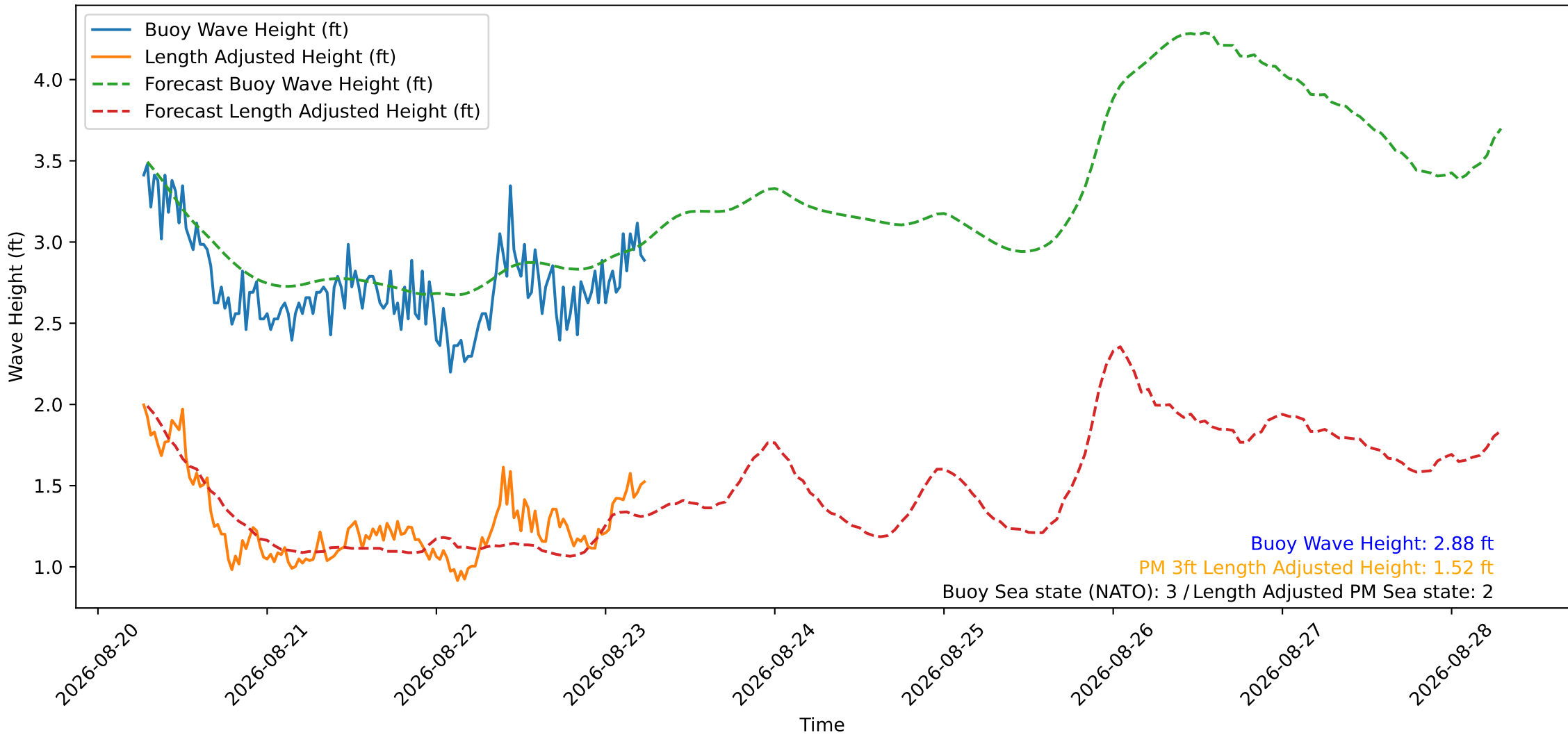
Wave Heights over Time for Oceanside Harbor at 2026-08-23 06:30:29
