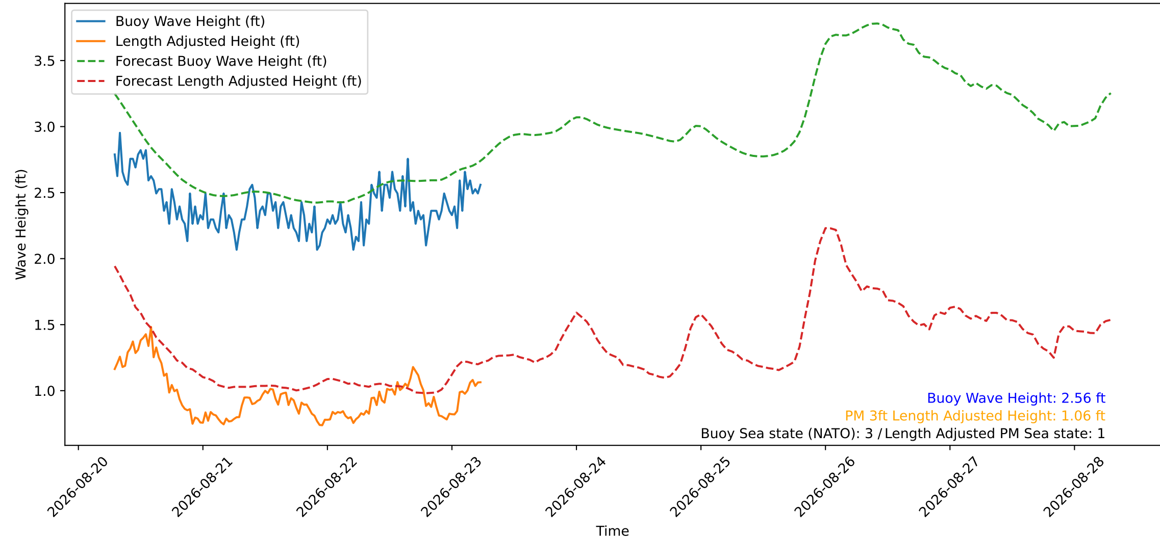
Wave Heights over Time for Red Beach at 2026-08-23 06:30:48
