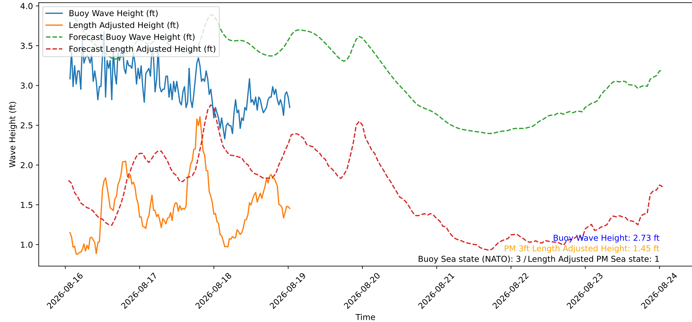
Wave Heights over Time for Red Beach at 2026-08-19 01:20:47
