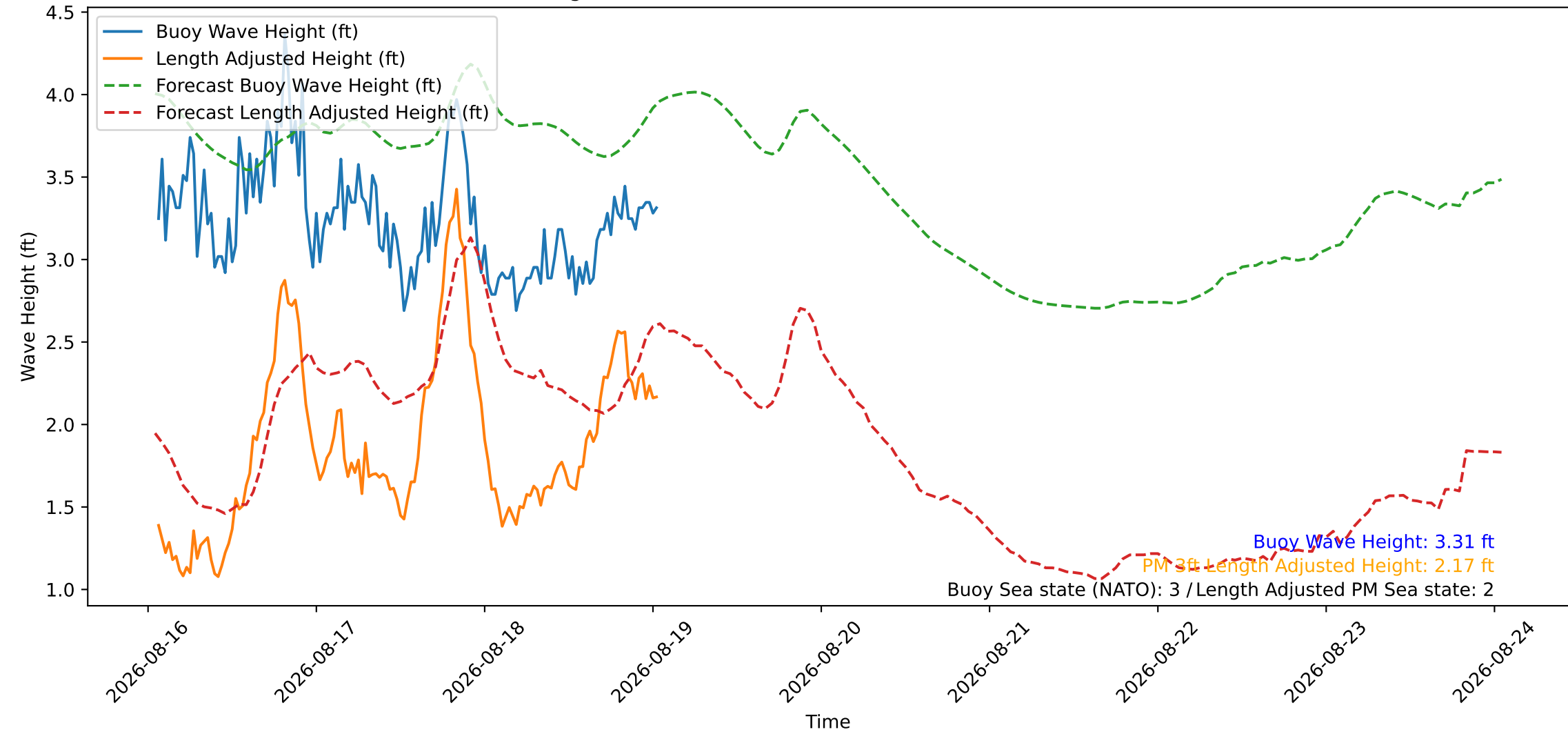
Wave Heights over Time for Green Beach at 2026-08-19 01:21:11
