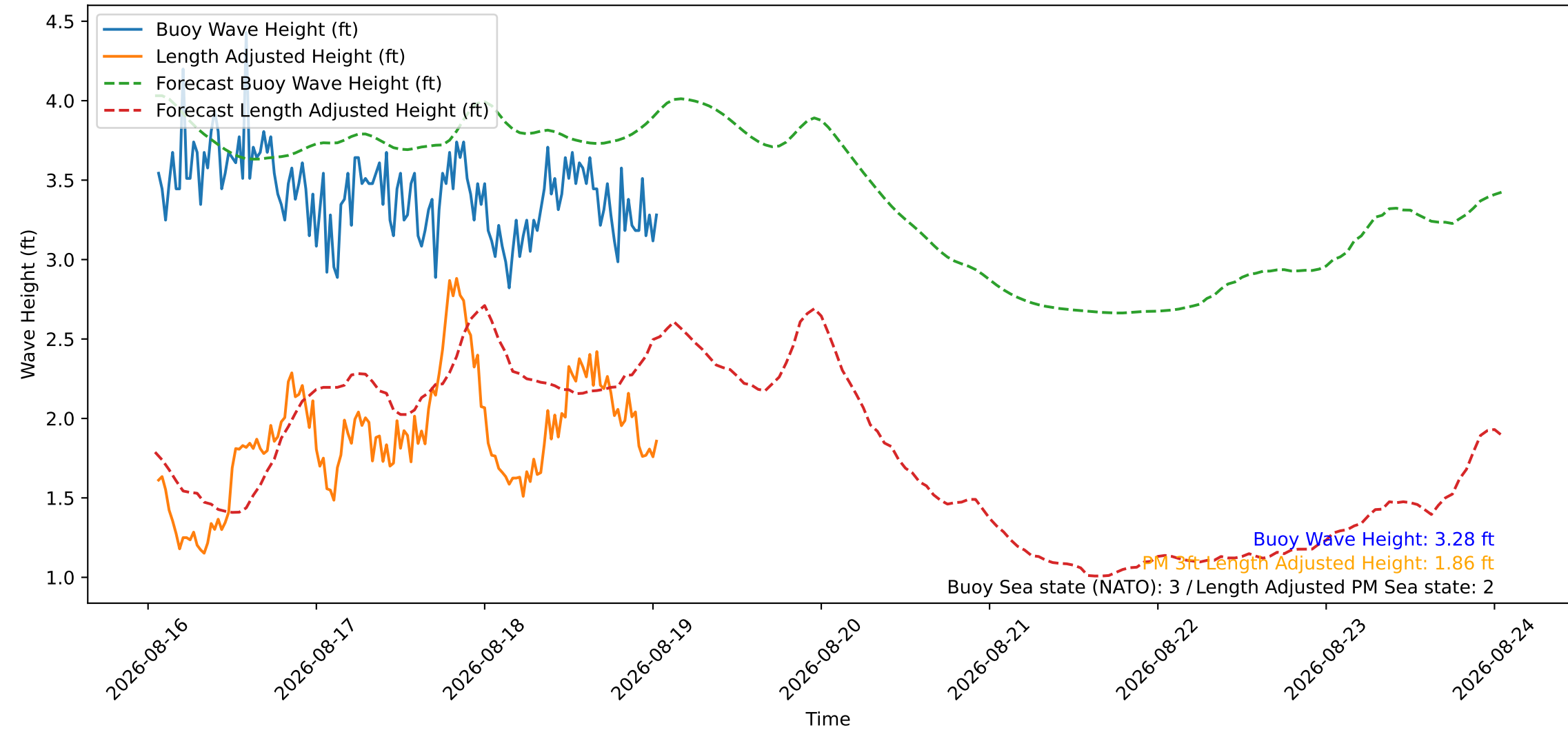
Wave Heights over Time for Oceanside Harbor at 2026-08-19 01:20:26
