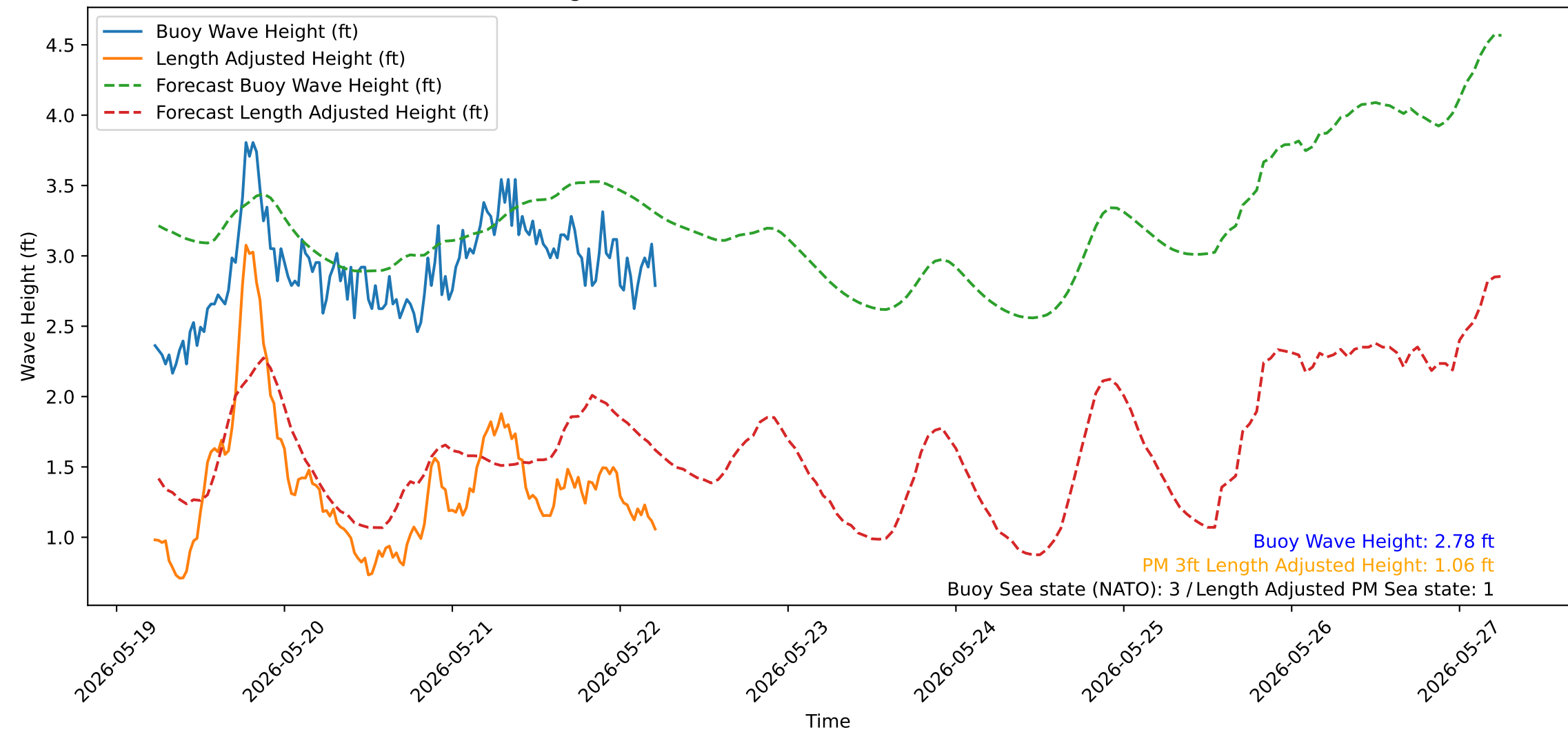
Wave Heights over Time for Green Beach at 2026-05-22 05:41:13
