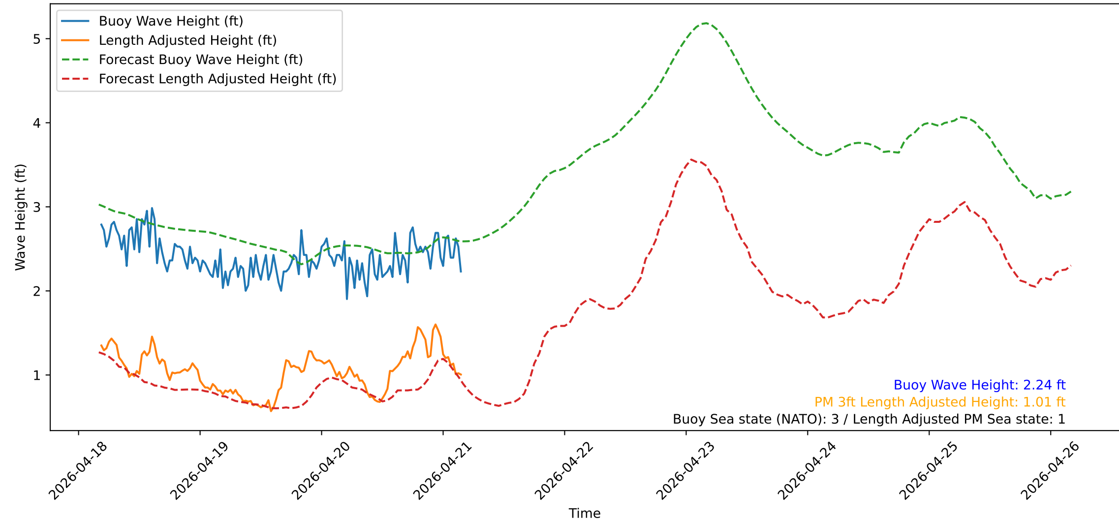
Wave Heights over Time for Oceanside Harbor at 2026-04-21 04:20:31
