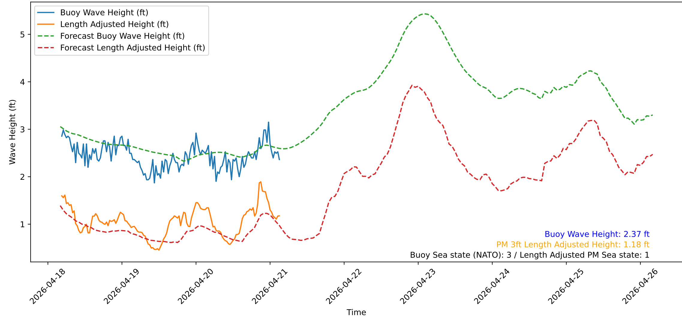
Wave Heights over Time for Green Beach at 2026-04-21 04:21:14
