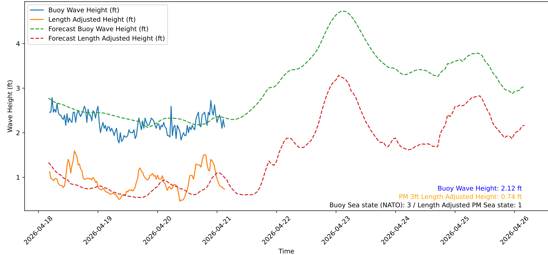
Wave Heights over Time for Red Beach at 2026-04-21 04:20:52
