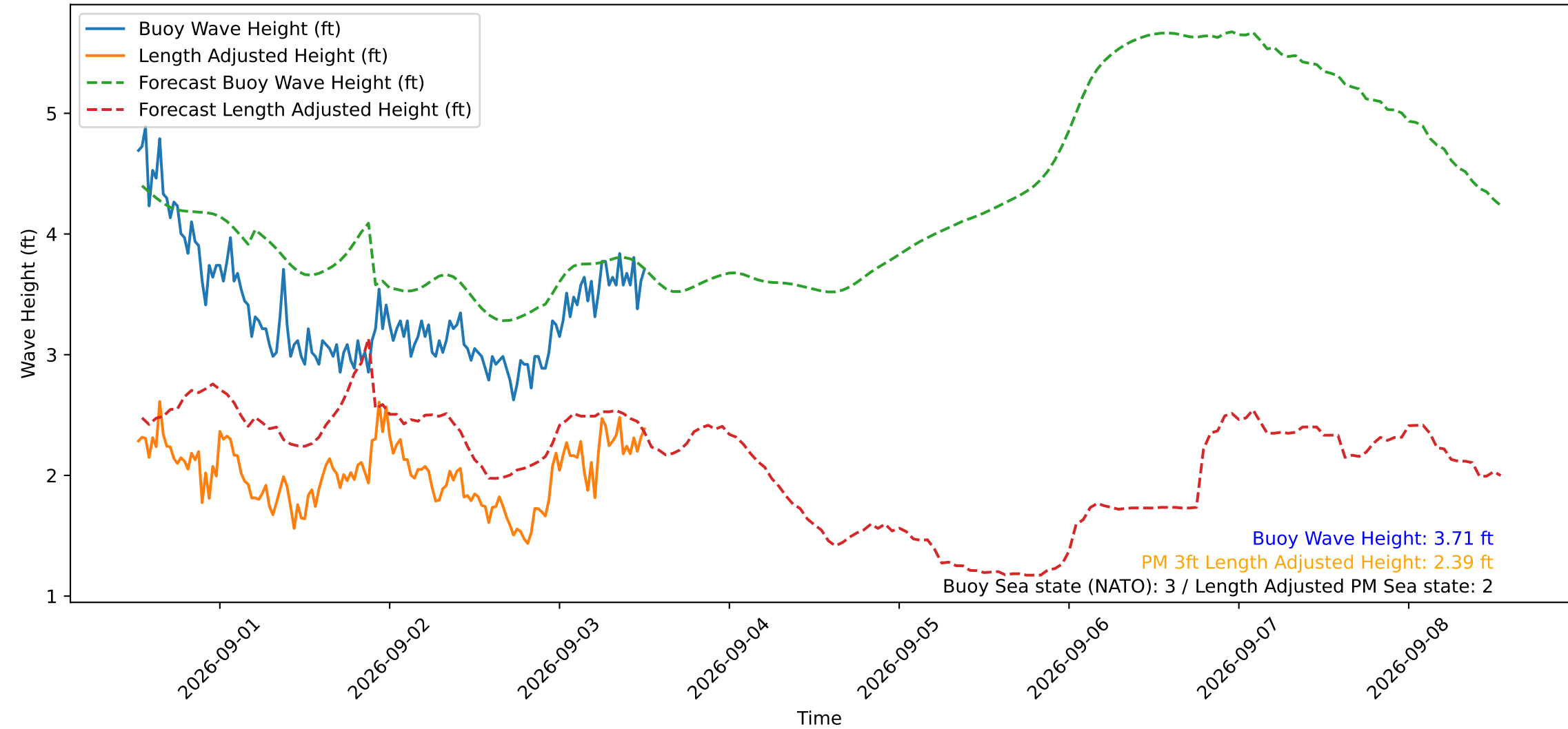
Wave Heights over Time for Oceanside Harbor at 2026-09-03 12:40:30
