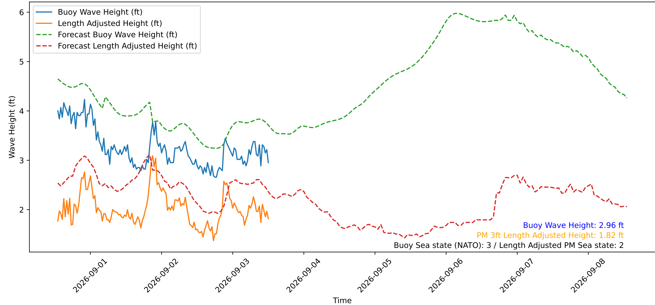
Wave Heights over Time for Green Beach at 2026-09-03 12:41:13
