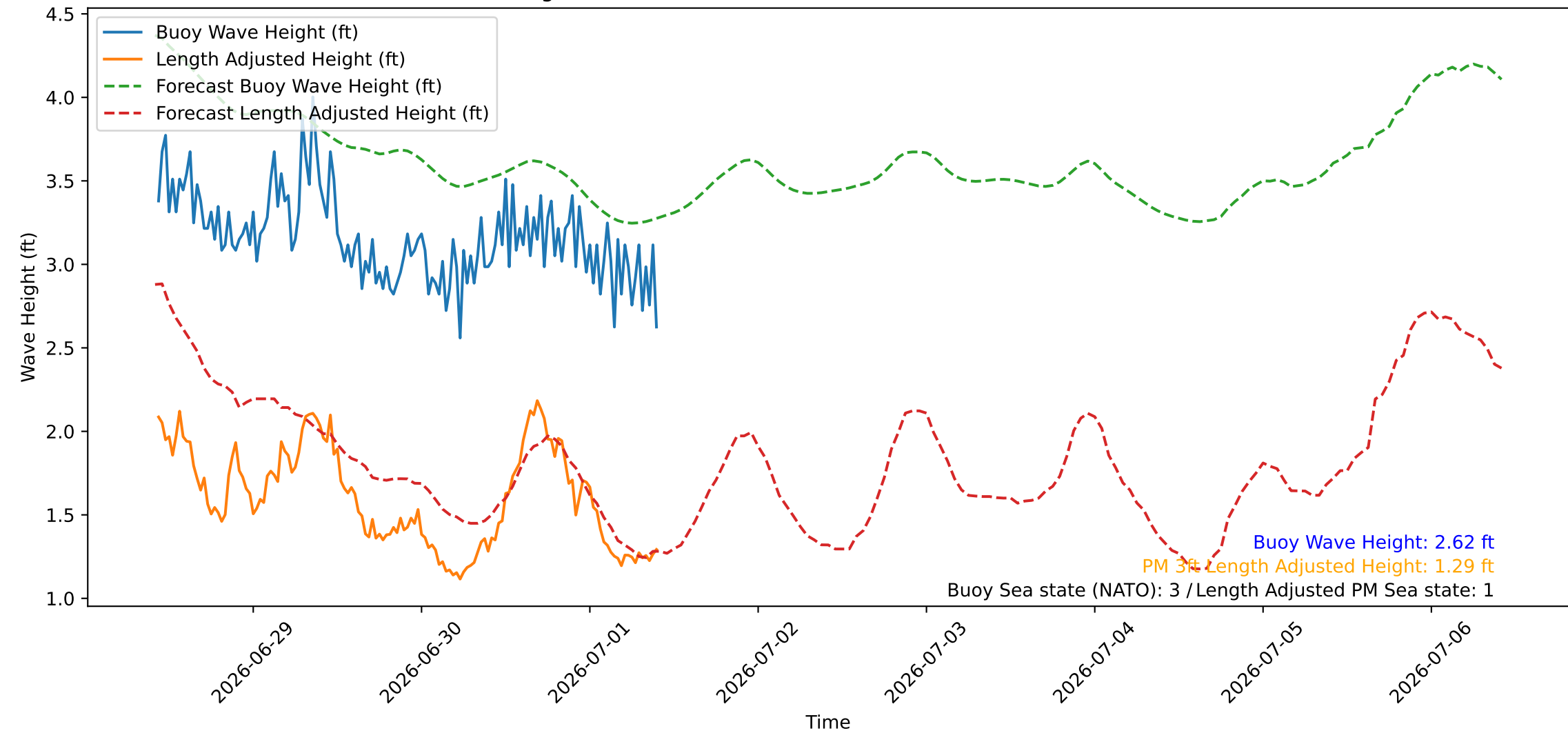
Wave Heights over Time for Oceanside Harbor at 2026-07-01 10:20:27
