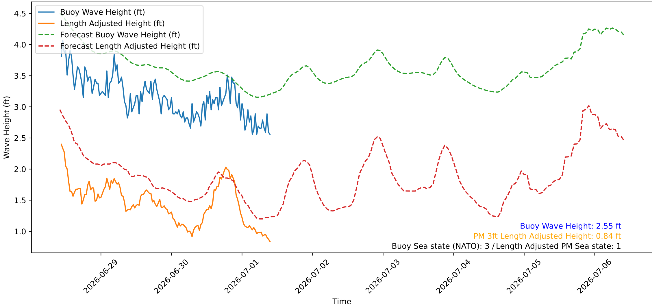
Wave Heights over Time for Green Beach at 2026-07-01 10:21:09
