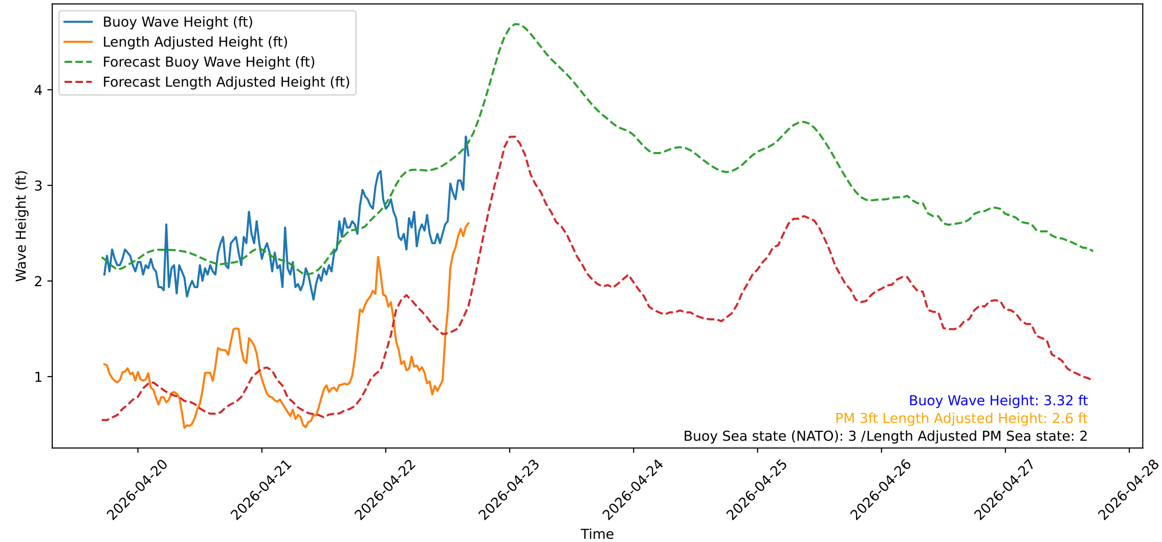
Wave Heights over Time for Red Beach at 2026-04-22 17:00:50
