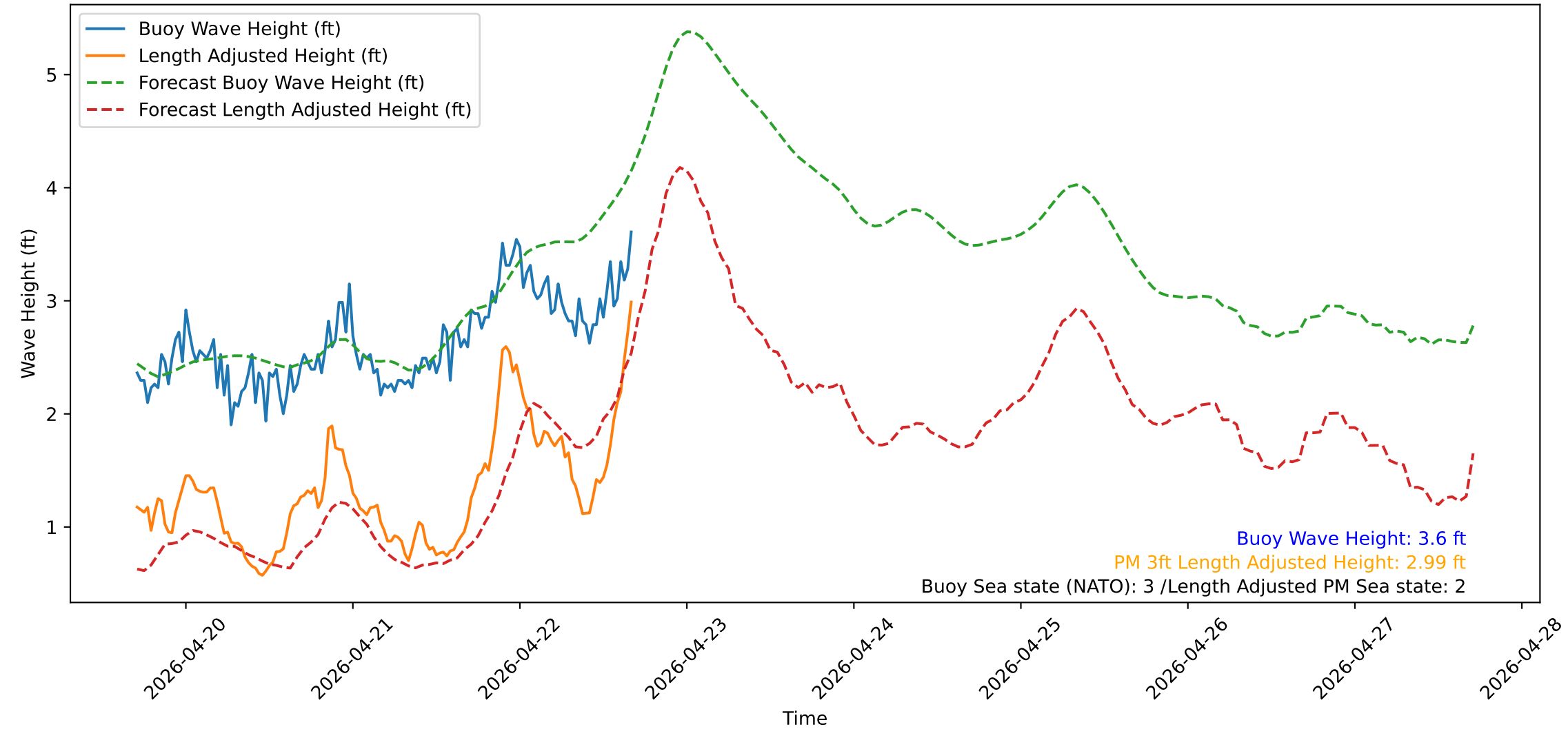
Wave Heights over Time for Green Beach at 2026-04-22 17:01:13
