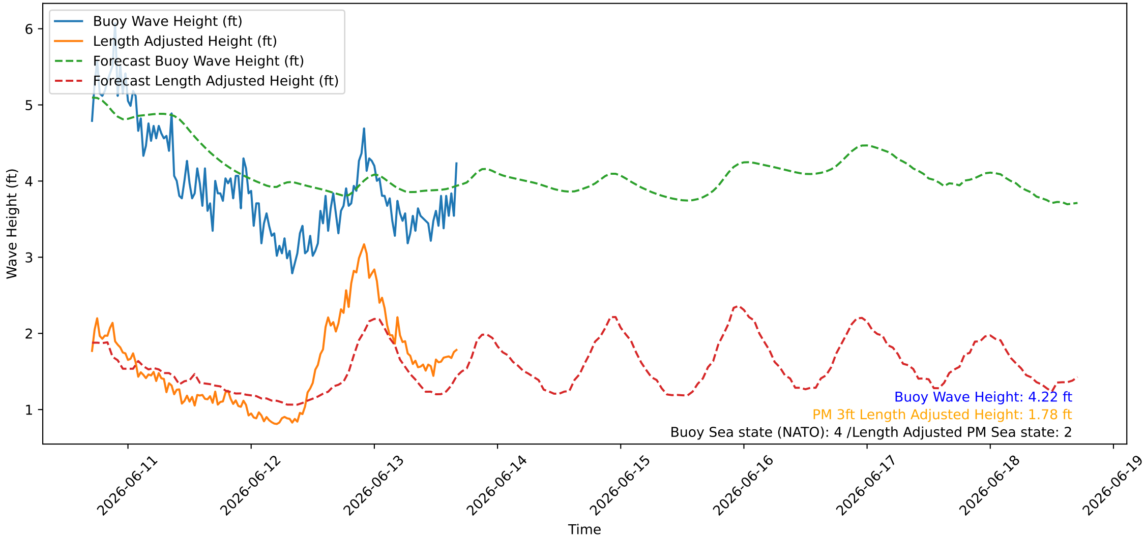
Wave Heights over Time for Oceanside Harbor at 2026-06-13 17:00:26
