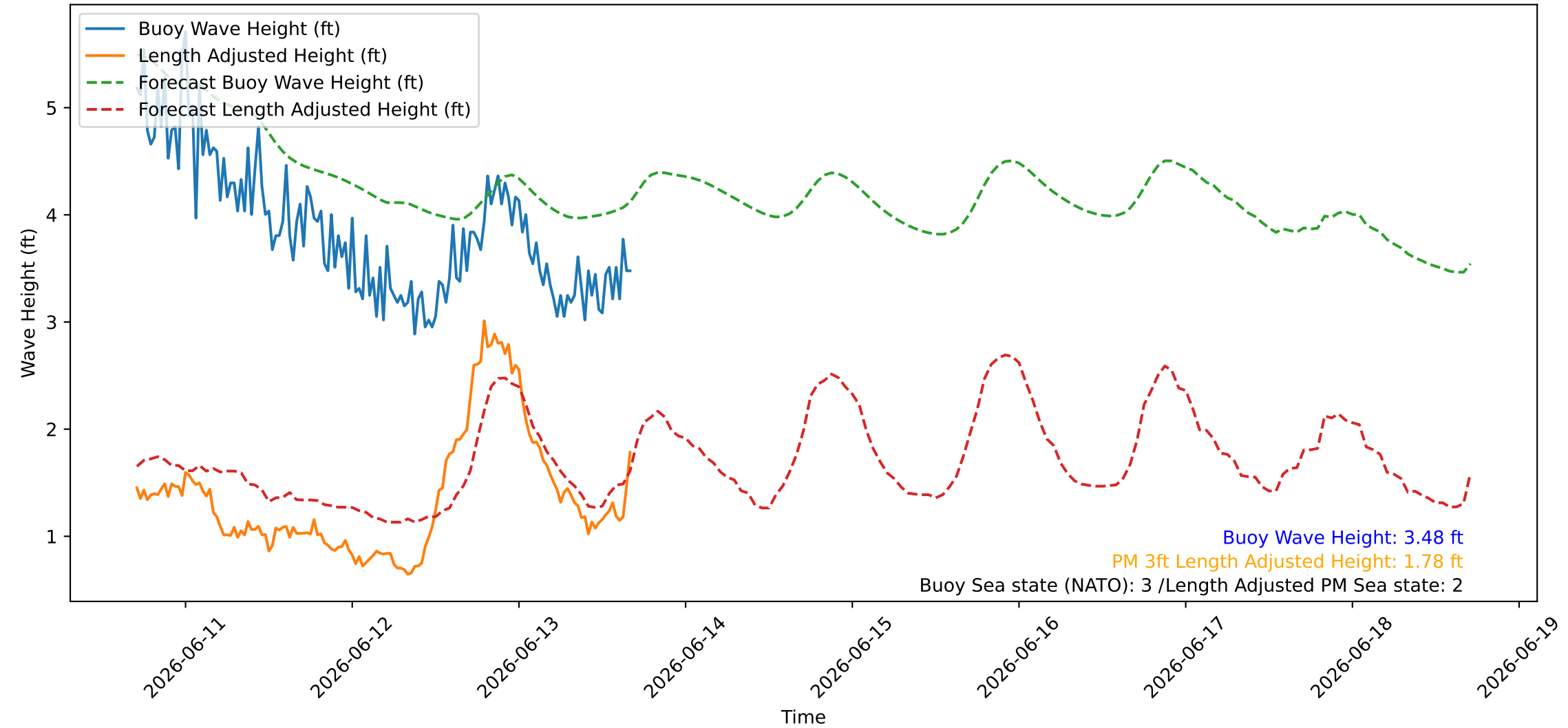
Wave Heights over Time for Green Beach at 2026-06-13 17:01:09
