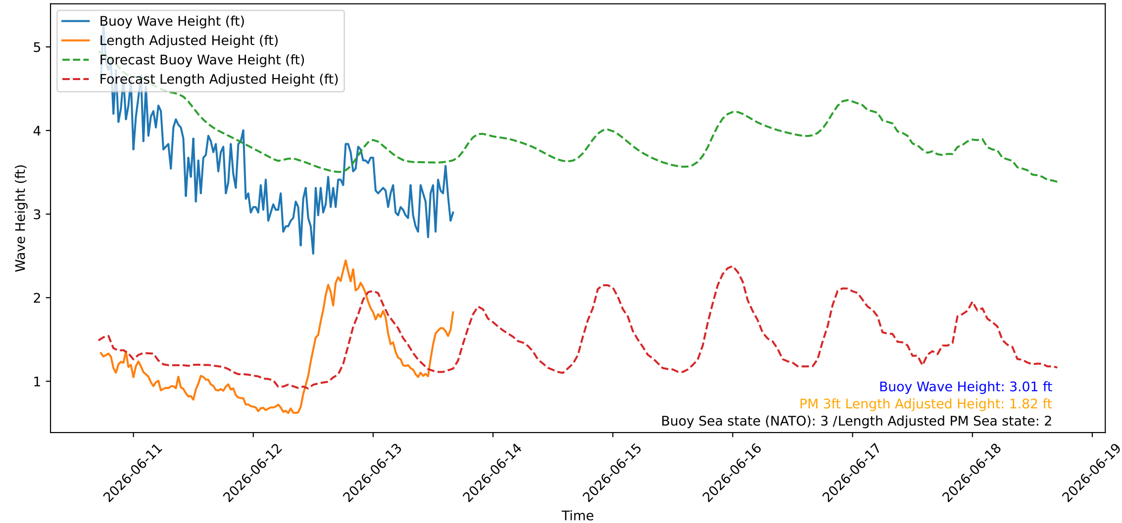
Wave Heights over Time for Red Beach at 2026-06-13 17:00:46
