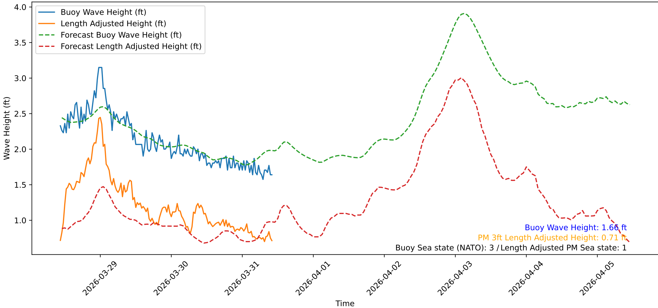
Wave Heights over Time for Oceanside Harbor at 2026-03-31 10:30:31
