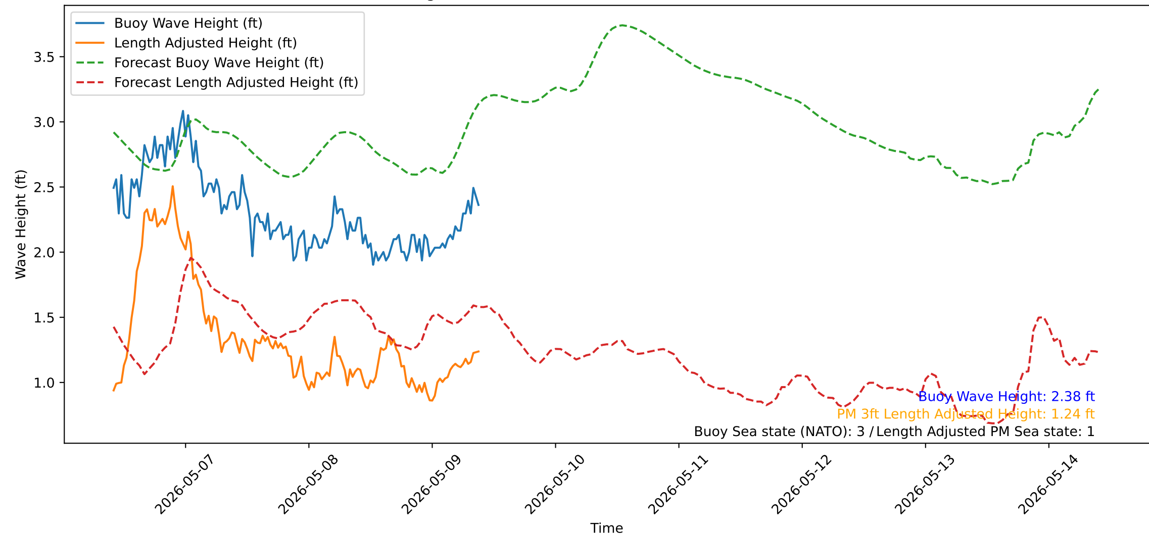
Wave Heights over Time for Red Beach at 2026-05-09 09:50:53
