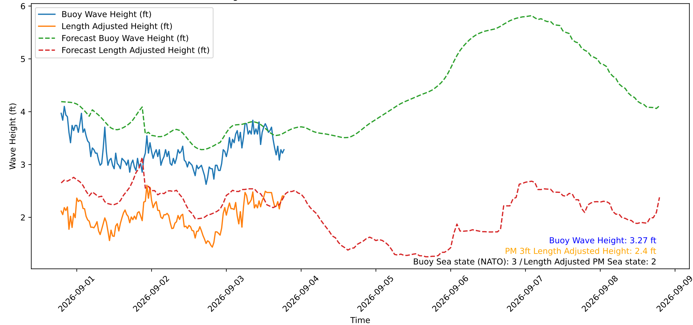
Wave Heights over Time for Oceanside Harbor at 2026-09-03 19:10:29
