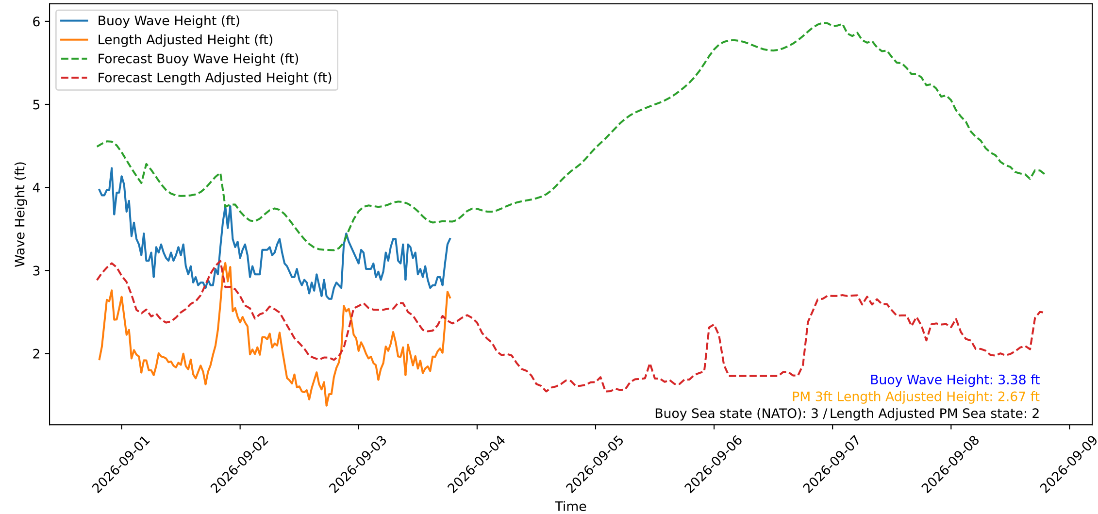
Wave Heights over Time for Green Beach at 2026-09-03 19:11:12
