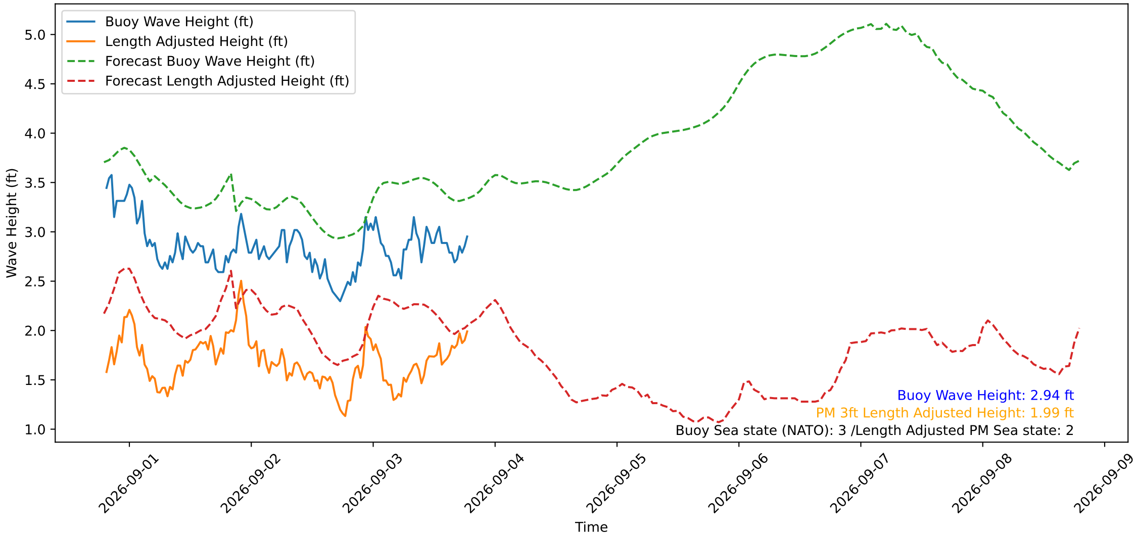
Wave Heights over Time for Red Beach at 2026-09-03 19:10:49
