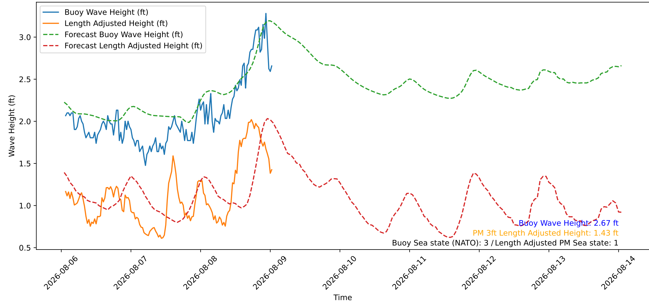
Wave Heights over Time for Red Beach at 2026-08-09 01:10:45
