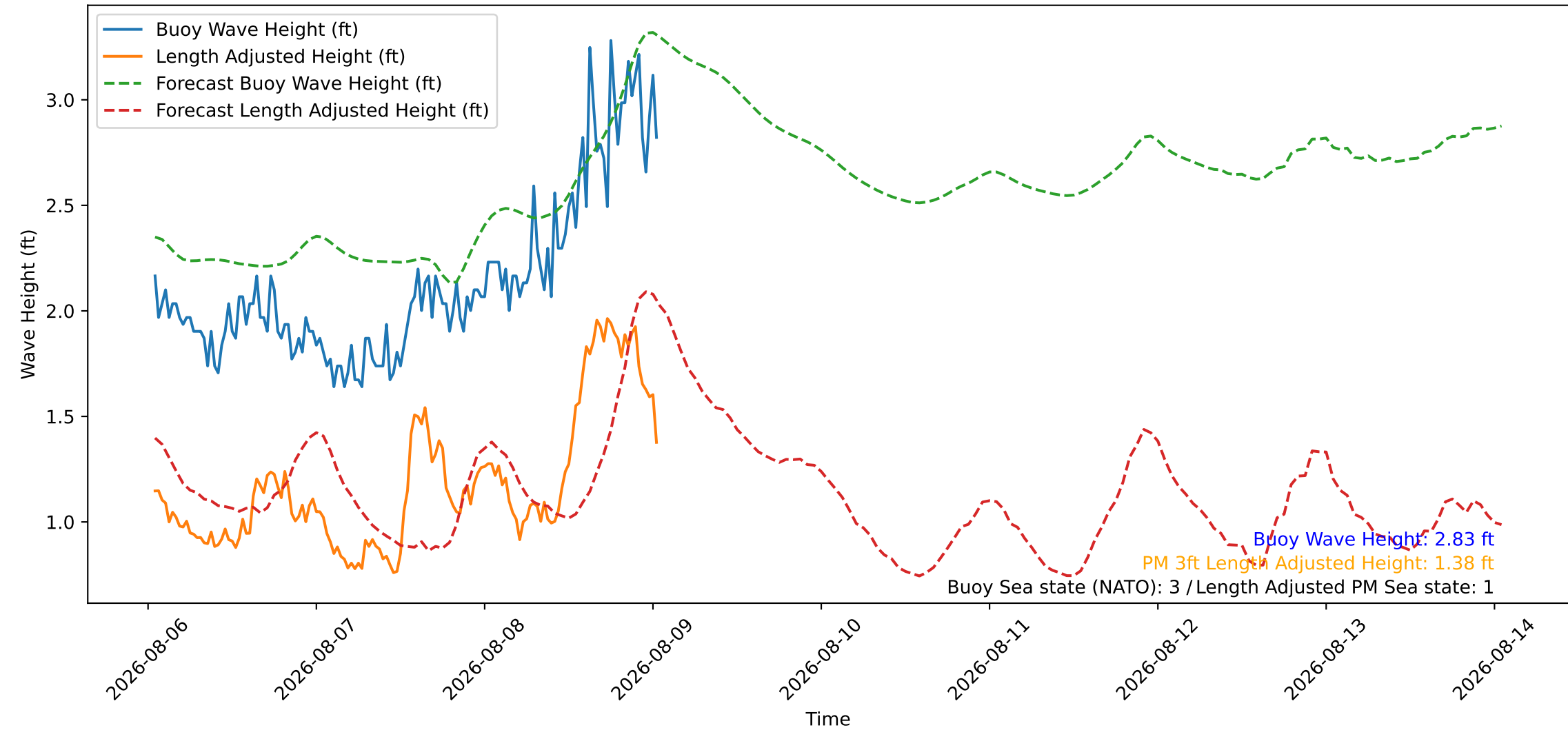
Wave Heights over Time for Oceanside Harbor at 2026-08-09 01:10:26
