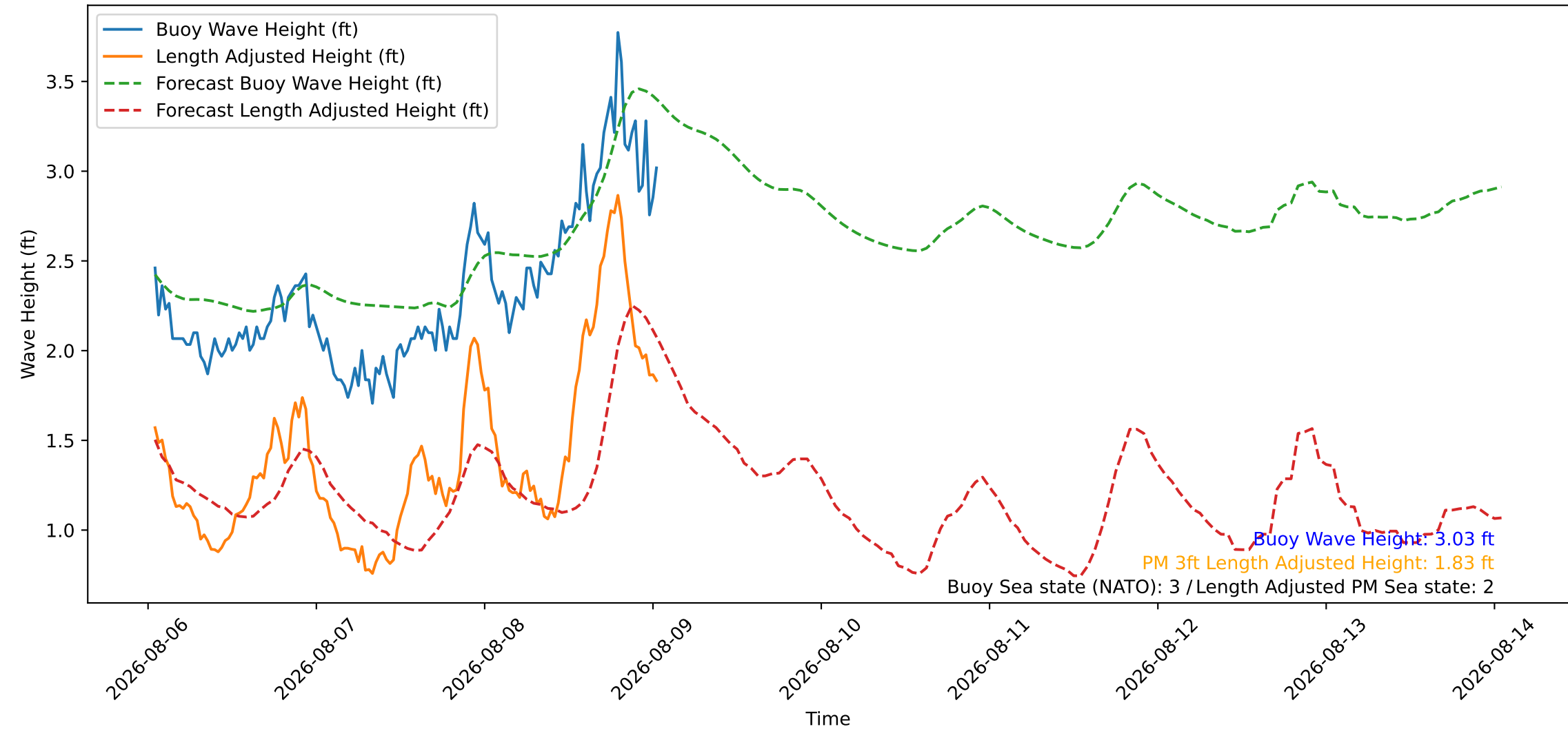
Wave Heights over Time for Green Beach at 2026-08-09 01:11:08
