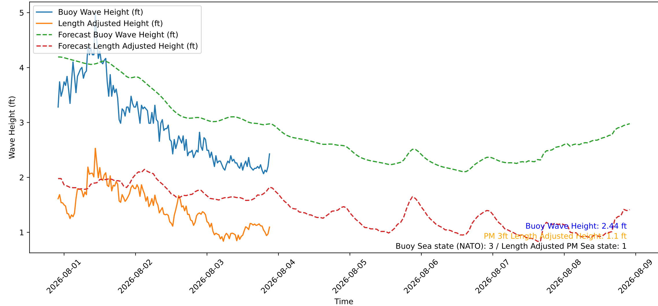
Wave Heights over Time for Green Beach at 2026-08-03 21:51:10
