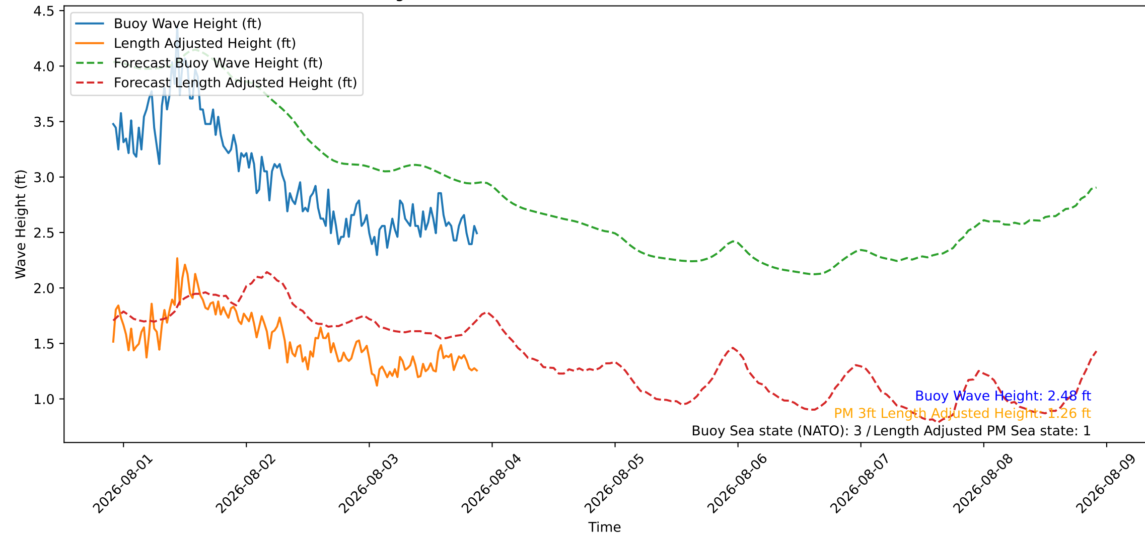
Wave Heights over Time for Oceanside Harbor at 2026-08-03 21:50:26
