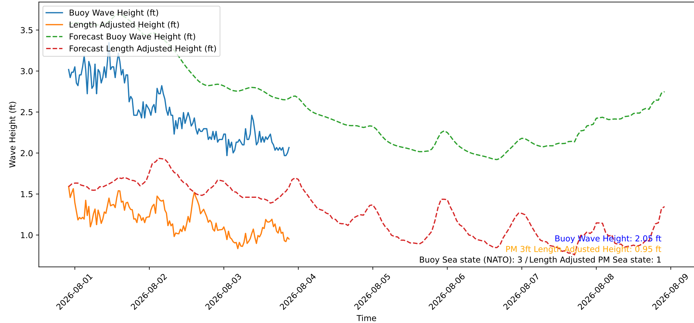
Wave Heights over Time for Red Beach at 2026-08-03 21:50:47
