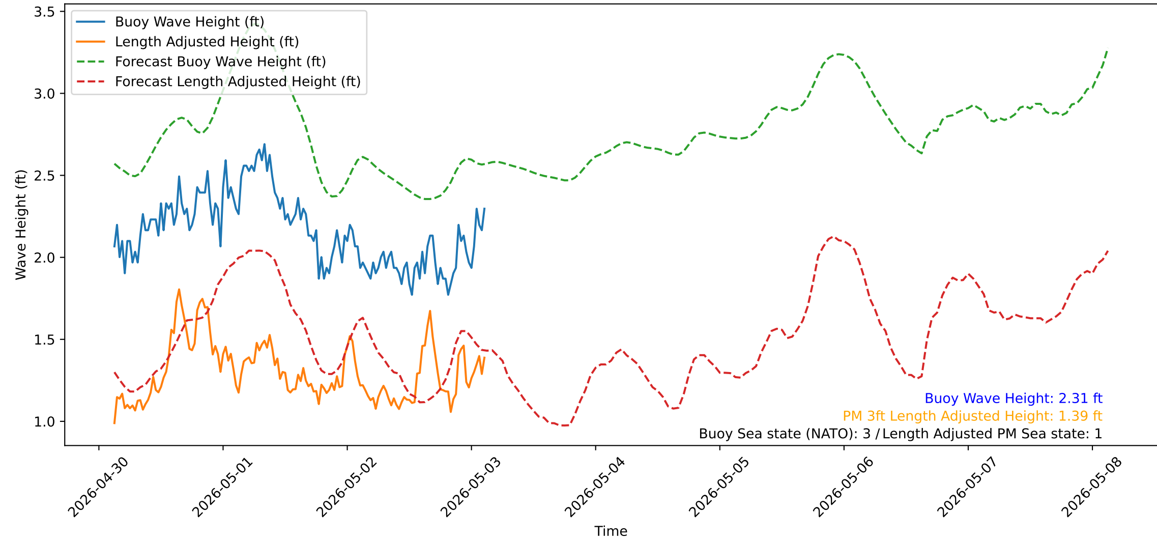
Wave Heights over Time for Oceanside Harbor at 2026-05-03 03:00:32
