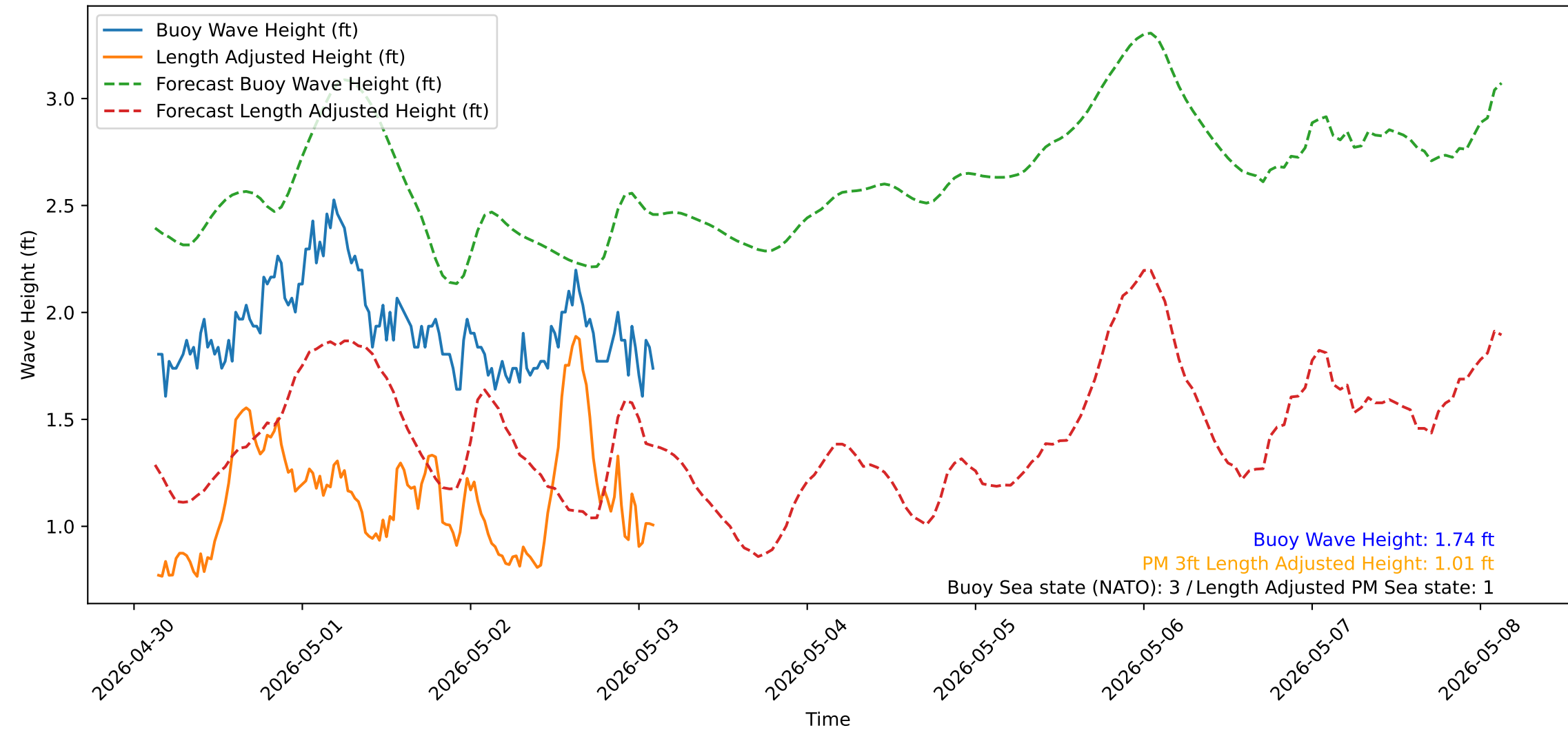
Wave Heights over Time for Red Beach at 2026-05-03 03:00:51
