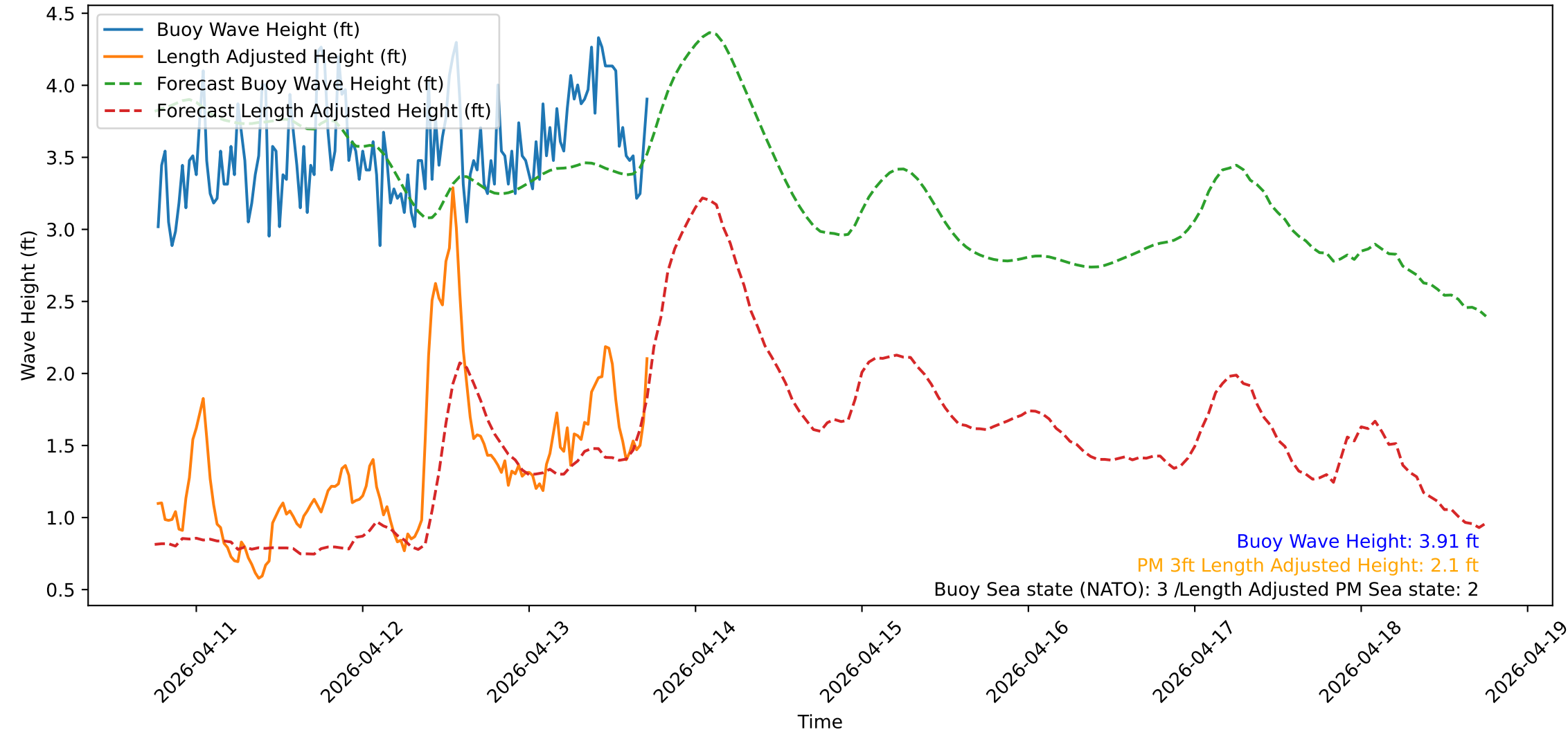
Wave Heights over Time for Red Beach at 2026-04-13 18:00:50
