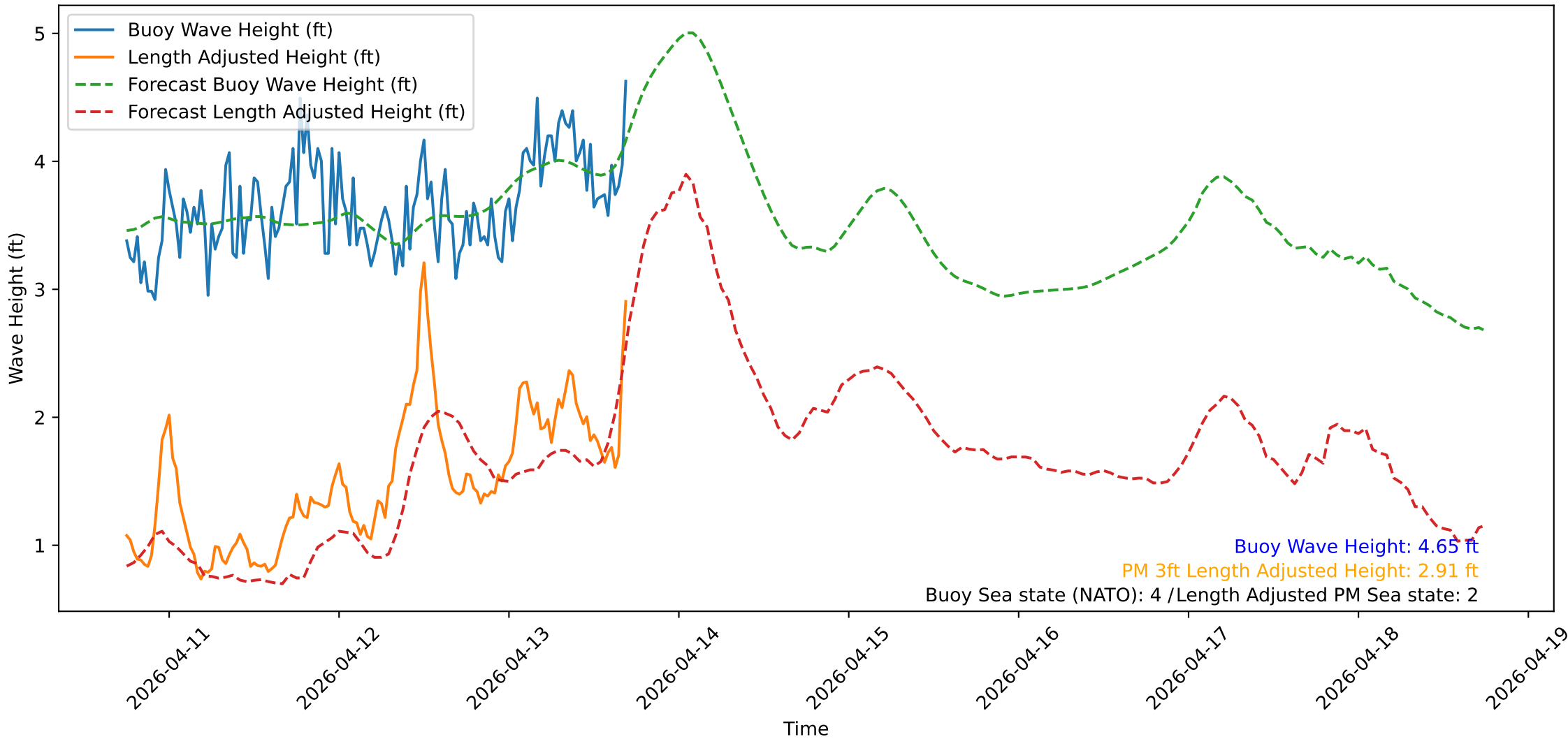
Wave Heights over Time for Green Beach at 2026-04-13 18:01:12
