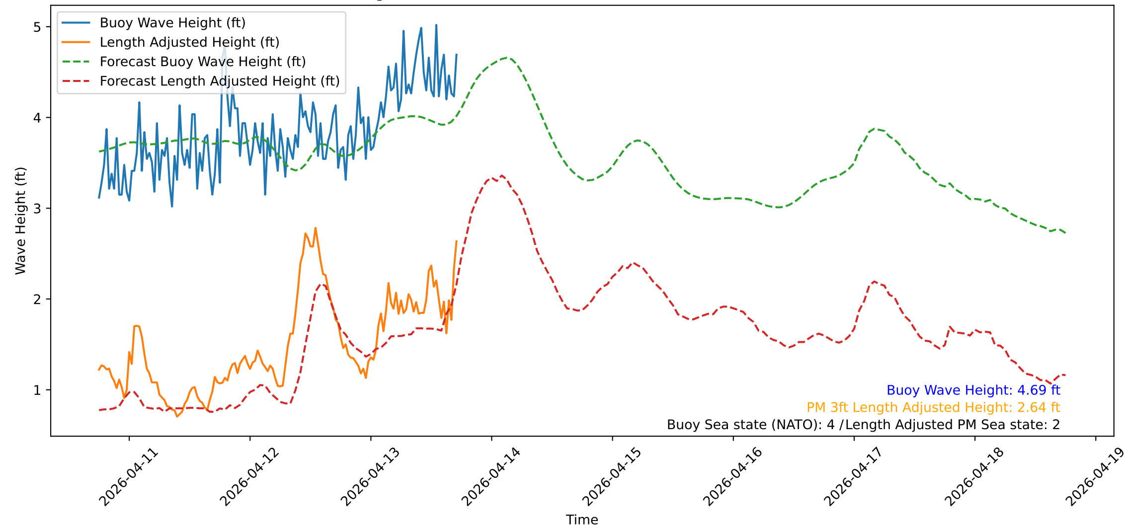
Wave Heights over Time for Oceanside Harbor at 2026-04-13 18:00:31
