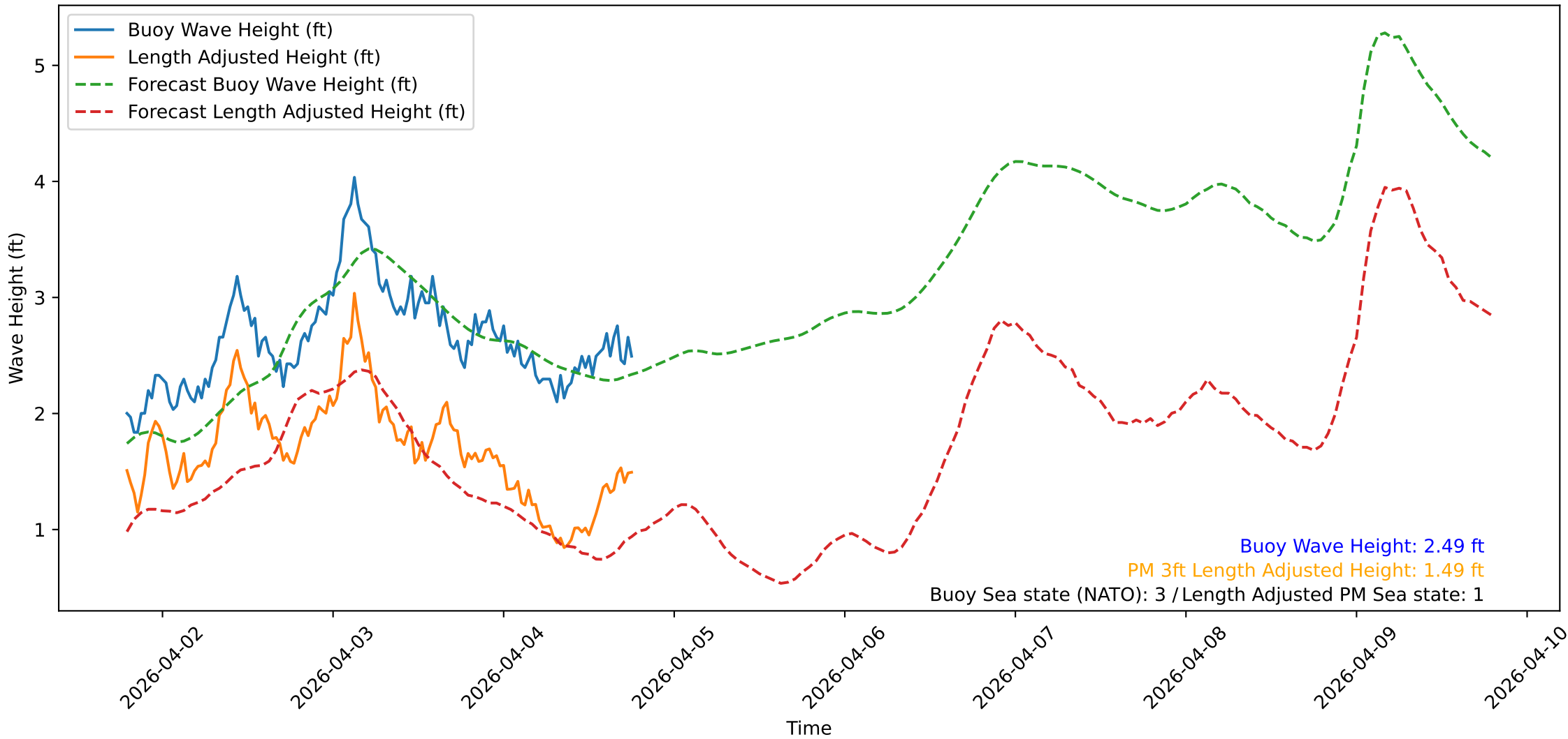
Wave Heights over Time for Oceanside Harbor at 2026-04-04 19:00:33
