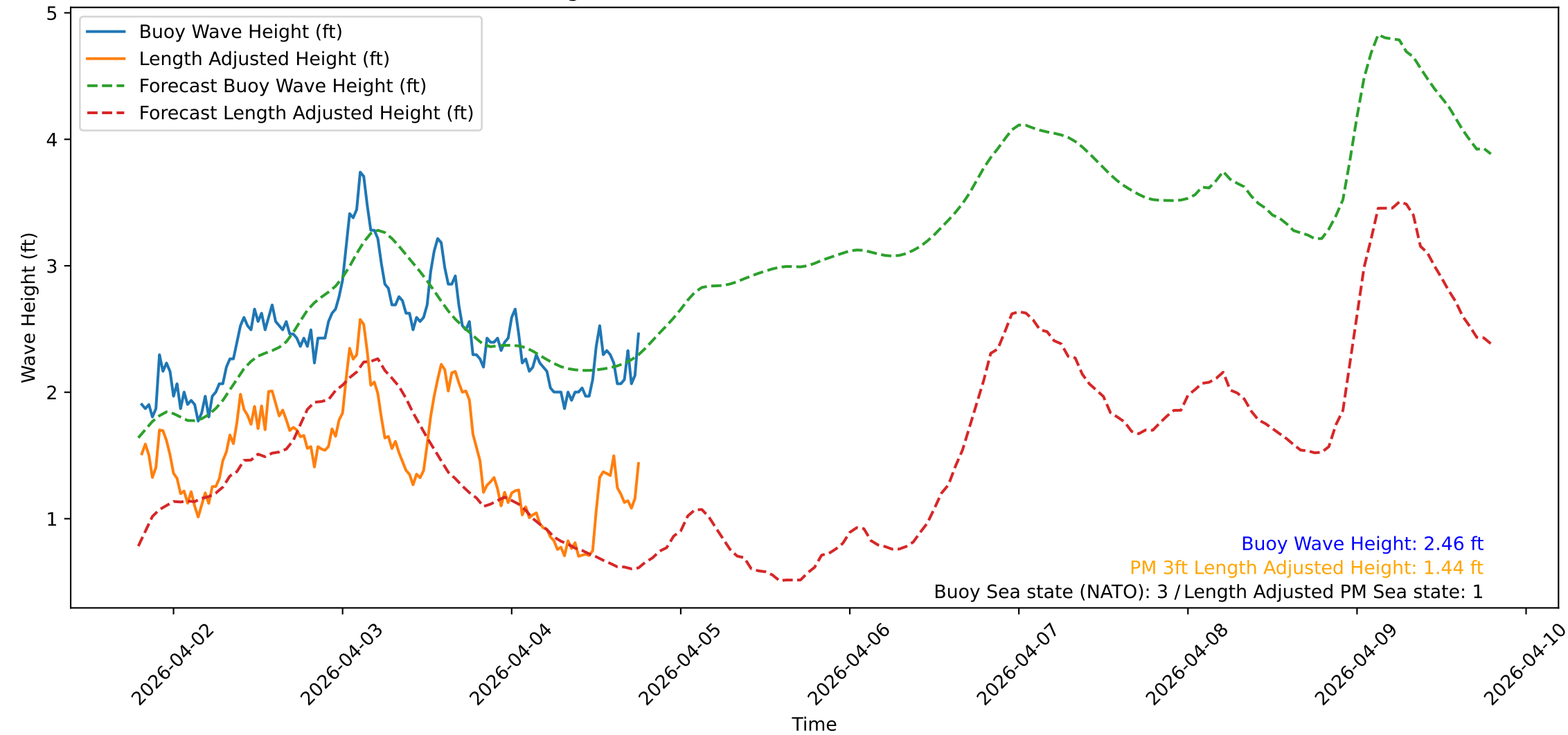
Wave Heights over Time for Red Beach at 2026-04-04 19:00:50
