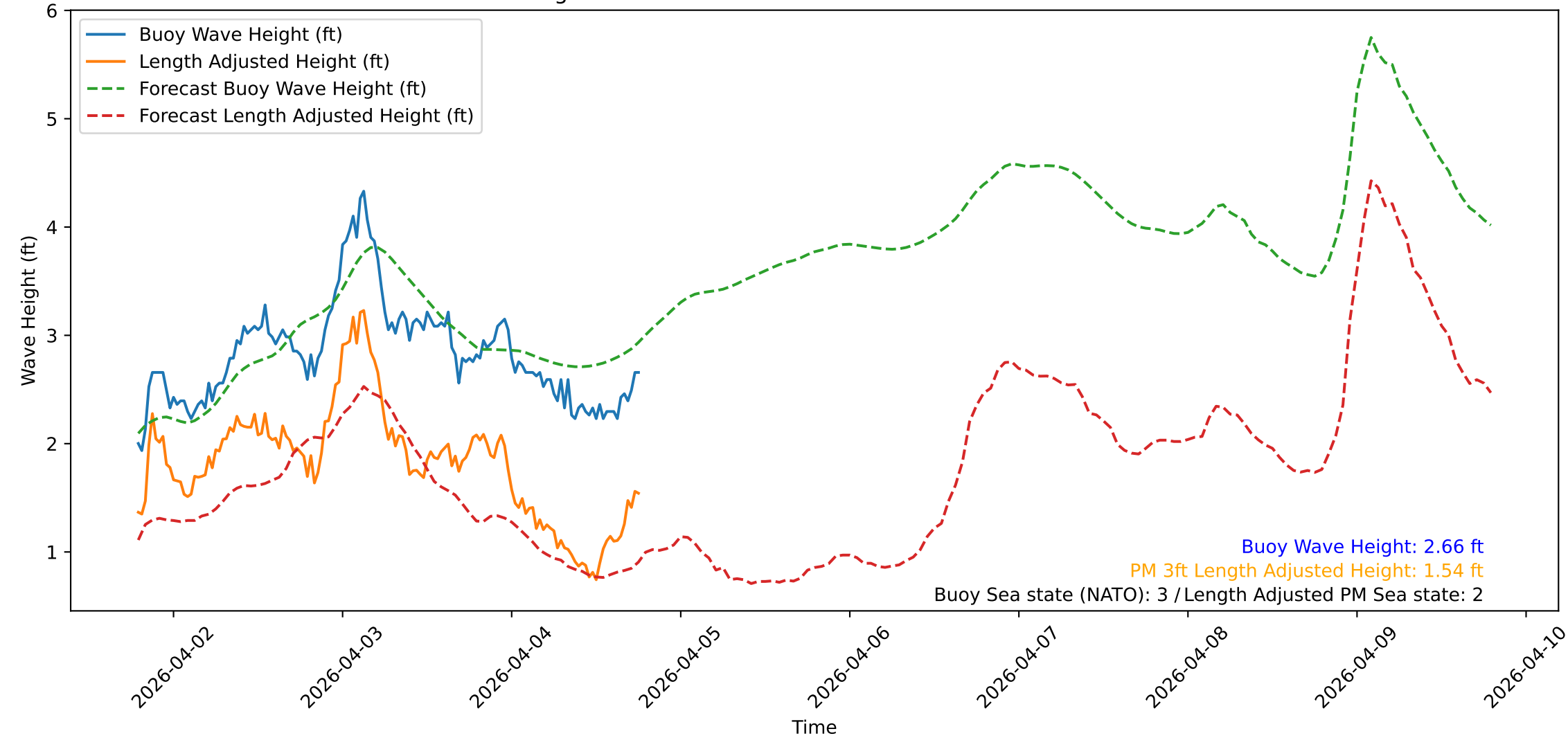
Wave Heights over Time for Green Beach at 2026-04-04 19:01:15
