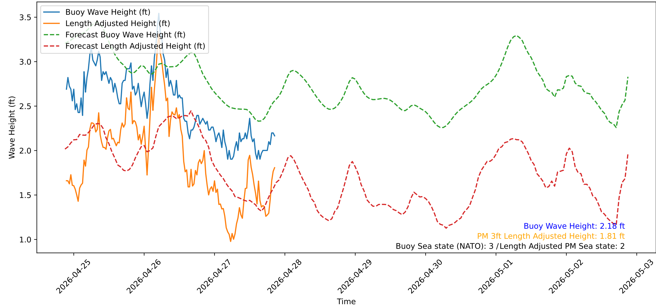
Wave Heights over Time for Red Beach at 2026-04-27 21:10:50
