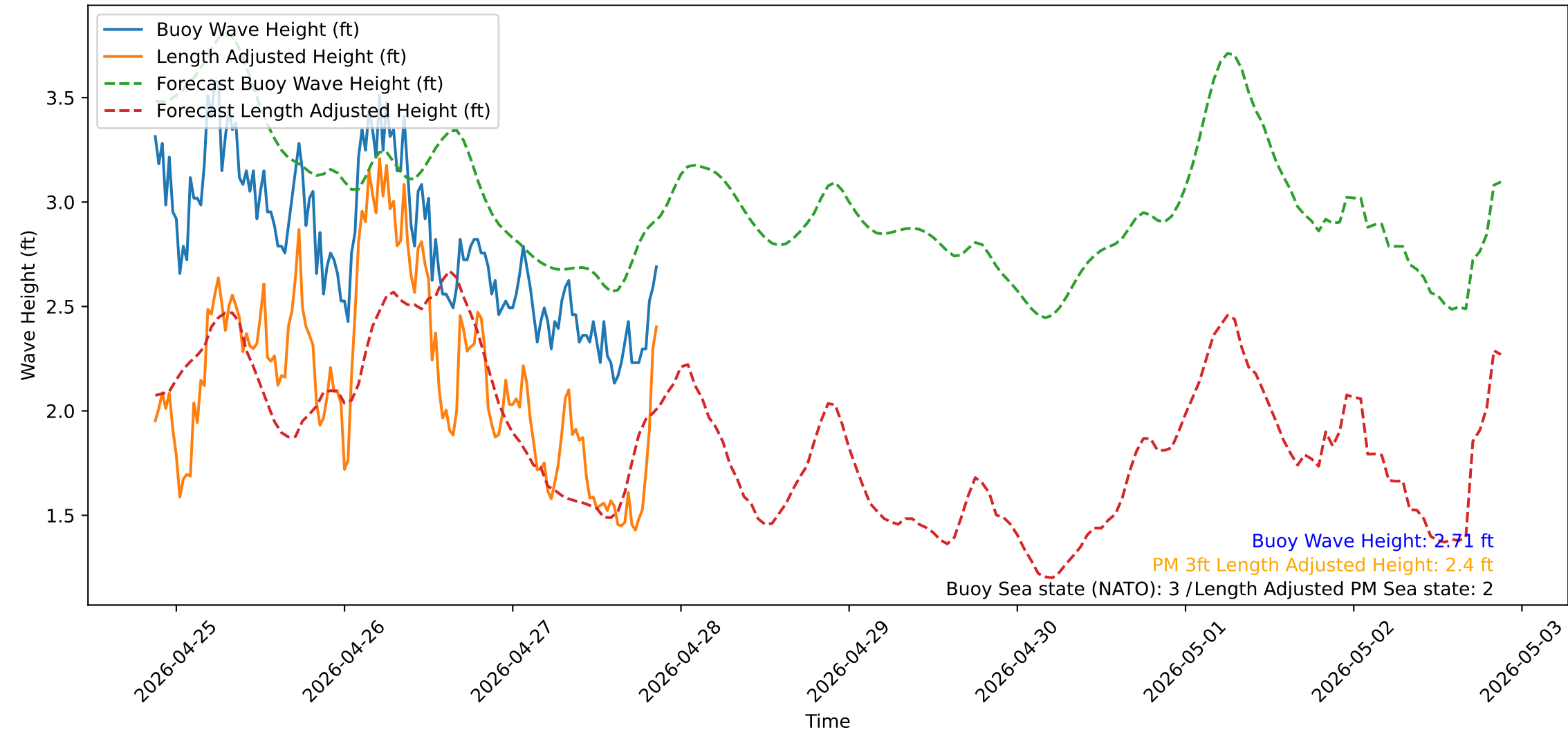
Wave Heights over Time for Green Beach at 2026-04-27 21:11:13
