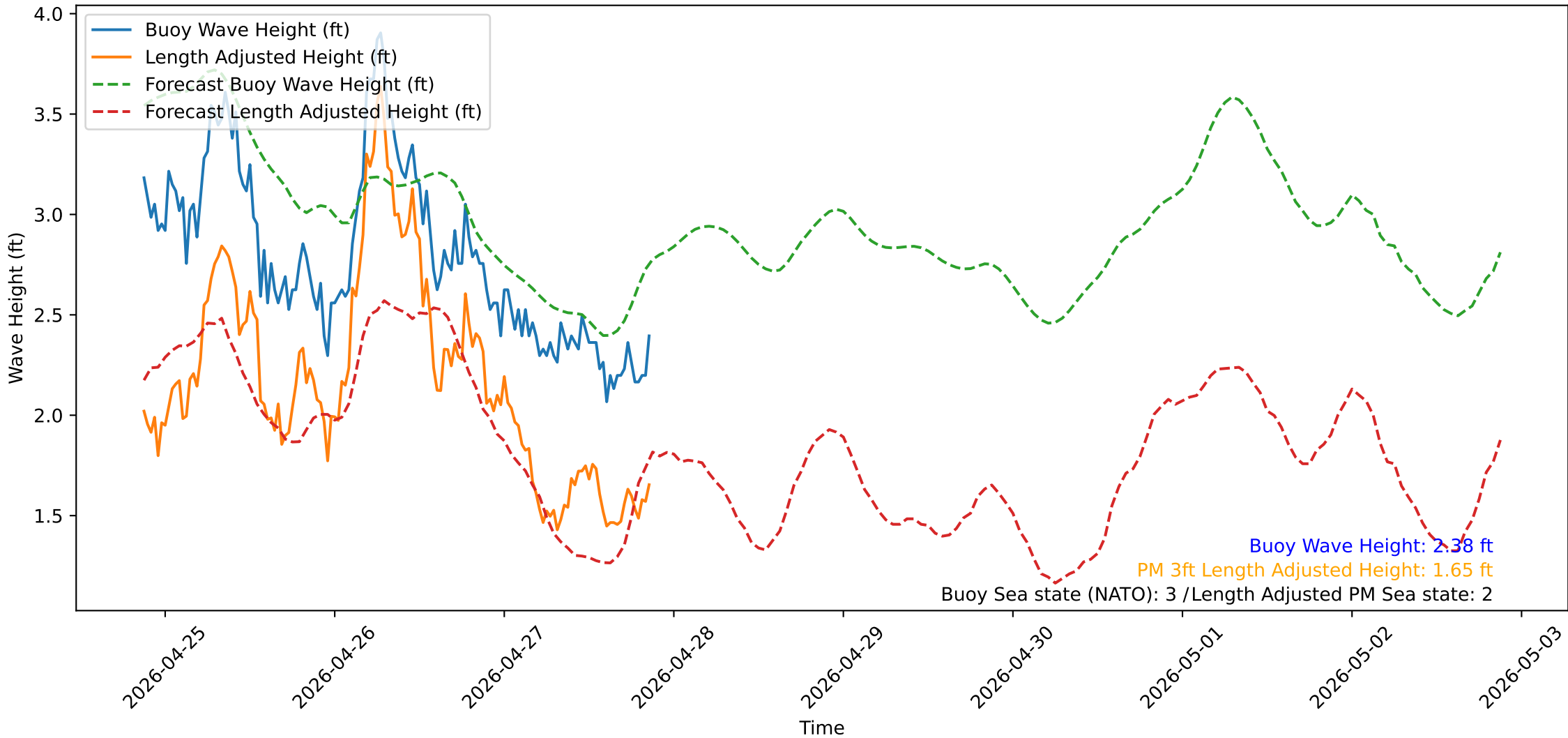
Wave Heights over Time for Oceanside Harbor at 2026-04-27 21:10:31
