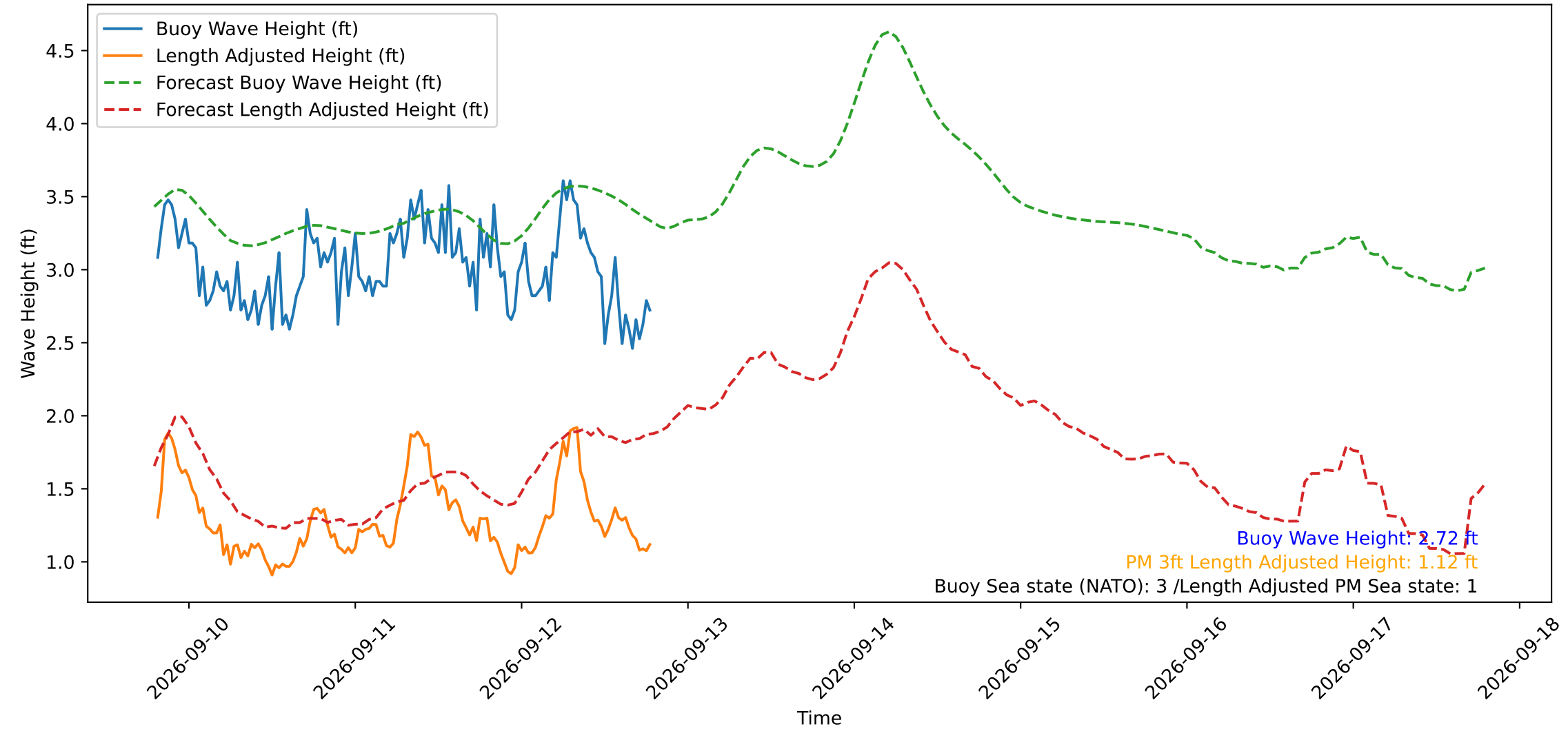
Wave Heights over Time for Green Beach at 2026-09-12 19:21:14
