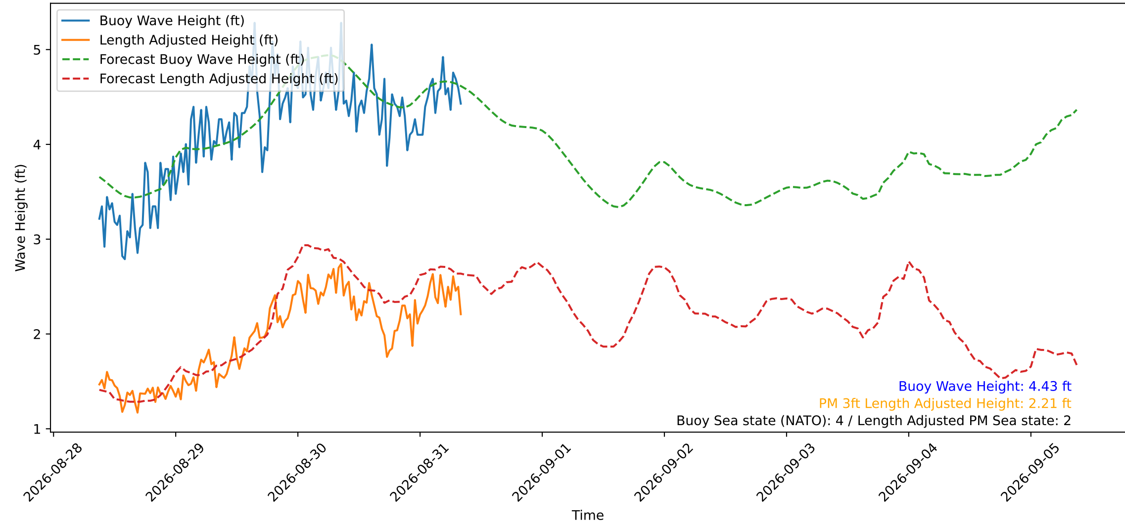
Wave Heights over Time for Oceanside Harbor at 2026-08-31 09:00:30
