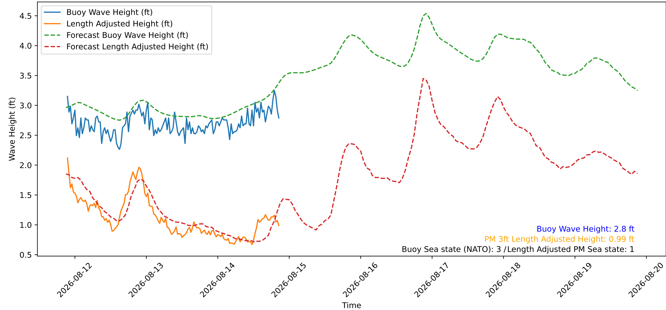
Wave Heights over Time for Green Beach at 2026-08-14 21:21:11
