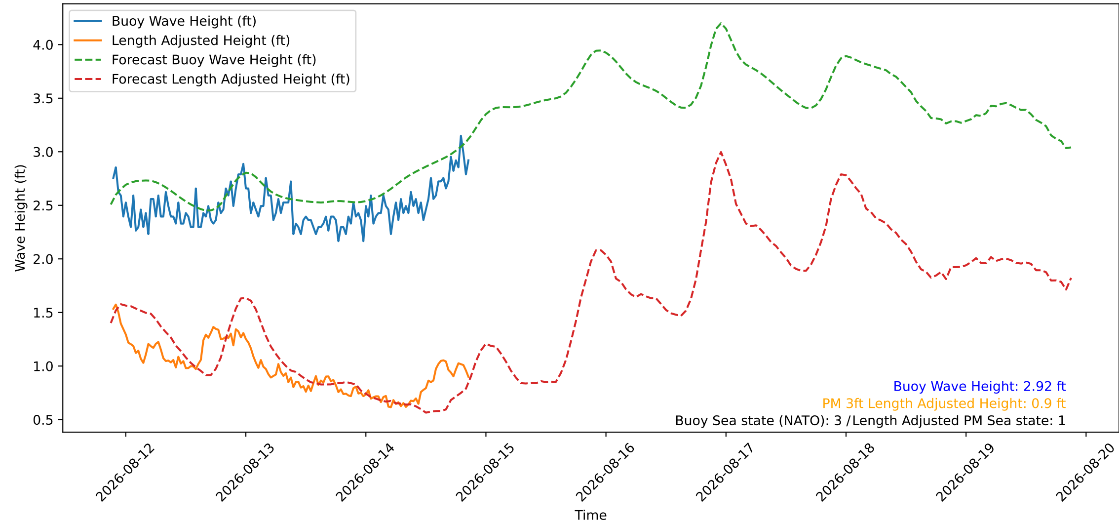
Wave Heights over Time for Red Beach at 2026-08-14 21:20:49
