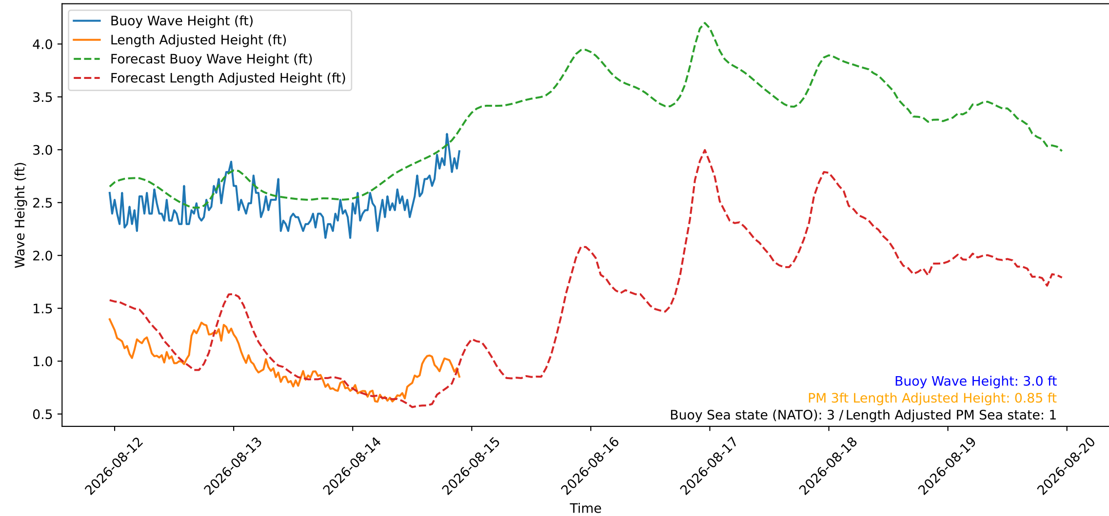
Wave Heights over Time for Red Beach at 2026-08-14 22:30:46
