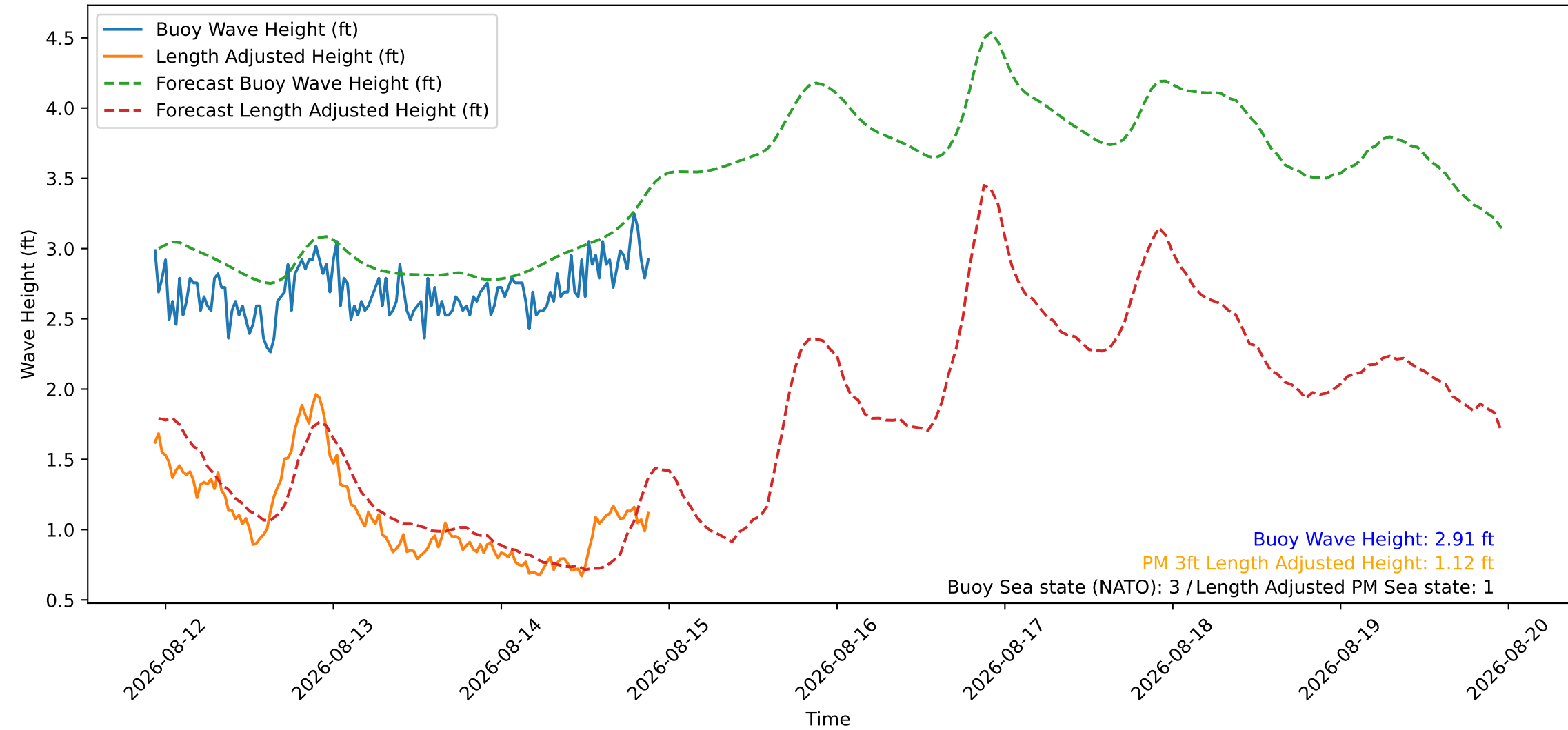
Wave Heights over Time for Green Beach at 2026-08-14 22:31:08
