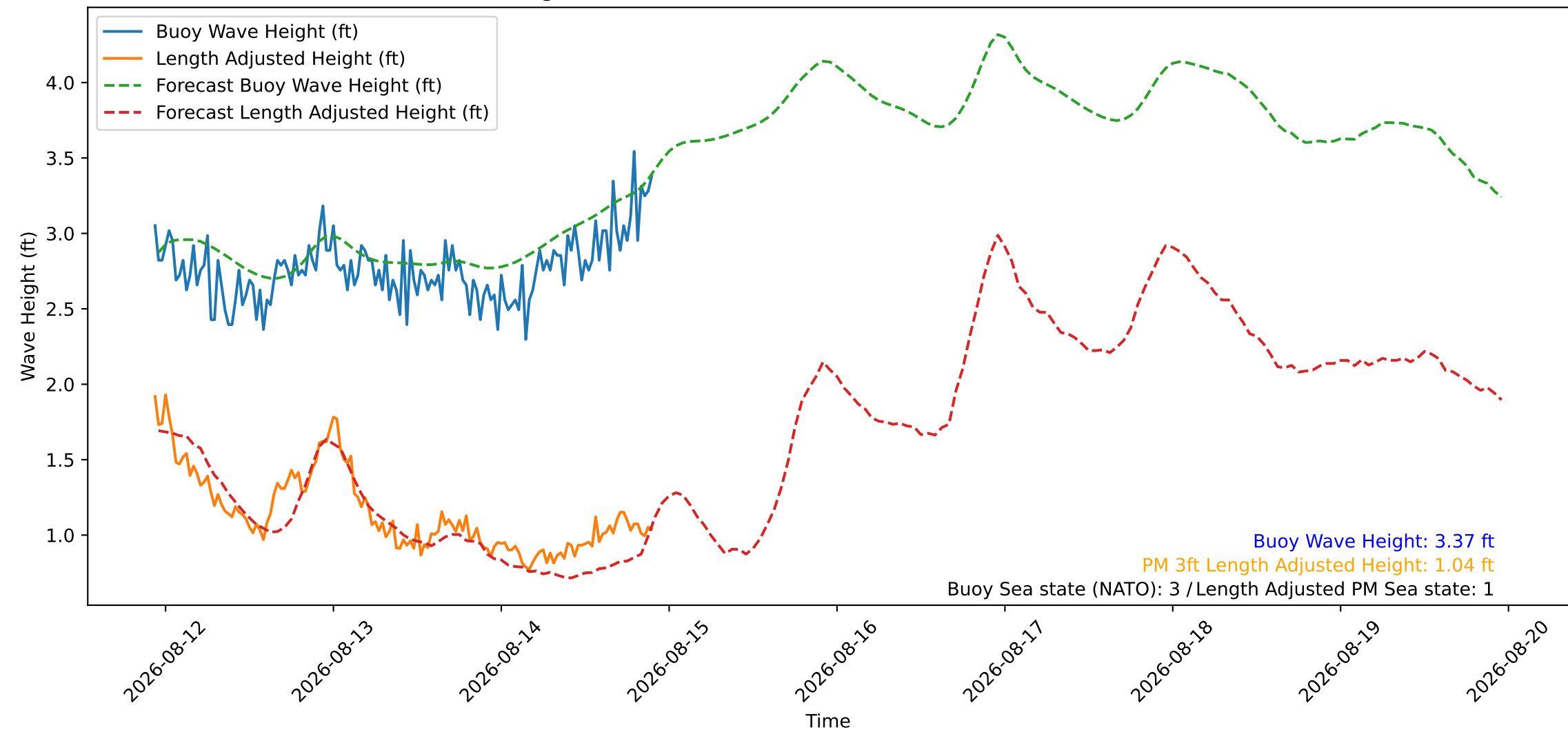
Wave Heights over Time for Oceanside Harbor at 2026-08-14 22:30:26
