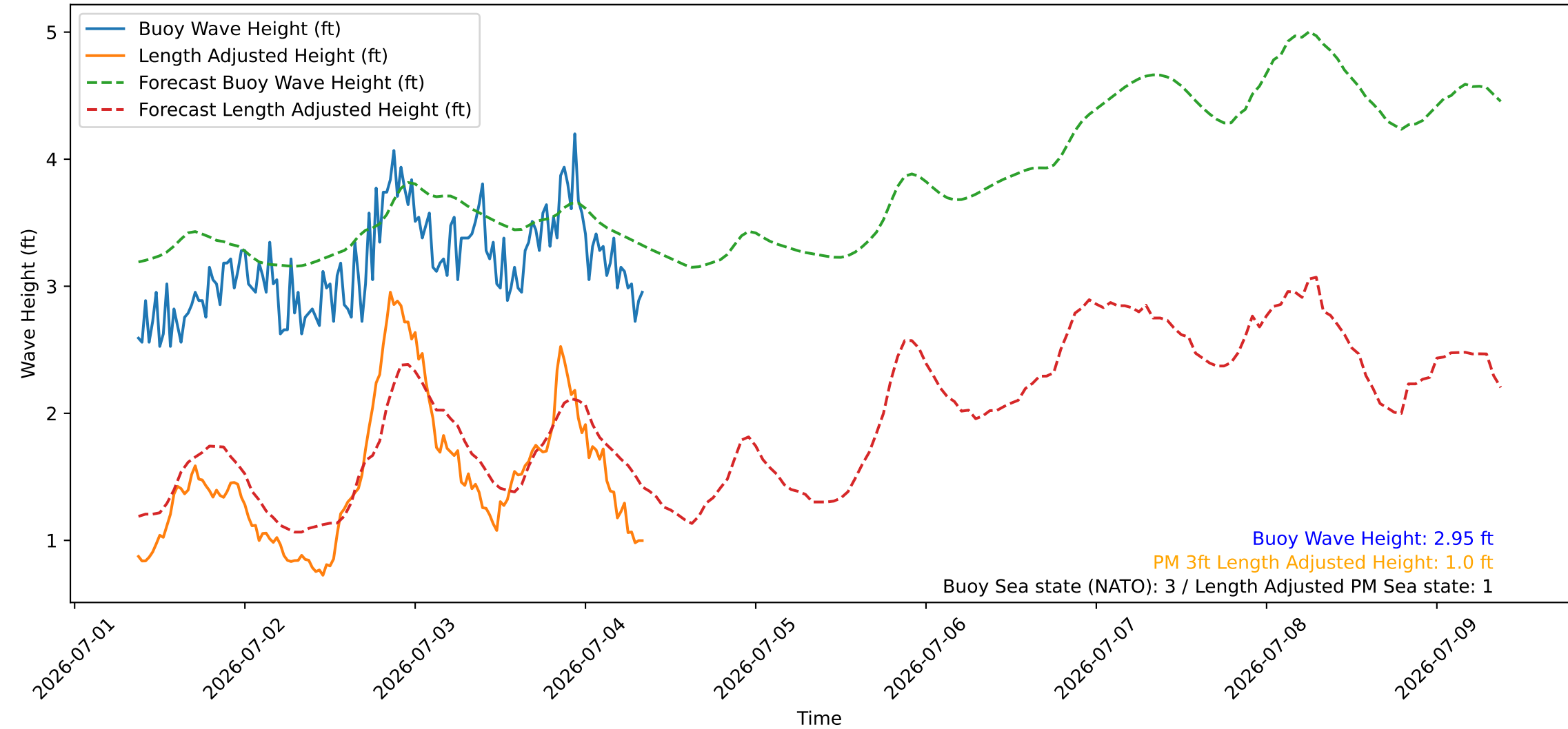
Wave Heights over Time for Green Beach at 2026-07-04 09:01:08
