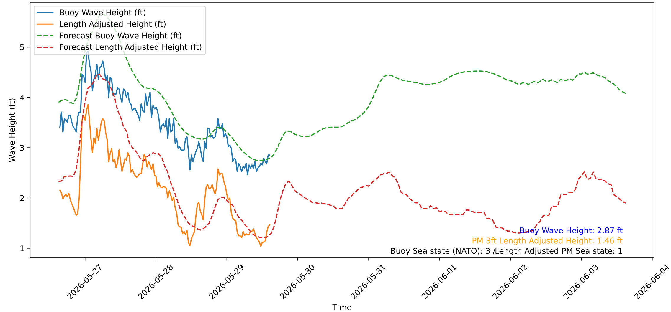
Wave Heights over Time for Green Beach at 2026-05-29 15:21:05
