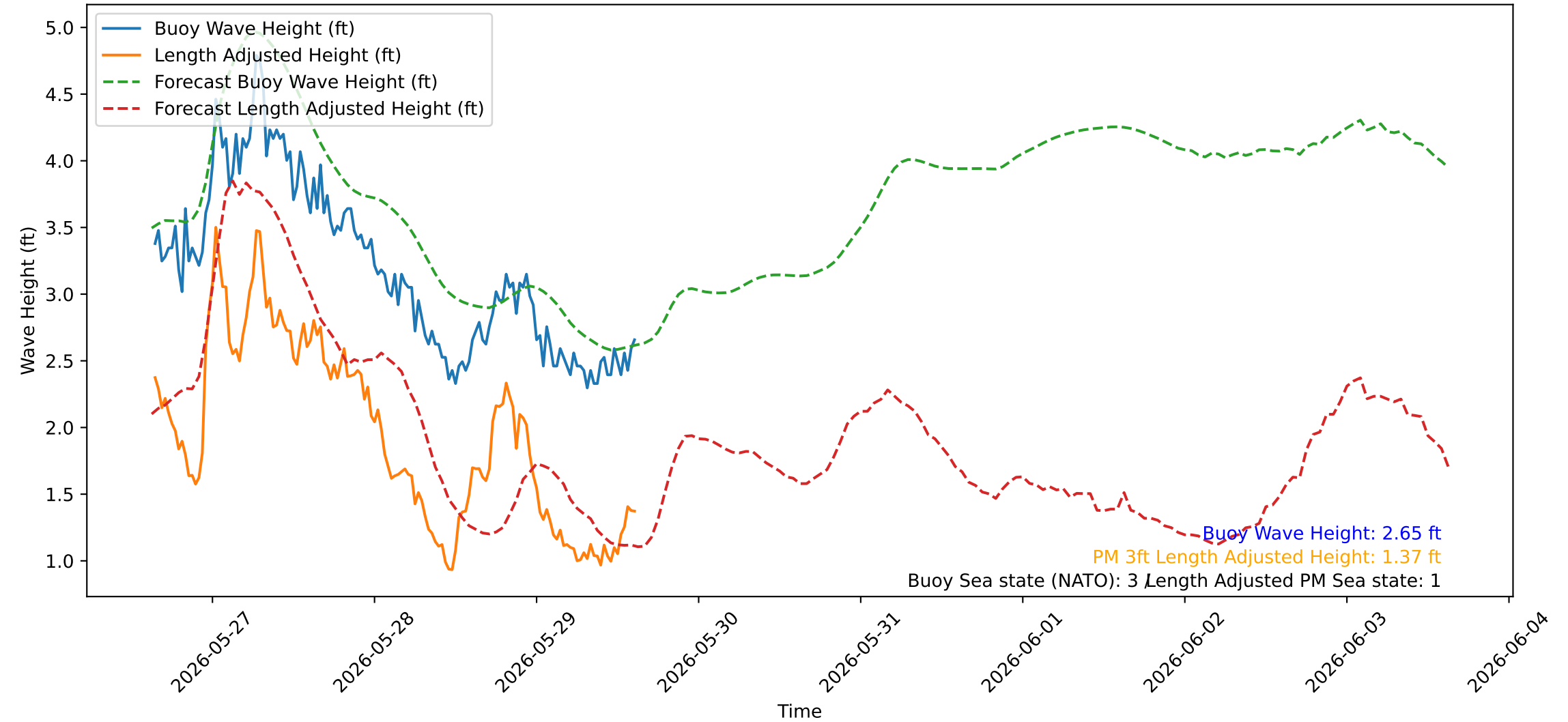
Wave Heights over Time for Red Beach at 2026-05-29 15:20:42
