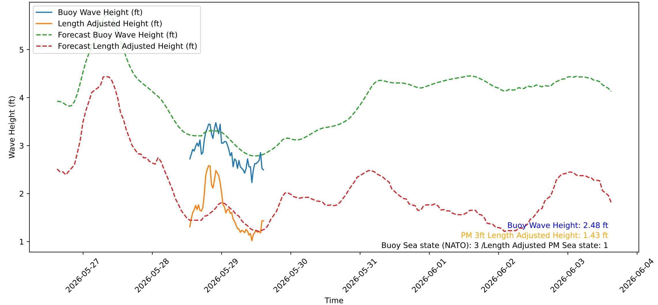
Wave Heights over Time for Oceanside Harbor at 2026-05-29 15:20:21
