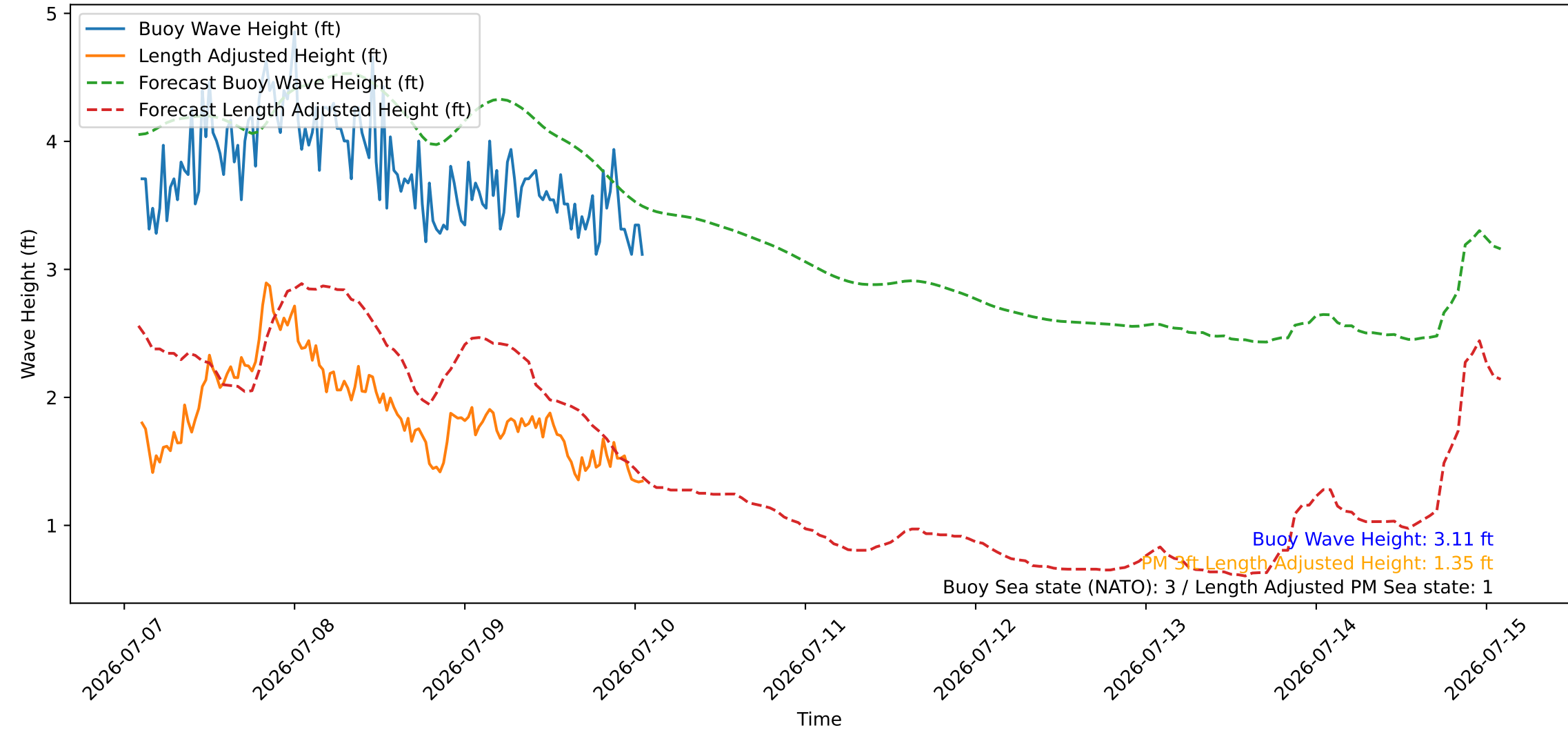
Wave Heights over Time for Red Beach at 2026-07-10 02:00:47
