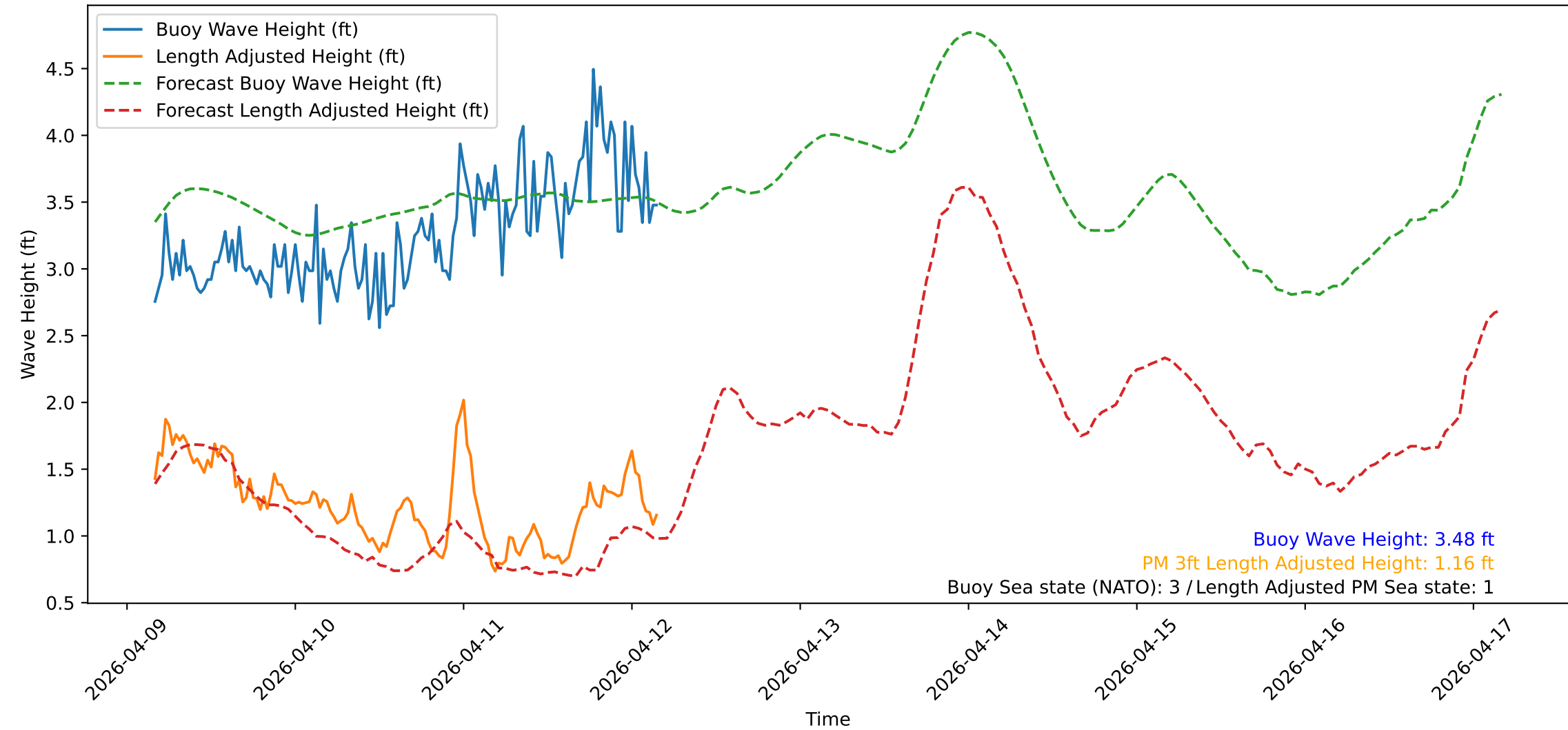
Wave Heights over Time for Green Beach at 2026-04-12 04:11:14
