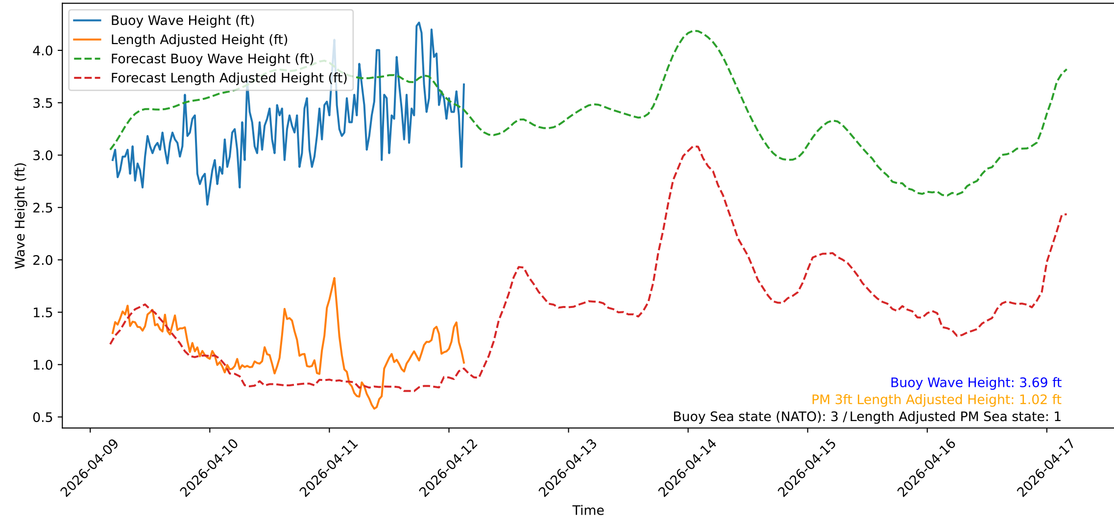
Wave Heights over Time for Red Beach at 2026-04-12 04:10:51
