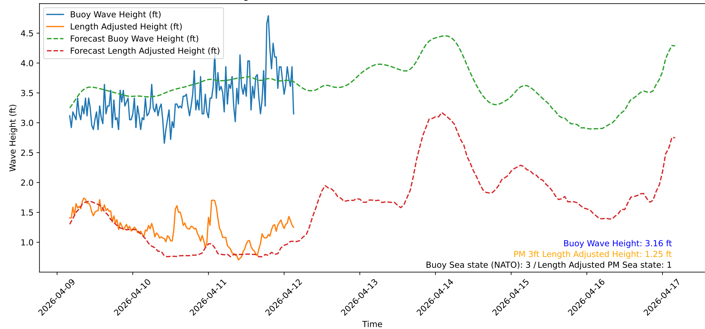
Wave Heights over Time for Oceanside Harbor at 2026-04-12 04:10:31
