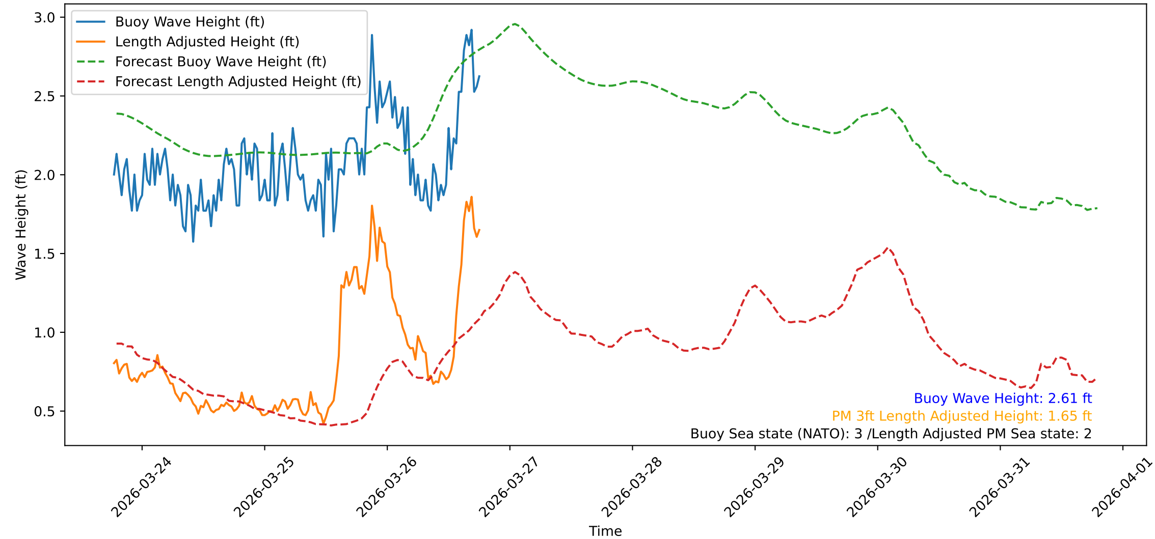
Wave Heights over Time for Oceanside Harbor at 2026-03-26 18:40:31
