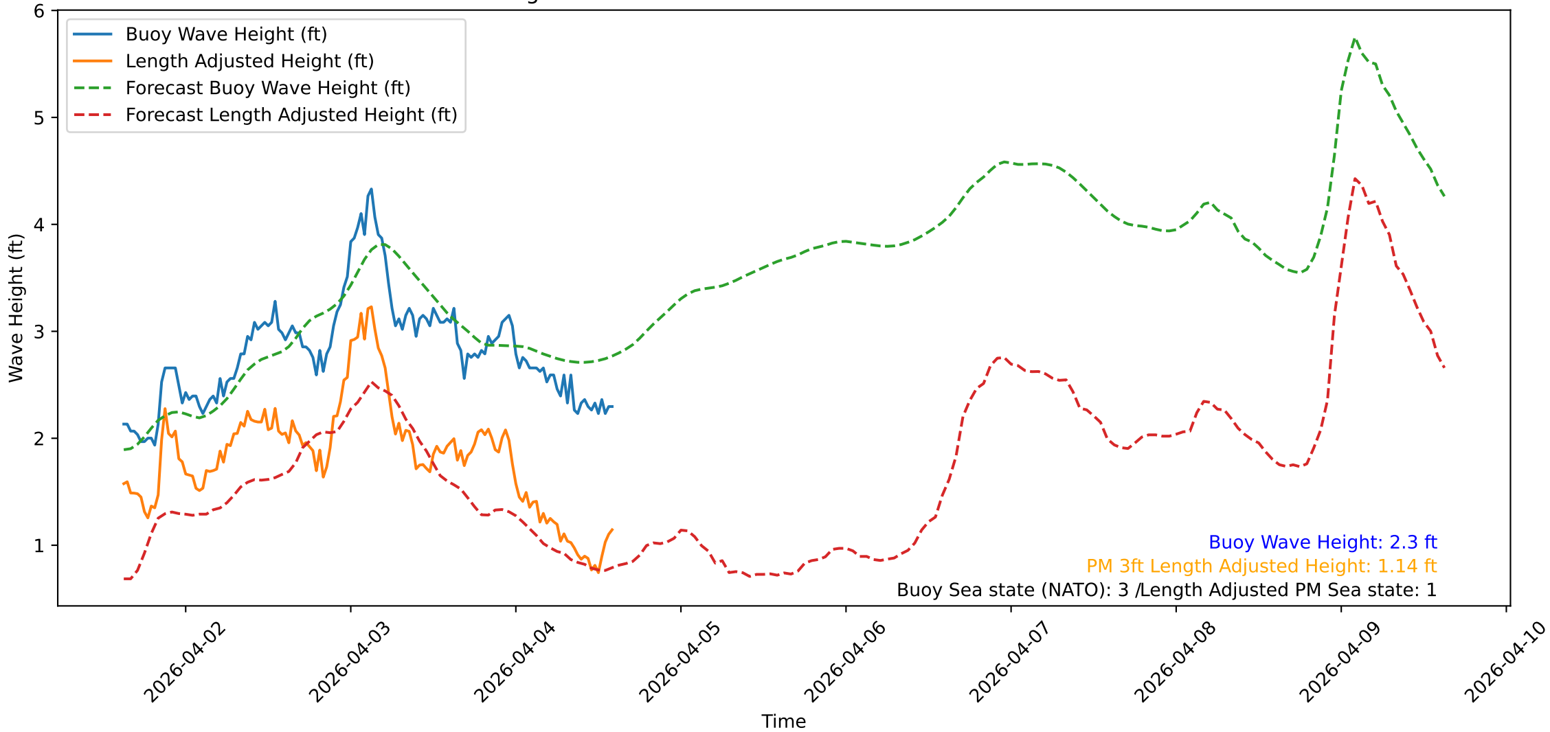
Wave Heights over Time for Green Beach at 2026-04-04 14:51:10
