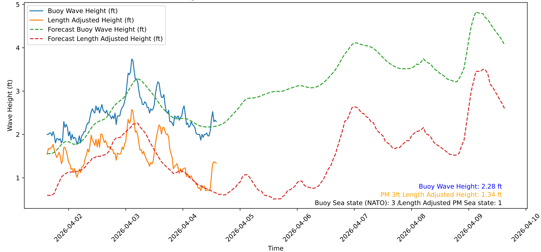
Wave Heights over Time for Red Beach at 2026-04-04 14:50:47
