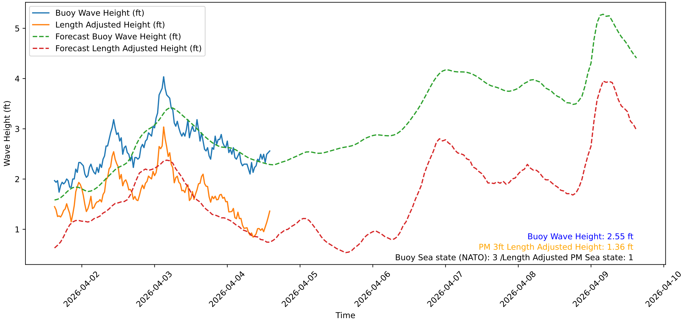
Wave Heights over Time for Oceanside Harbor at 2026-04-04 14:50:31
