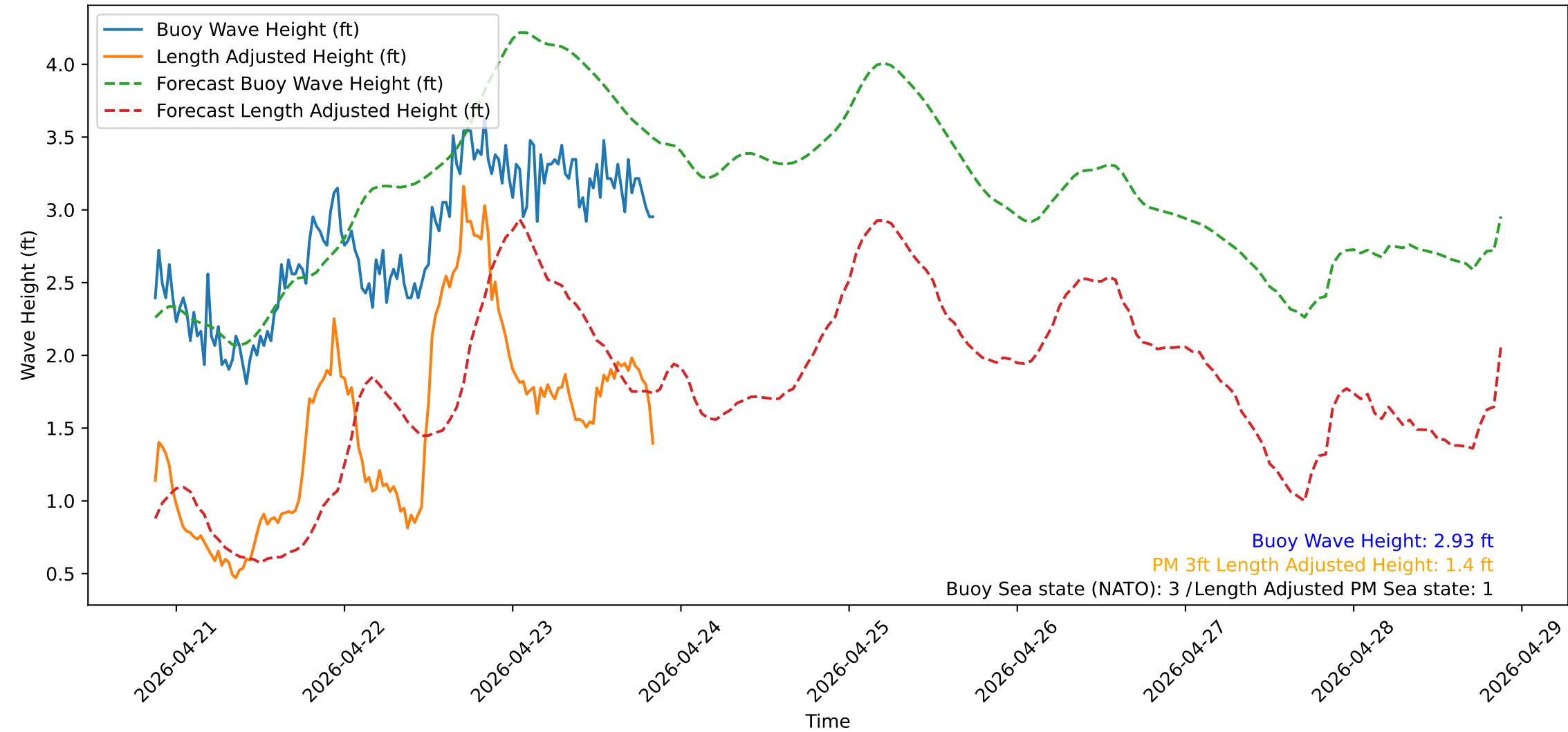
Wave Heights over Time for Red Beach at 2026-04-23 20:40:50
