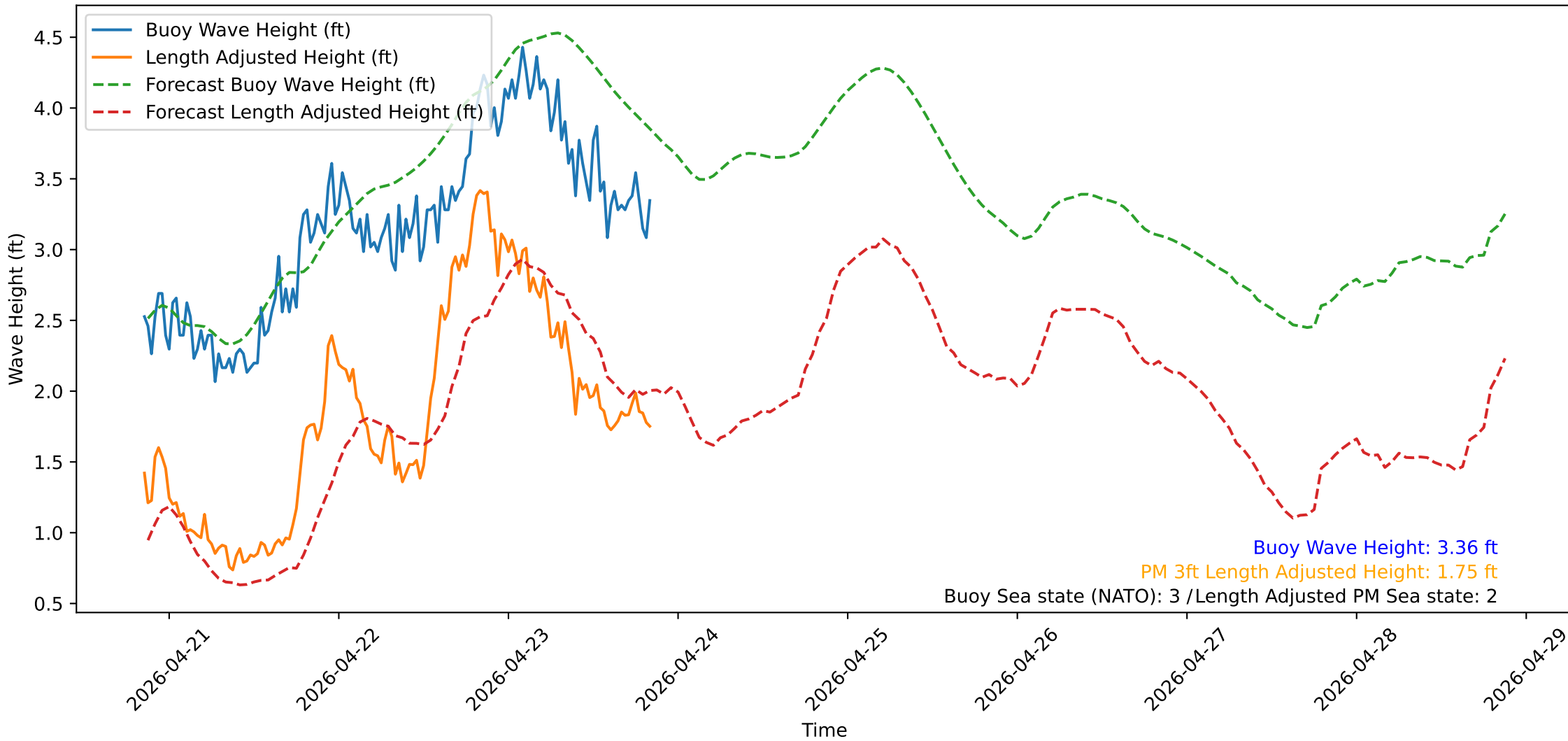
Wave Heights over Time for Oceanside Harbor at 2026-04-23 20:40:31
