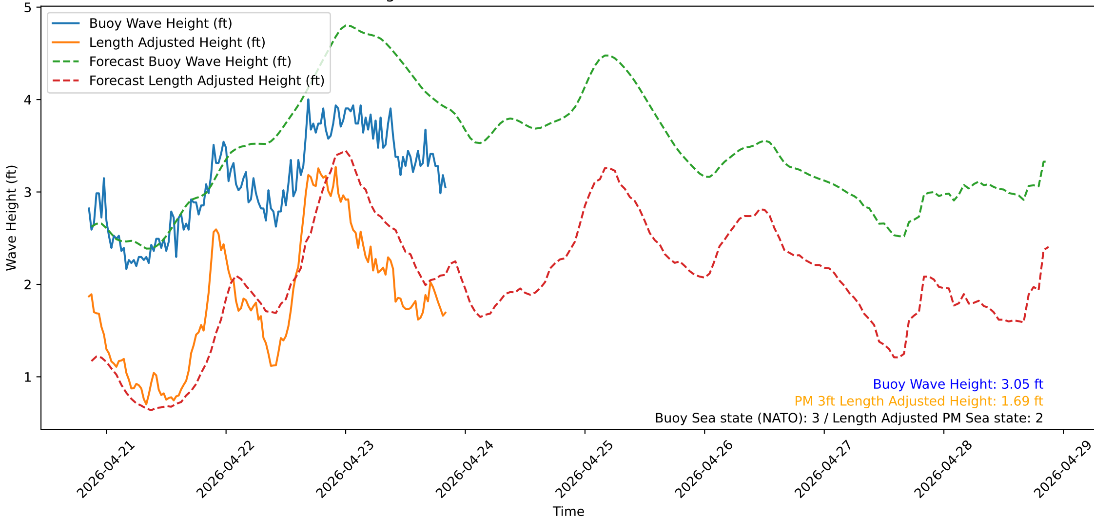
Wave Heights over Time for Green Beach at 2026-04-23 20:41:13
