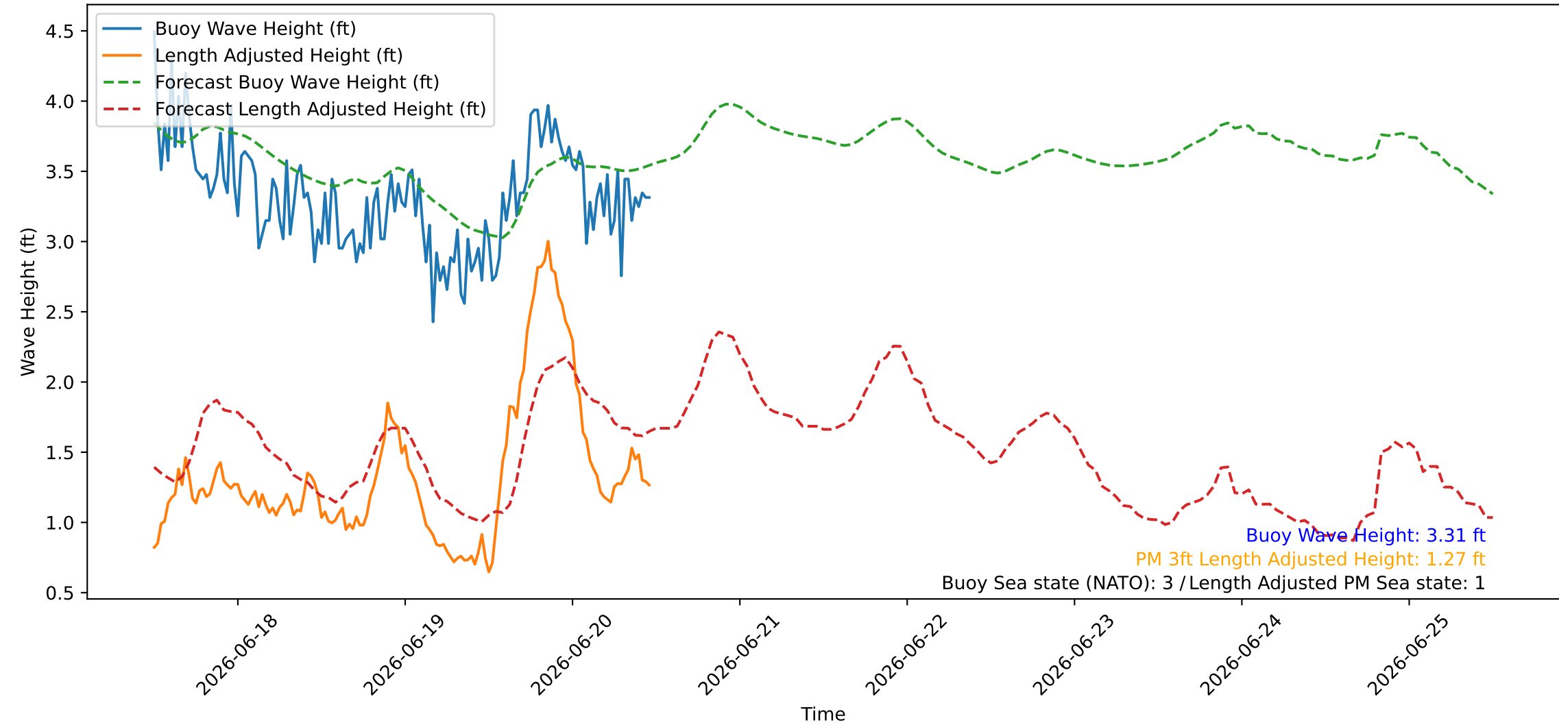
Wave Heights over Time for Green Beach at 2026-06-20 11:51:10
