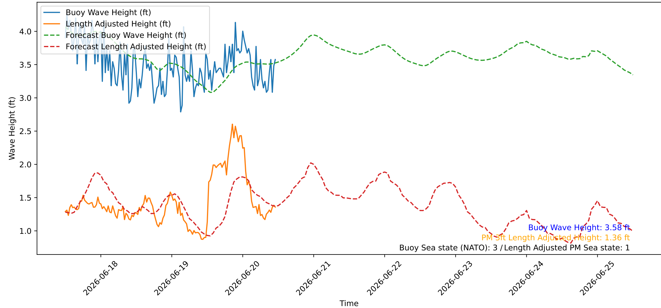
Wave Heights over Time for Oceanside Harbor at 2026-06-20 11:50:26
