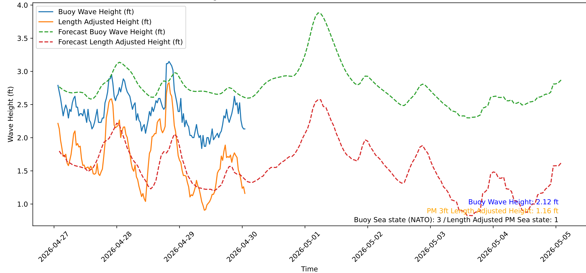
Wave Heights over Time for Green Beach at 2026-04-30 01:41:13
