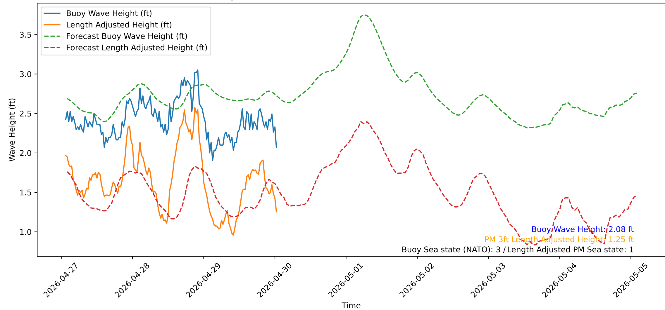
Wave Heights over Time for Oceanside Harbor at 2026-04-30 01:40:32
