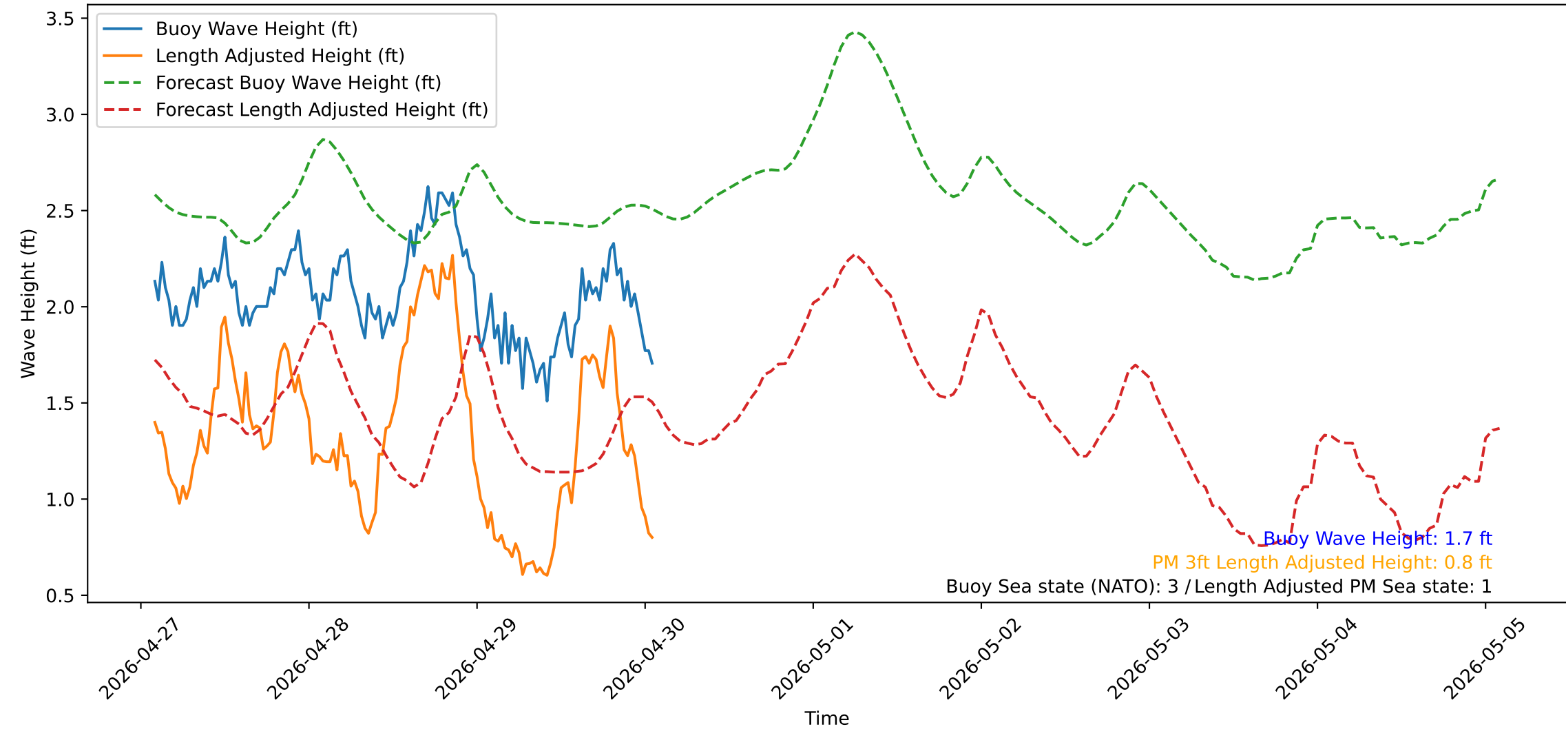
Wave Heights over Time for Red Beach at 2026-04-30 01:40:51
