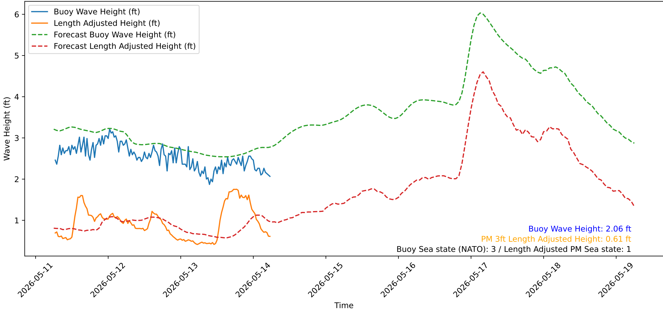
Wave Heights over Time for Red Beach at 2026-05-14 06:10:51
