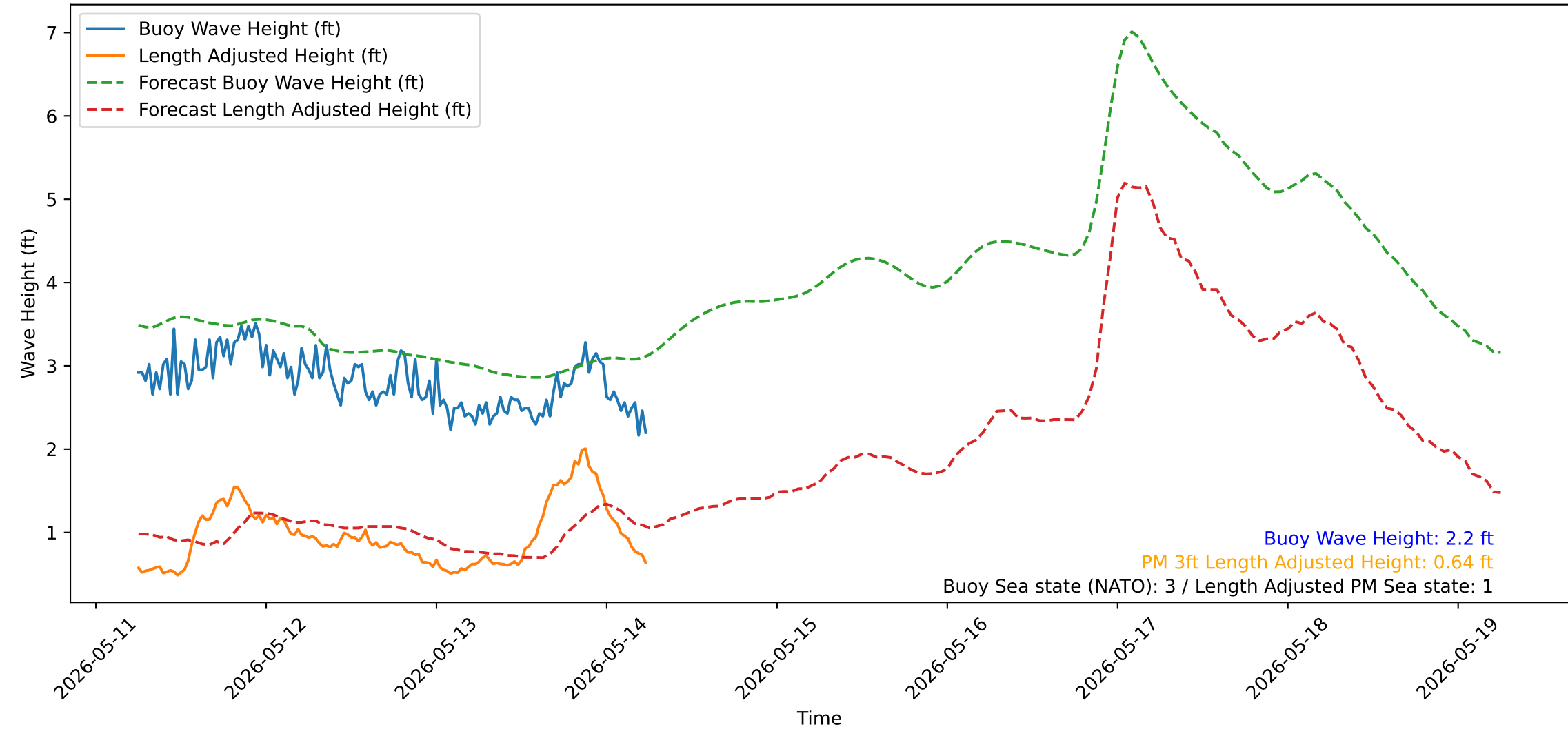
Wave Heights over Time for Green Beach at 2026-05-14 06:11:13
