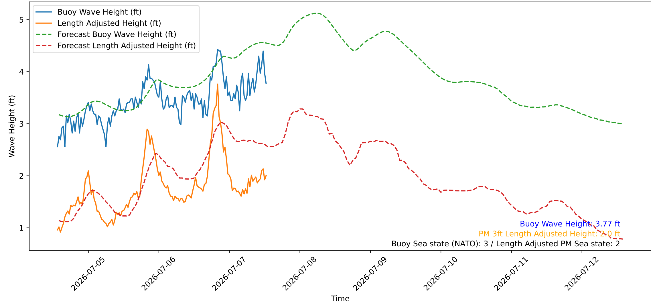
Wave Heights over Time for Green Beach at 2026-07-07 13:31:08
