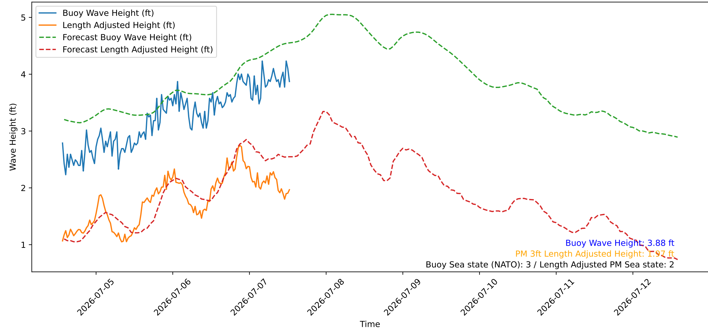
Wave Heights over Time for Oceanside Harbor at 2026-07-07 13:30:25
