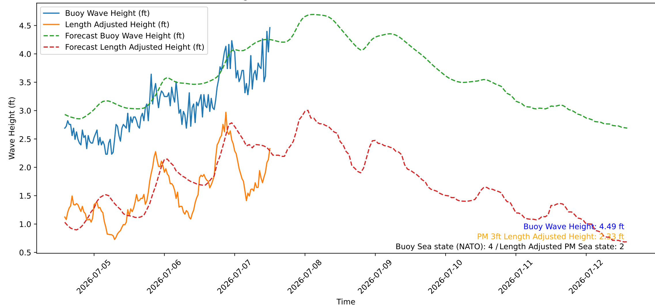
Wave Heights over Time for Red Beach at 2026-07-07 13:30:44
