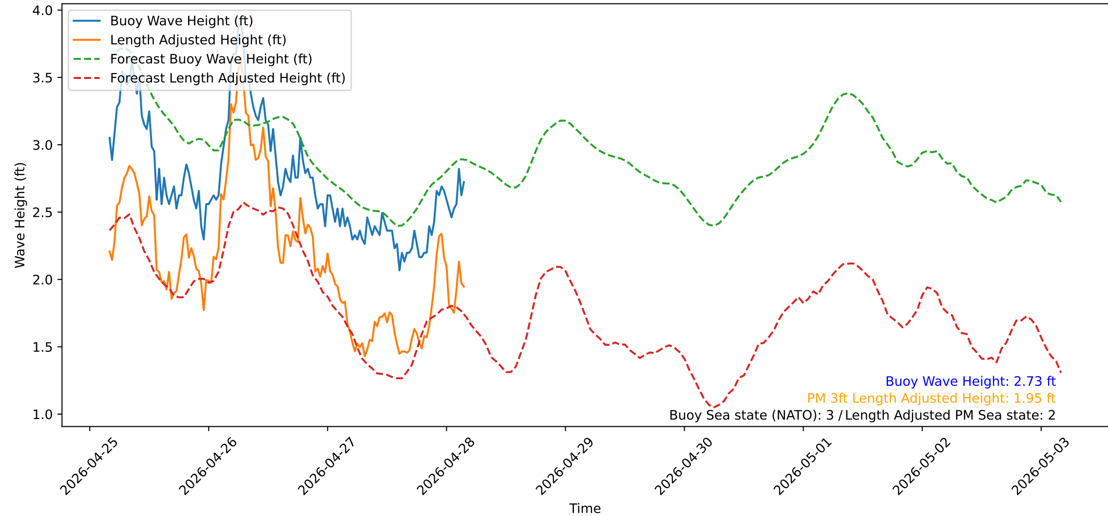
Wave Heights over Time for Oceanside Harbor at 2026-04-28 04:00:31
