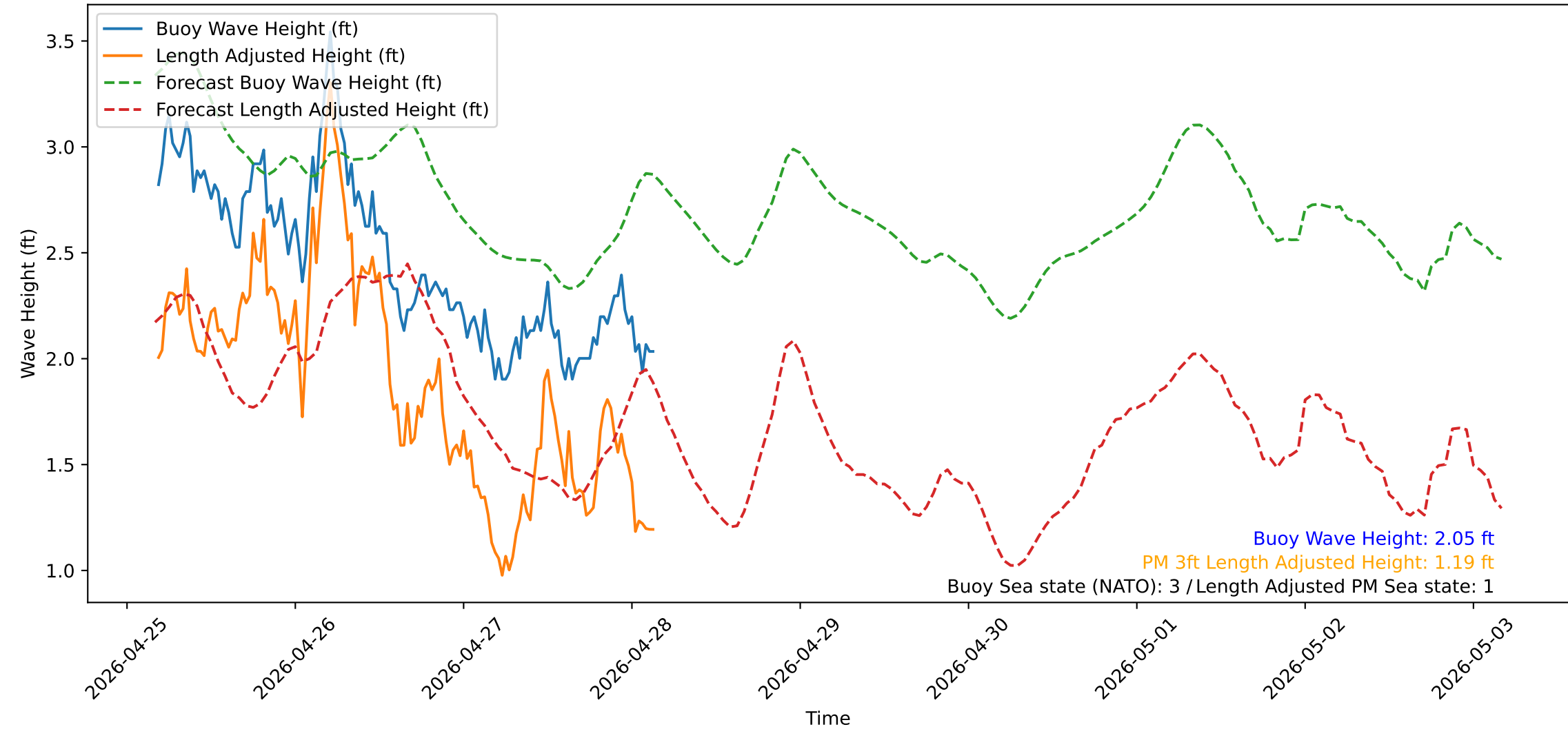
Wave Heights over Time for Red Beach at 2026-04-28 04:00:50
