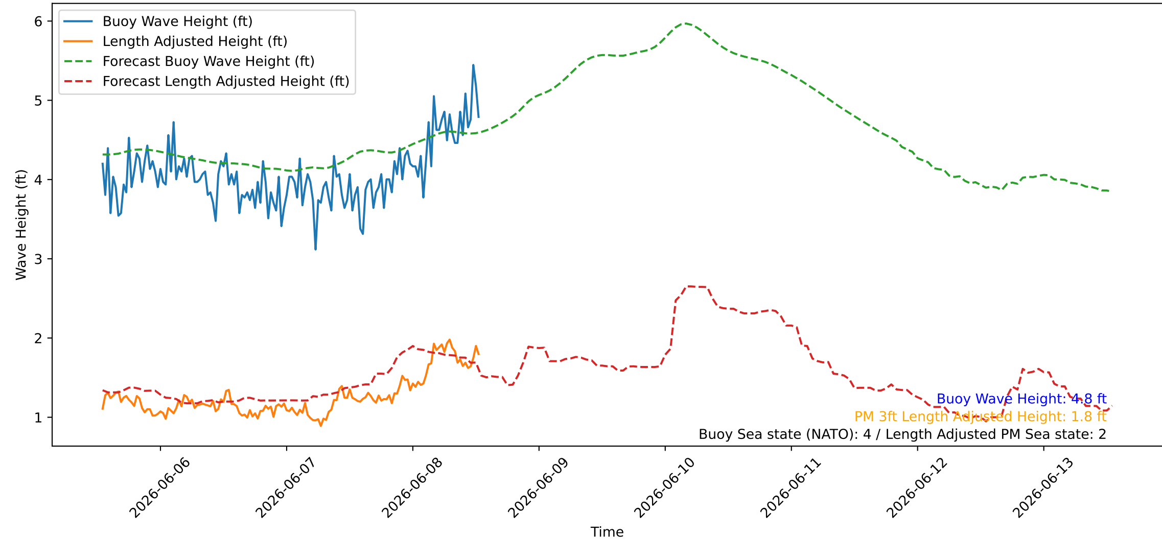
Wave Heights over Time for Green Beach at 2026-06-08 13:11:08
