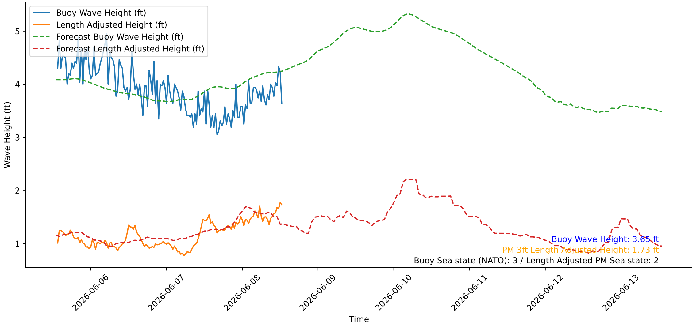
Wave Heights over Time for Red Beach at 2026-06-08 13:10:45
