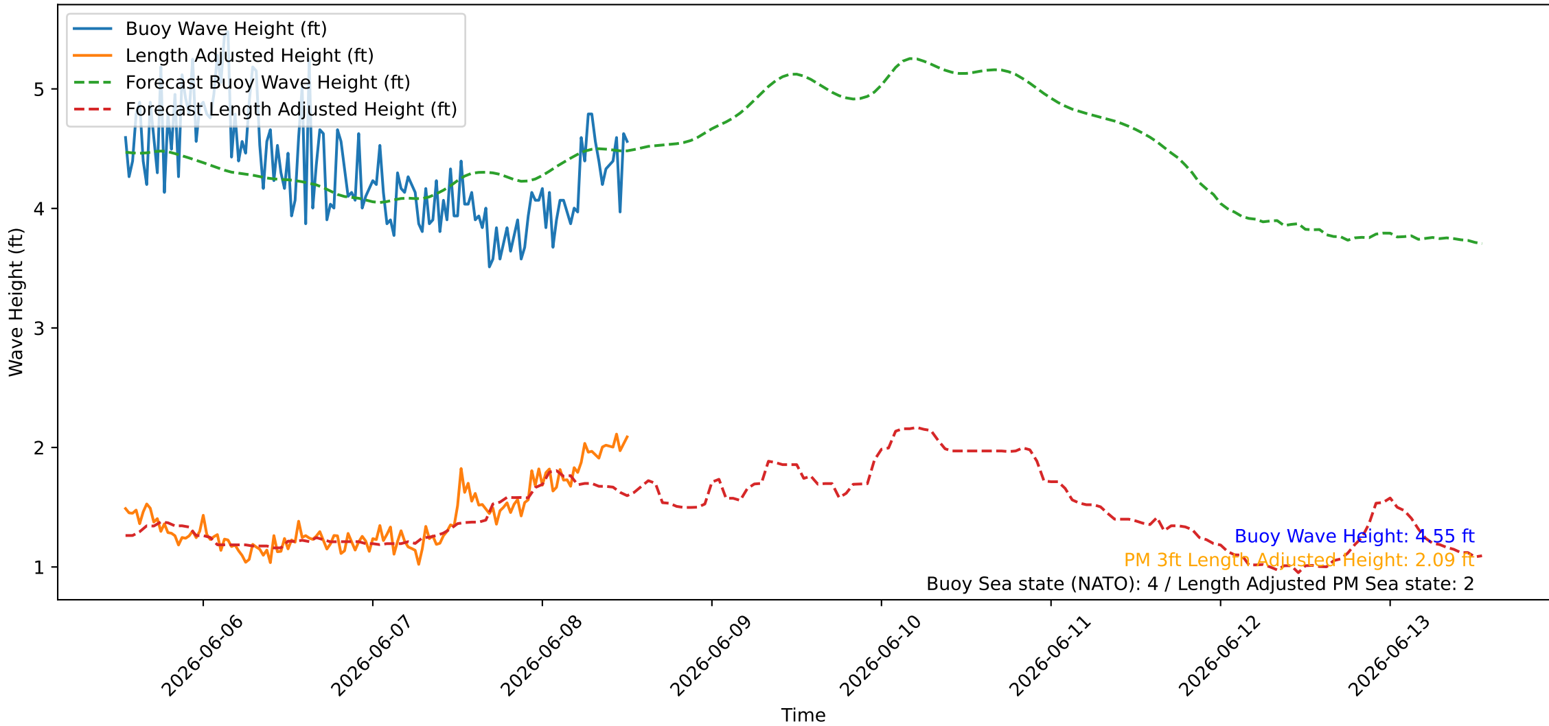
Wave Heights over Time for Oceanside Harbor at 2026-06-08 13:10:26
