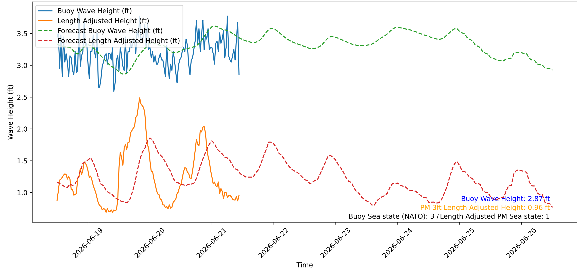
Wave Heights over Time for Red Beach at 2026-06-21 11:30:45
