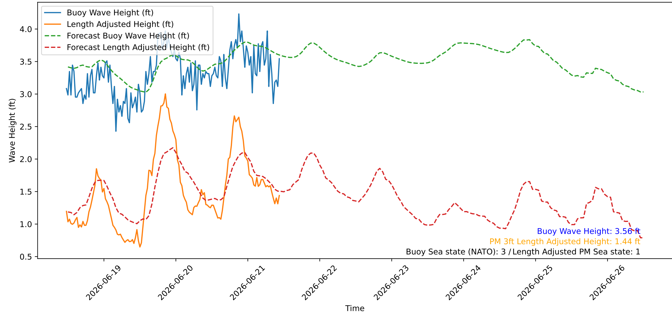
Wave Heights over Time for Green Beach at 2026-06-21 11:31:08
