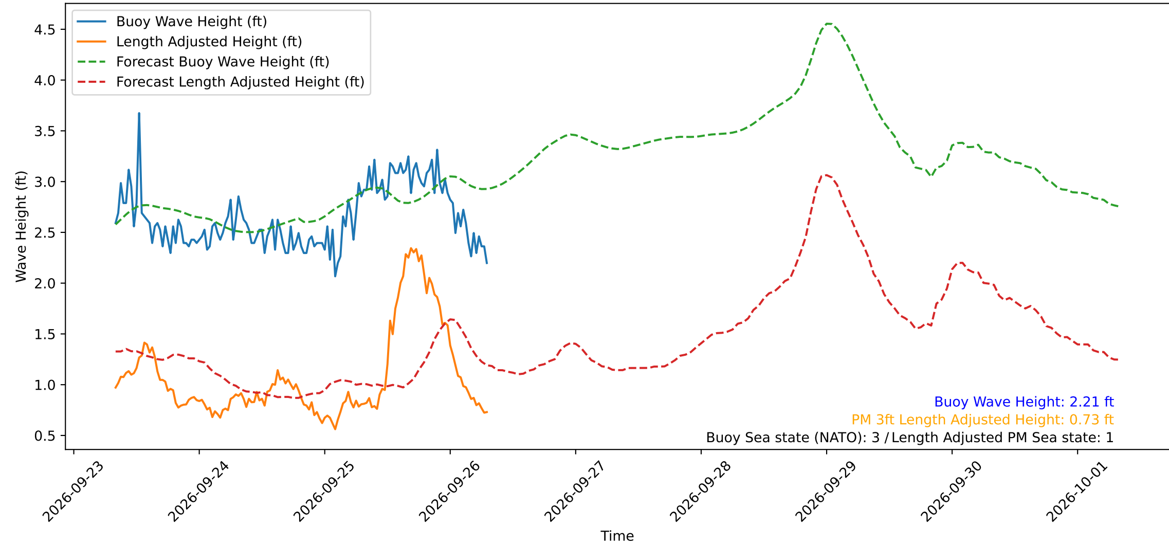
Wave Heights over Time for Red Beach at 2026-09-26 07:50:51
