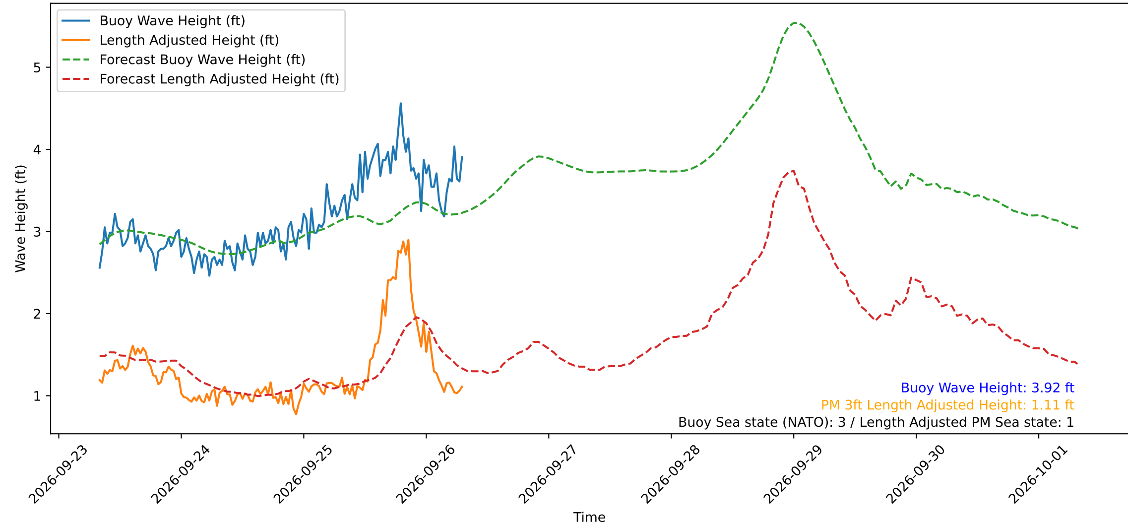
Wave Heights over Time for Green Beach at 2026-09-26 07:51:14
