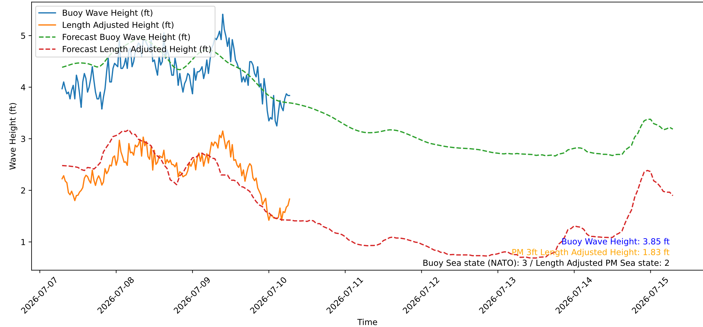
Wave Heights over Time for Oceanside Harbor at 2026-07-10 07:10:26
