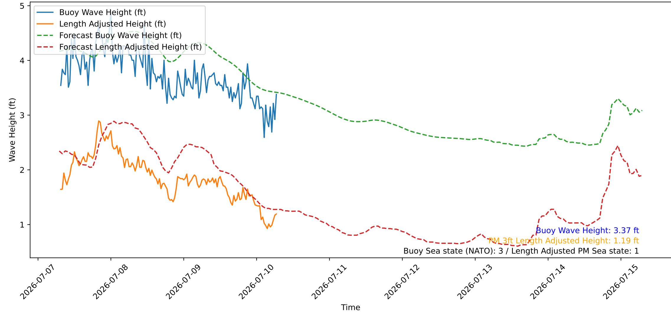
Wave Heights over Time for Red Beach at 2026-07-10 07:10:45
