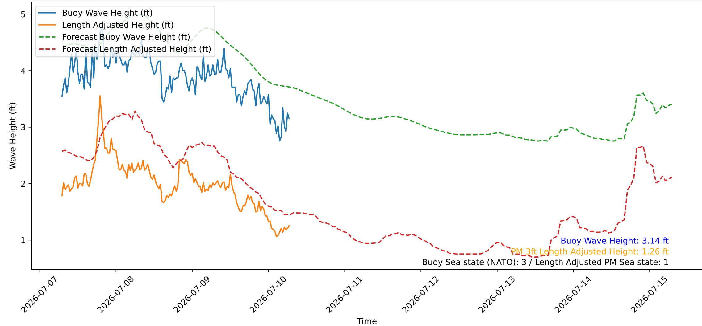
Wave Heights over Time for Green Beach at 2026-07-10 07:11:08
