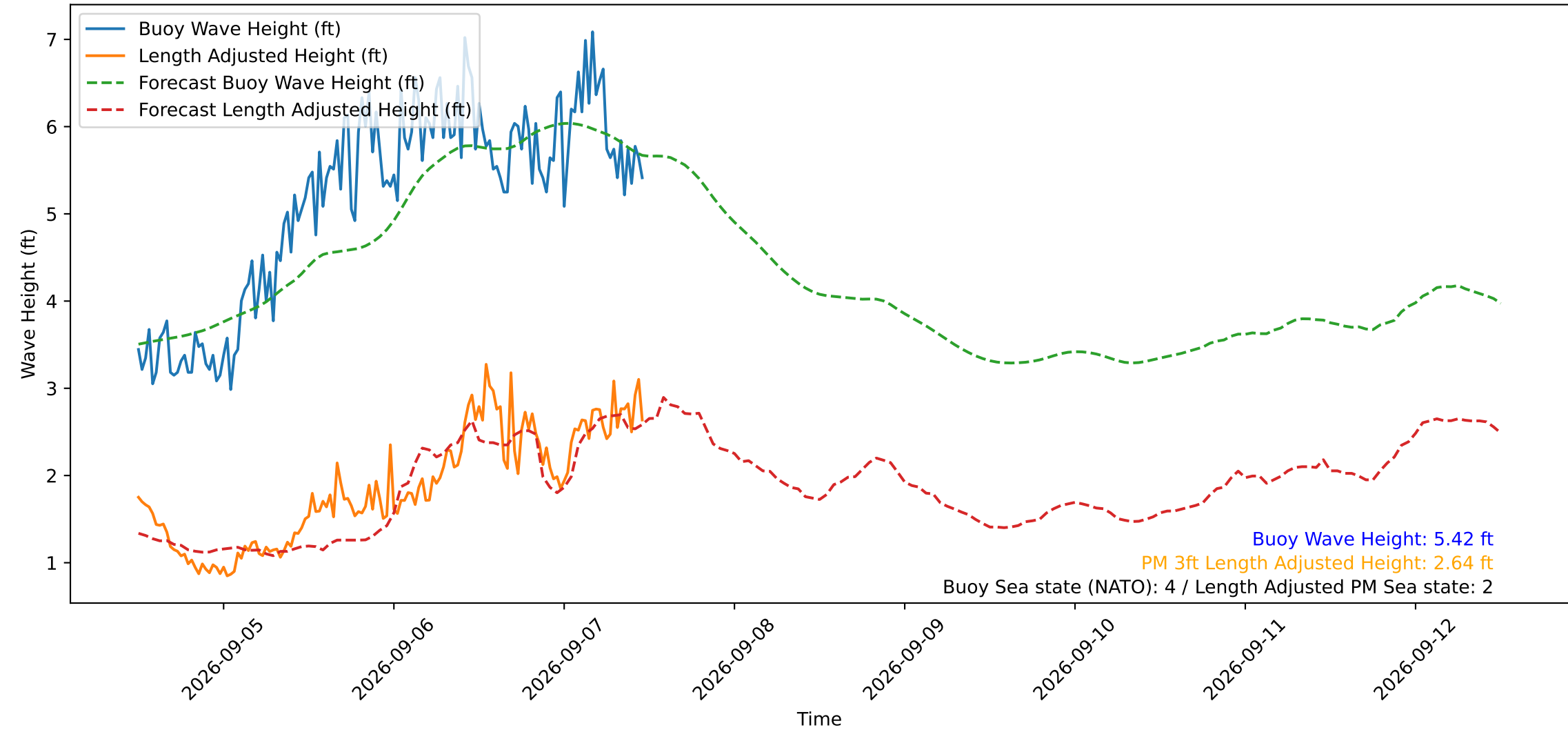
Wave Heights over Time for Oceanside Harbor at 2026-09-07 11:50:30
