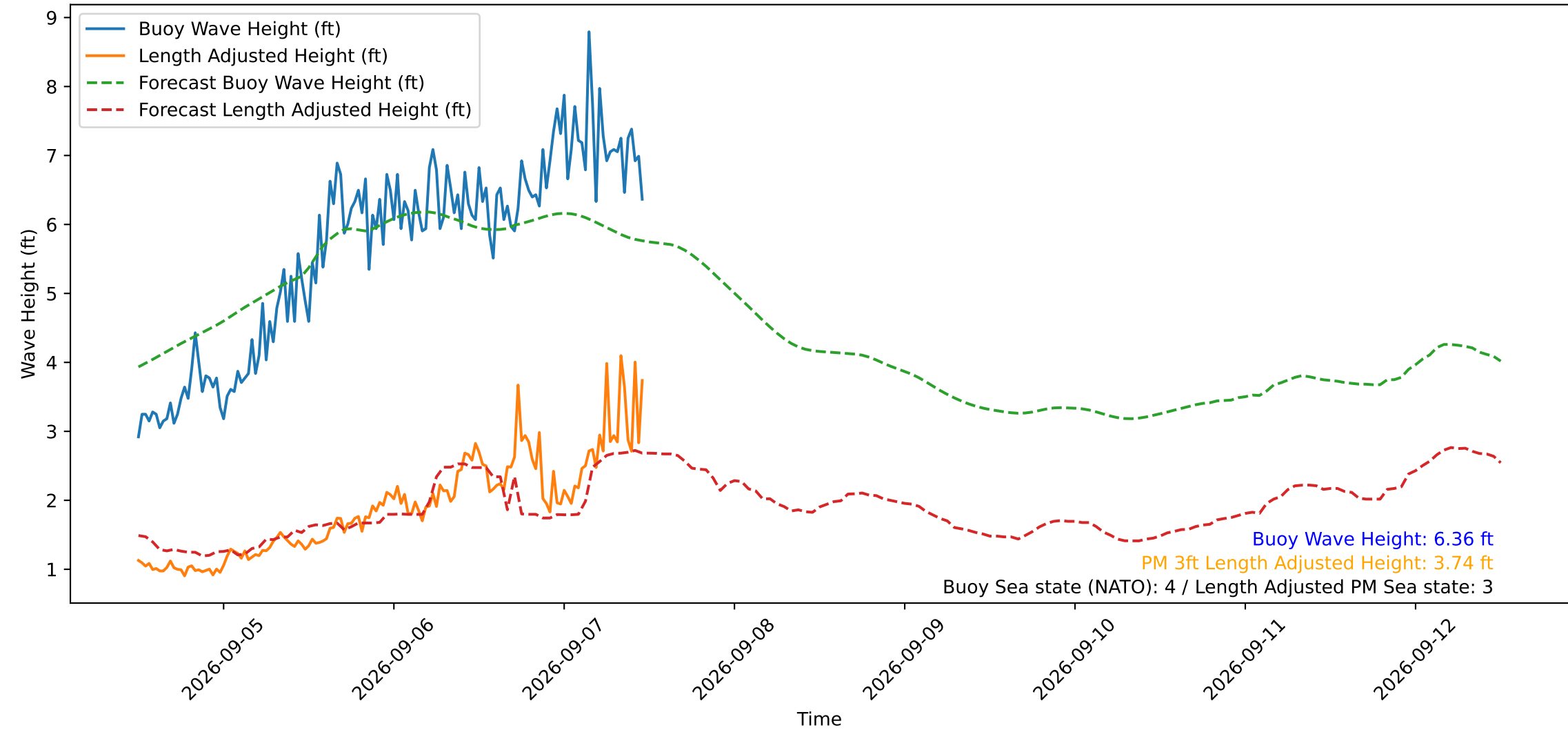
Wave Heights over Time for Green Beach at 2026-09-07 11:51:15
