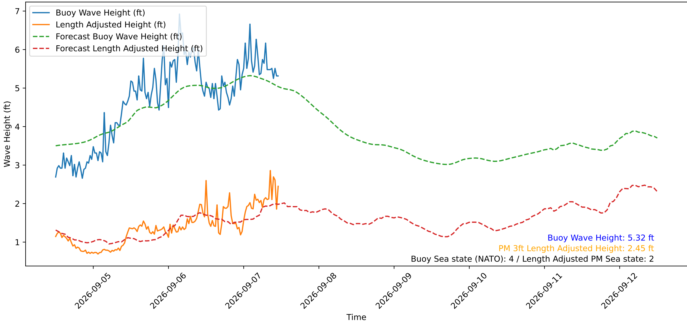
Wave Heights over Time for Red Beach at 2026-09-07 11:50:51
