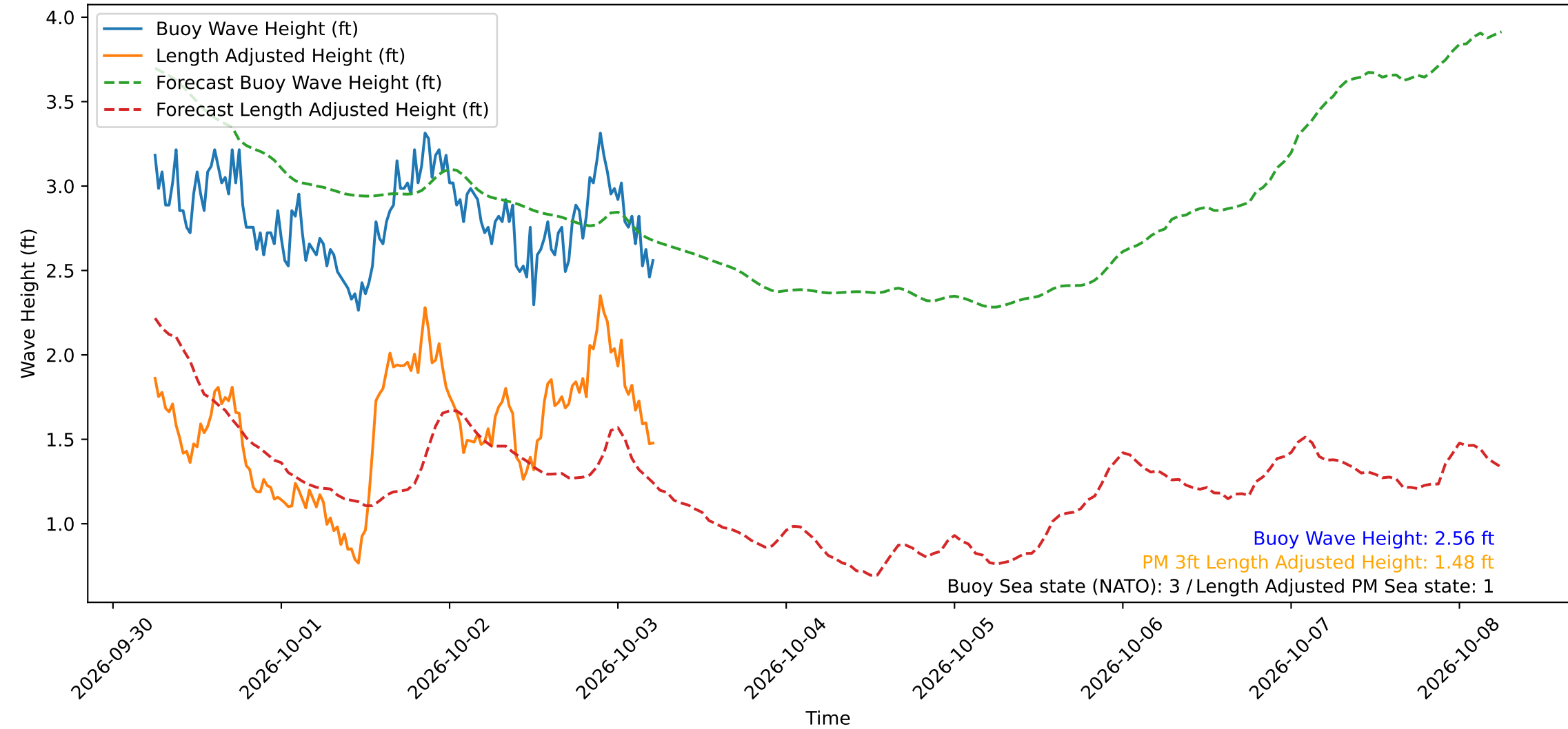
Wave Heights over Time for Oceanside Harbor at 2026-10-03 06:00:29
