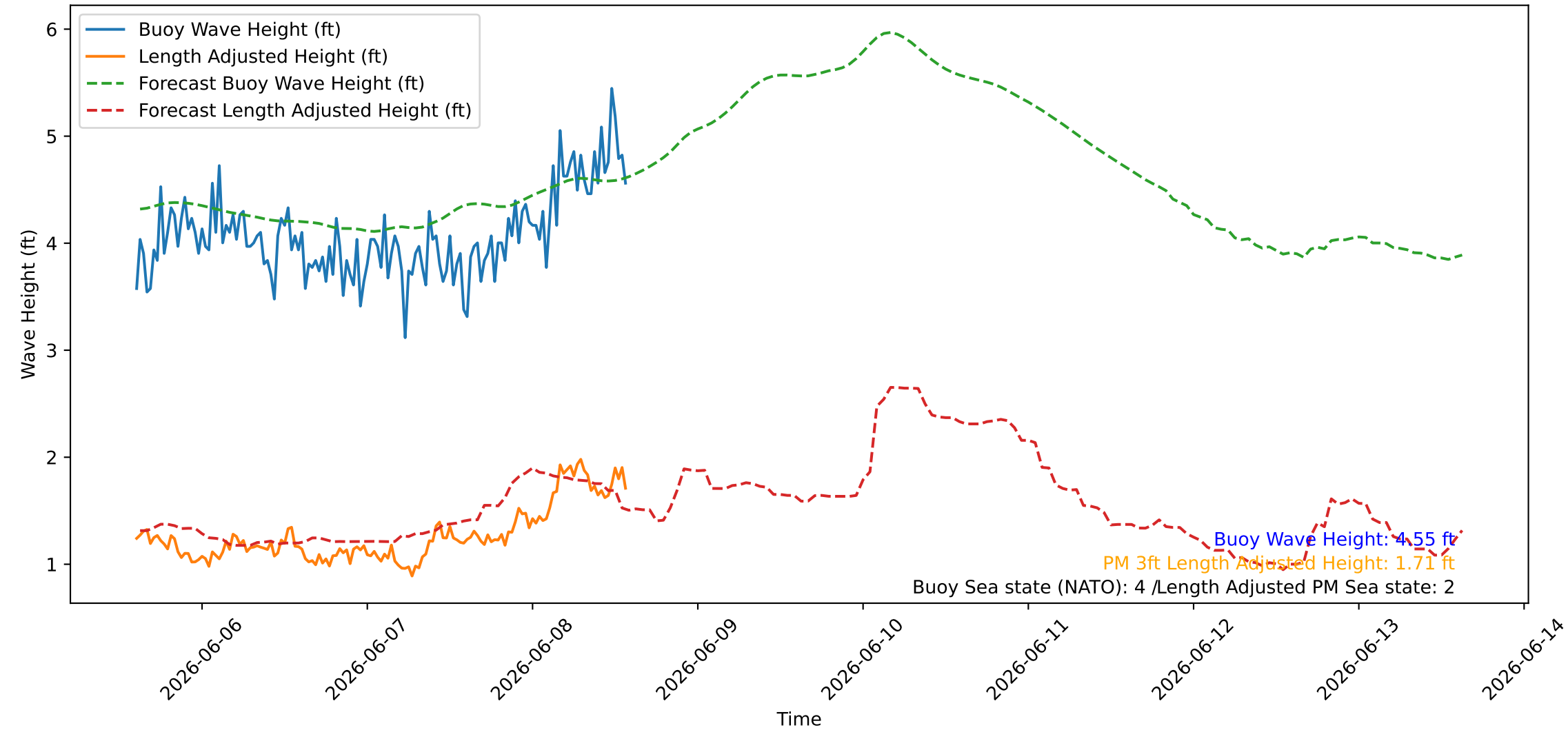
Wave Heights over Time for Green Beach at 2026-06-08 14:31:09
