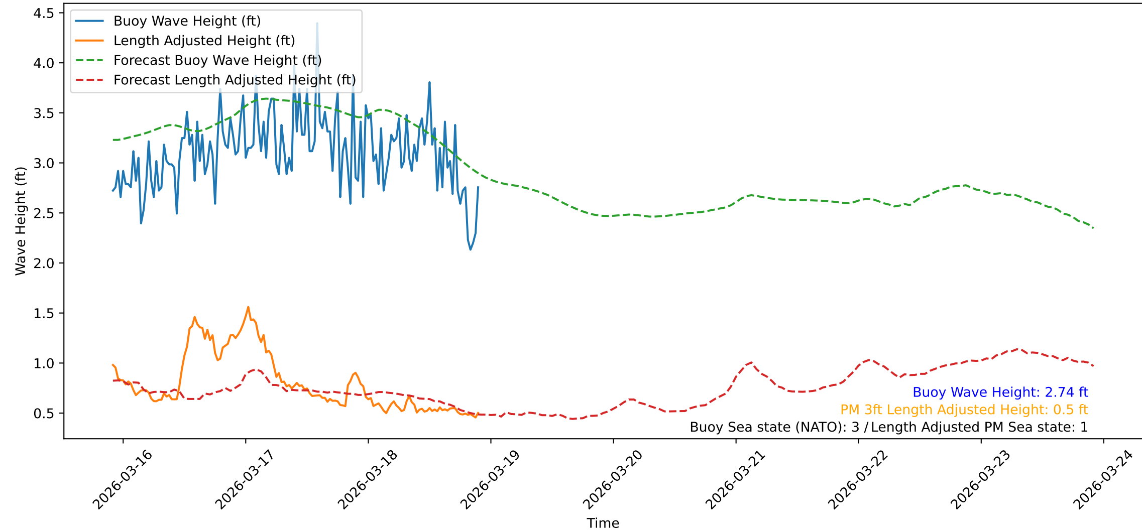
Wave Heights over Time for Oceanside Harbor at 2026-03-18 22:00:32
