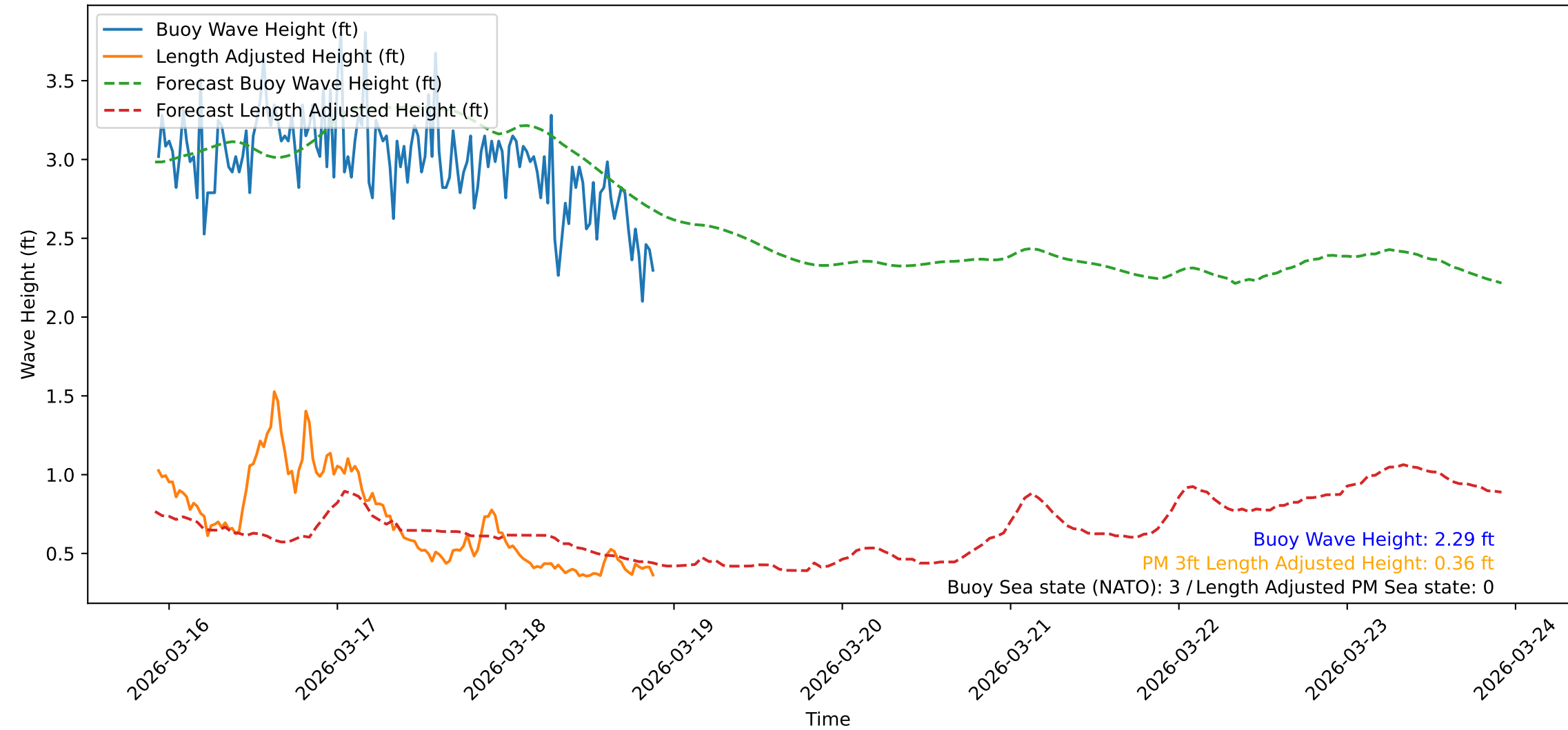
Wave Heights over Time for Red Beach at 2026-03-18 22:00:49
