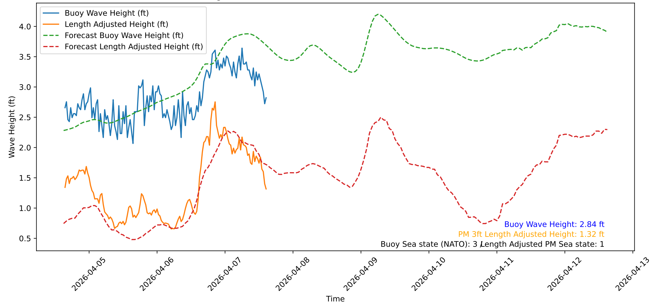
Wave Heights over Time for Oceanside Harbor at 2026-04-07 15:20:31
