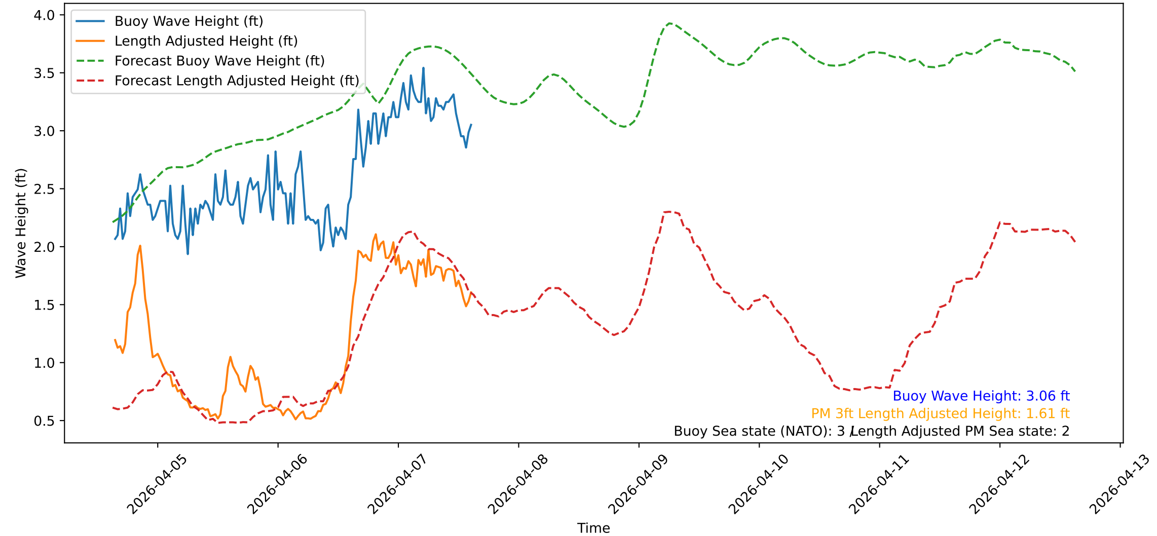
Wave Heights over Time for Red Beach at 2026-04-07 15:20:47
