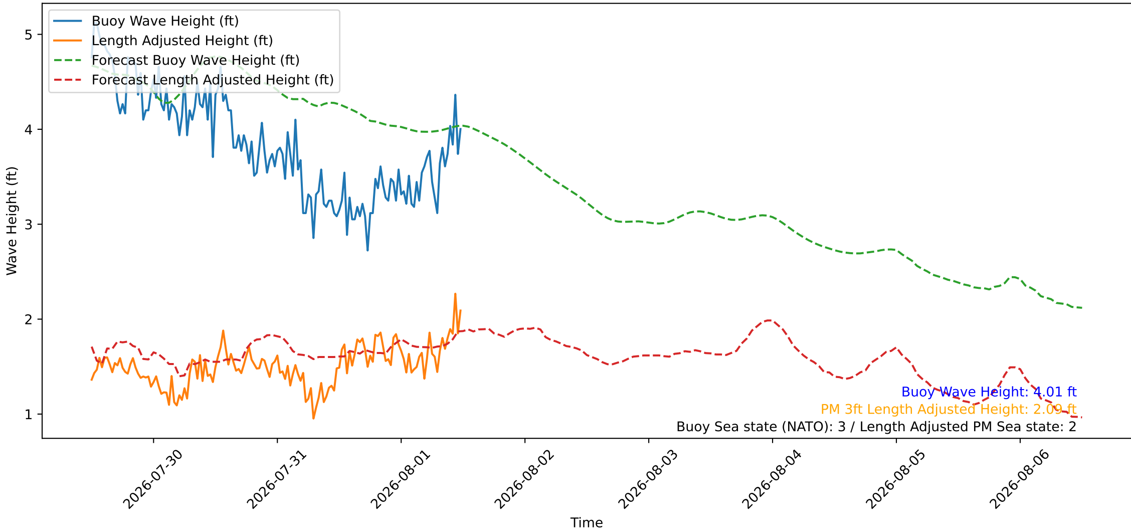
Wave Heights over Time for Oceanside Harbor at 2026-08-01 12:10:26
