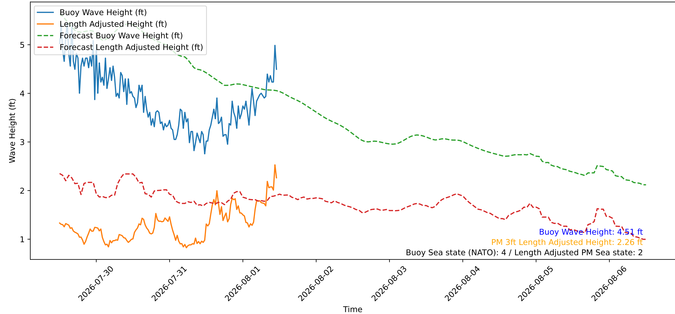
Wave Heights over Time for Green Beach at 2026-08-01 12:11:08
