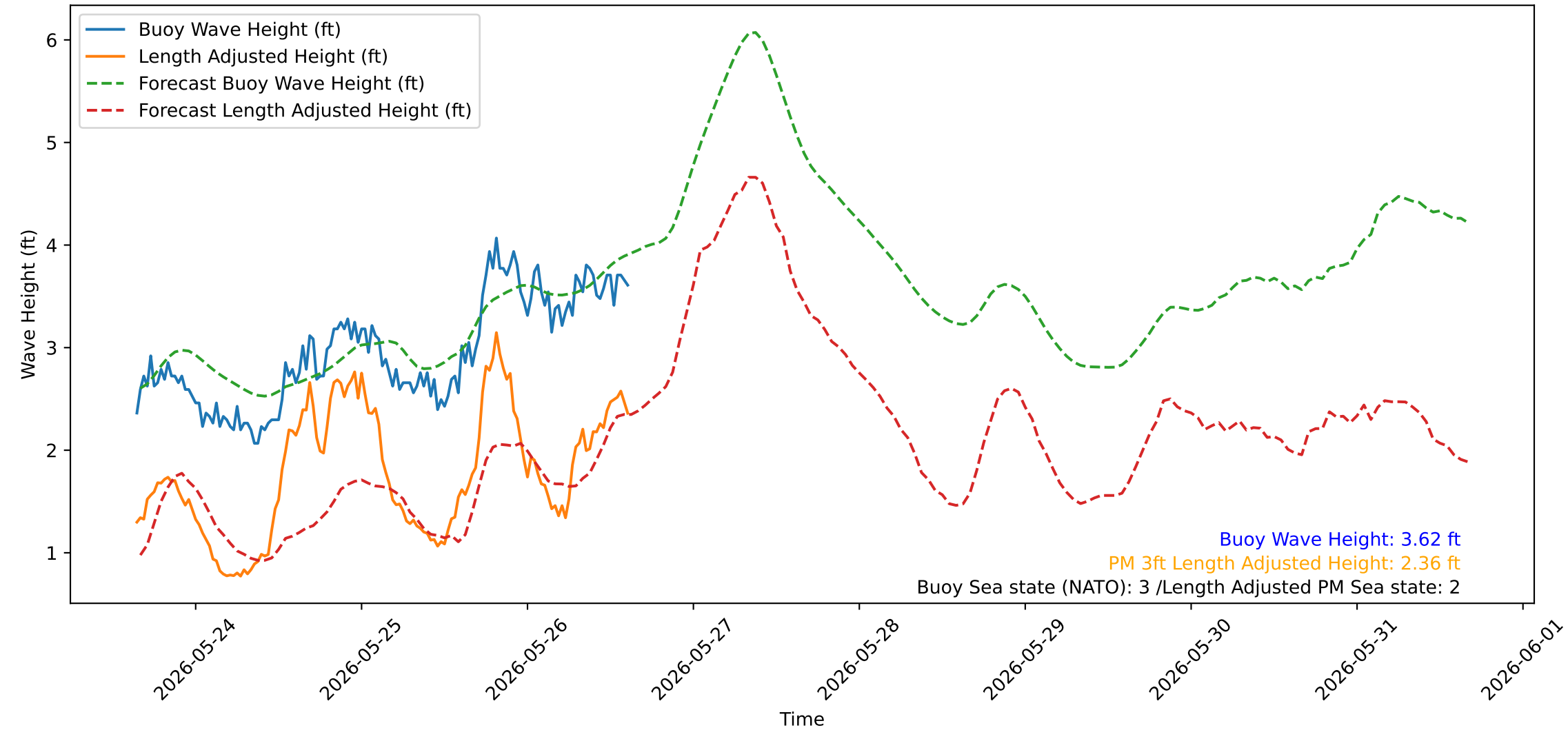
Wave Heights over Time for Green Beach at 2026-05-26 15:31:09
