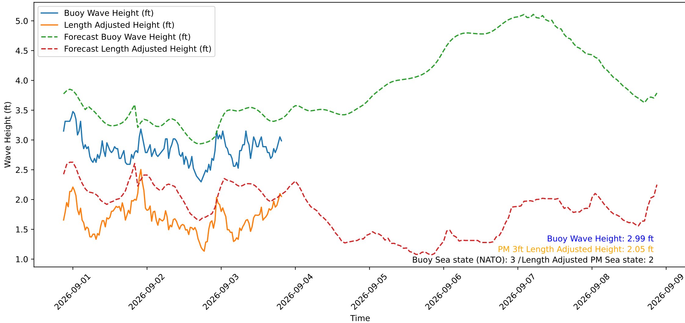
Wave Heights over Time for Red Beach at 2026-09-03 20:30:49
