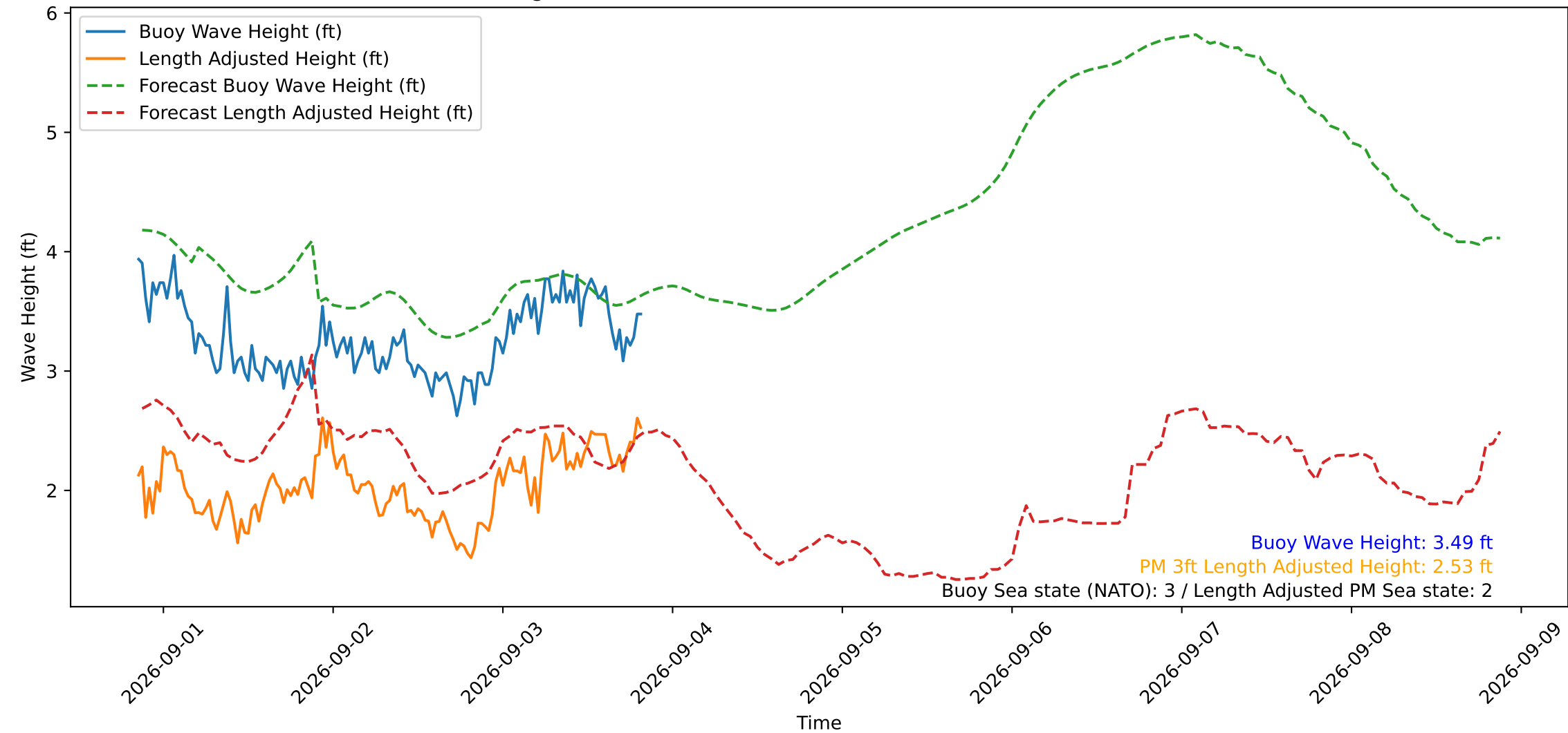
Wave Heights over Time for Oceanside Harbor at 2026-09-03 20:30:29
